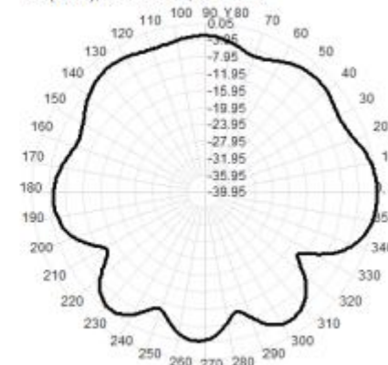
Total(H-XY), Max= 0.05dBi, CirD=13.78
