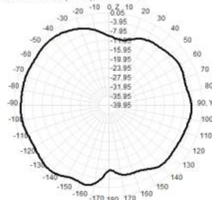
2450.0MHz Total(E2-YZ), Max= -2.51dBi
