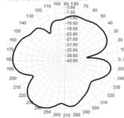
Total(H-XY), Max= -4.50dBi, CirD=22.59
