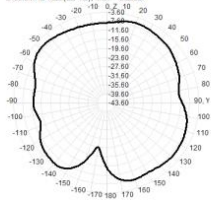
2400.0MHz Total(E2-YZ), Max= -6.22dBi
