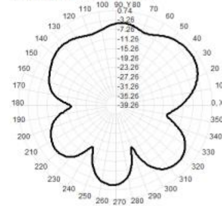
Total(H-XY), Max= -1.32dBi, CirD= 19.81
