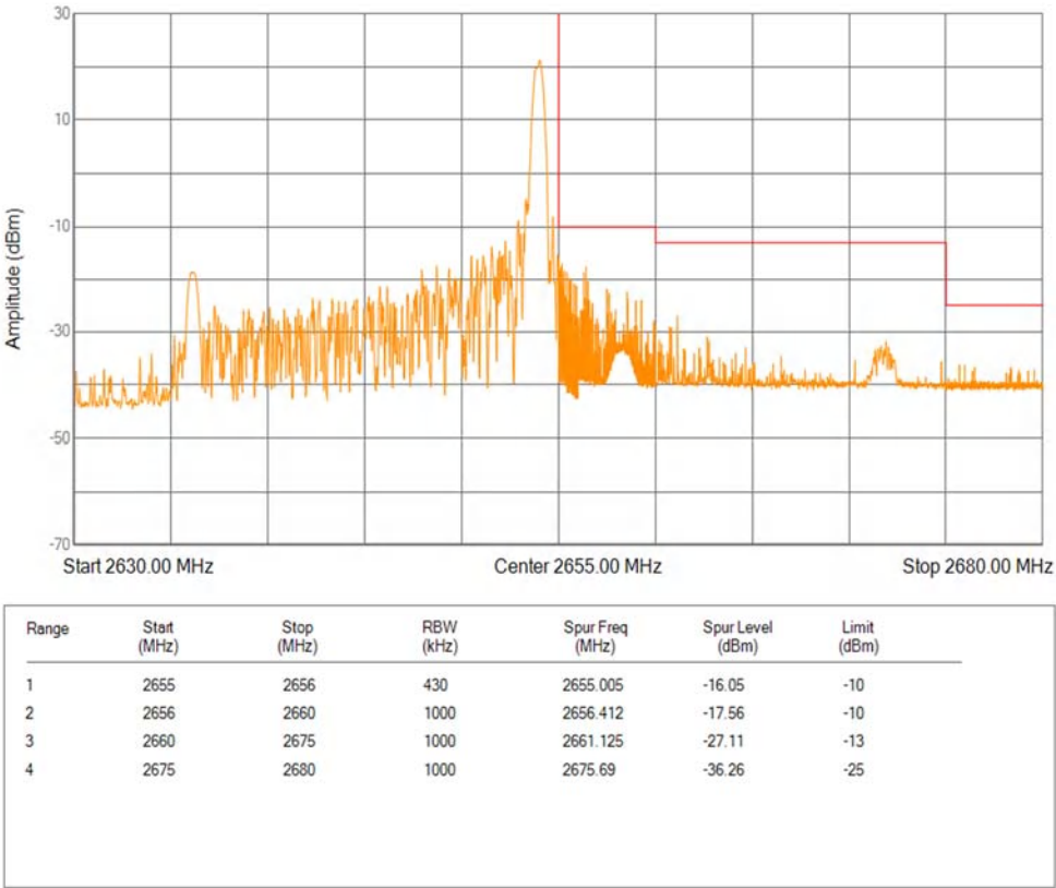
Band41(2535-2655) 16QAM BW=20MHz Channel=41140 RB Size=1 Position=#Max Extended
