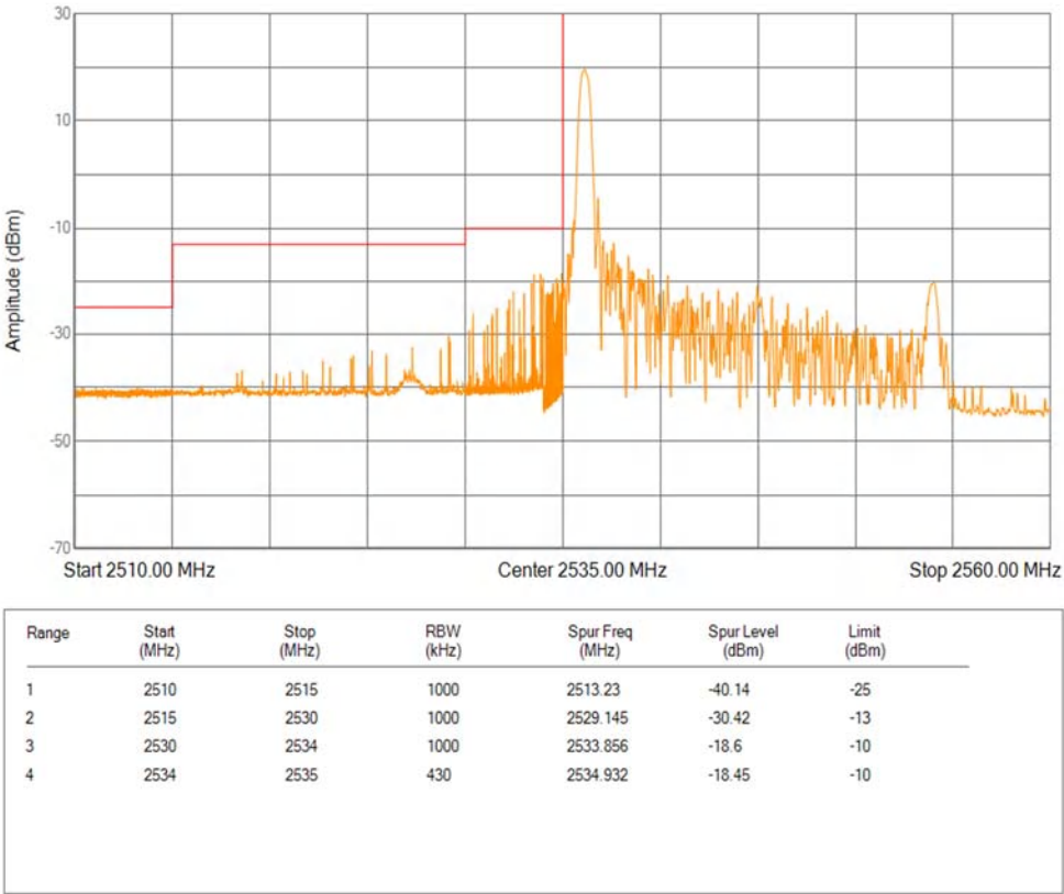
Band41(2535-2655) QPSK BW=20MHz Channel=40140 RB Size=1 Position=#0 Extended
