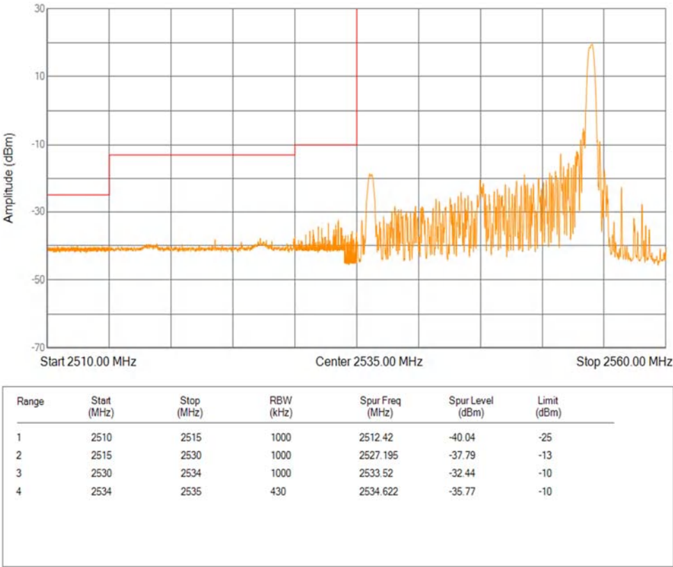
Band41(2535-2655) 16QAM BW=20MHz Channel=40140 RB Size=1 Position=#Max Extended
