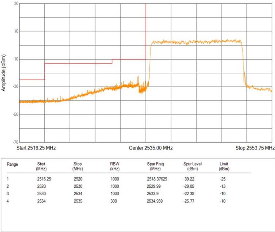
Band41(2535-2655) QPSK BW=15MHz Channel=40115 RB Size=75 Position=#0 Extended
