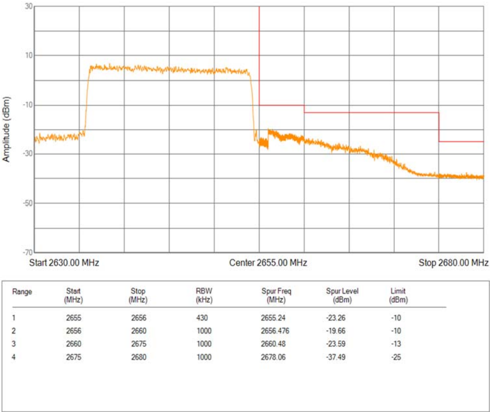
Band41(2535-2655) QPSK BW=20MHz Channel=41140 RB Size=100 Position=#0 Extended
