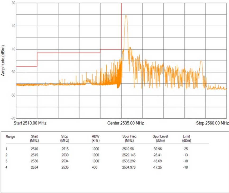
Band41(2535-2655) 16QAM BW=20MHz Channel=40140 RB Size=1 Position=#0 Extended
