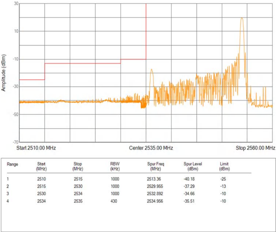
Band41(2535-2655) QPSK BW=20MHz Channel=40140 RB Size=1 Position=#Max Extended
