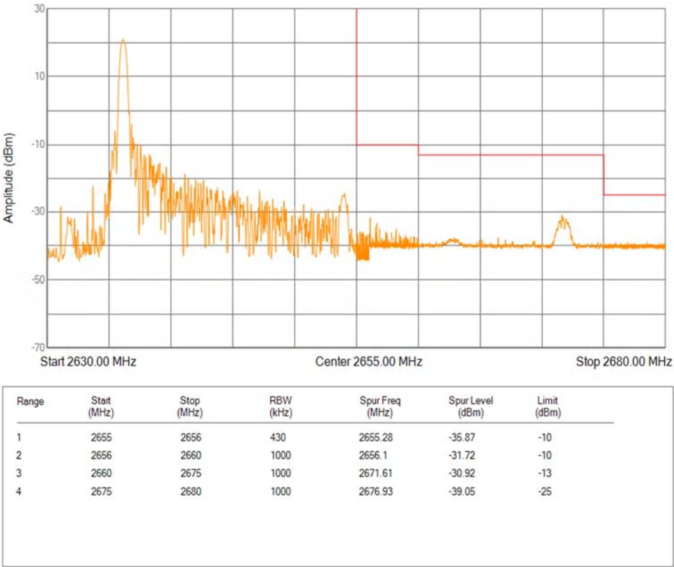
Band41(2535-2655) 16QAM BW=20MHz Channel=41140 RB Size=1 Position=#0 Extended
