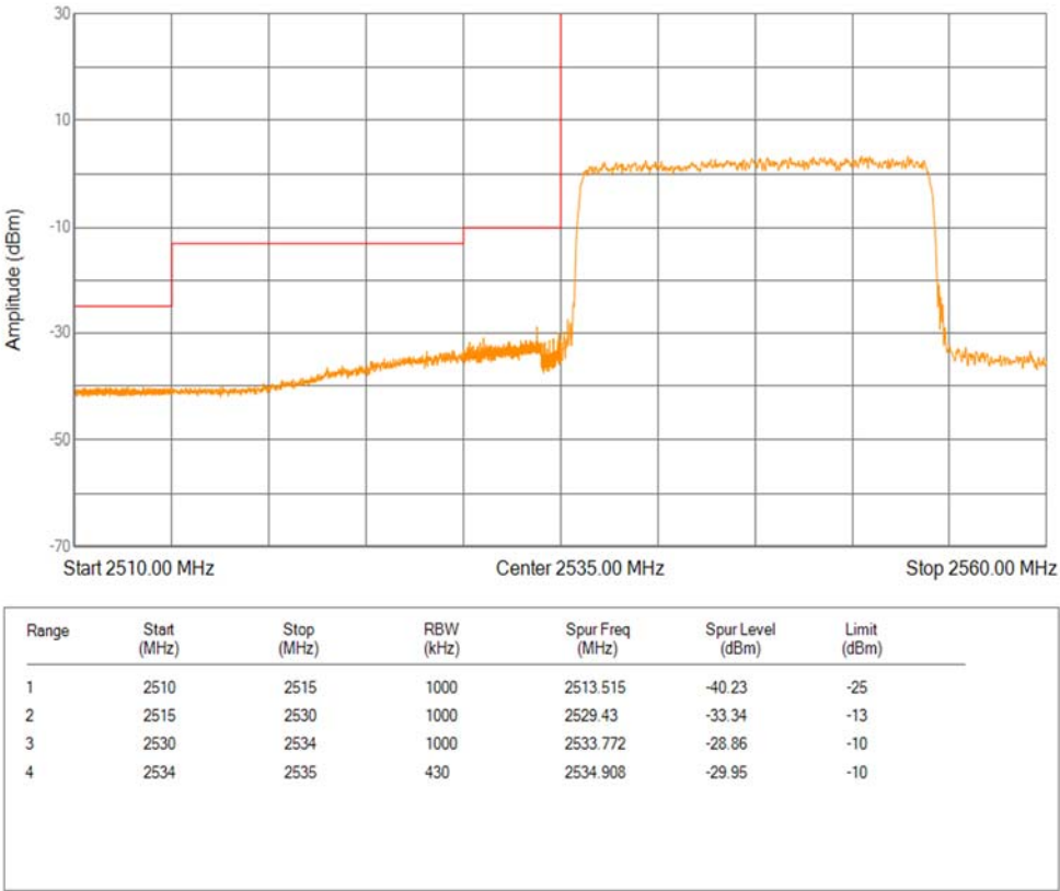
Band41(2535-2655) 16QAM BW=20MHz Channel=40140 RB Size=100 Position=#0 Extended
