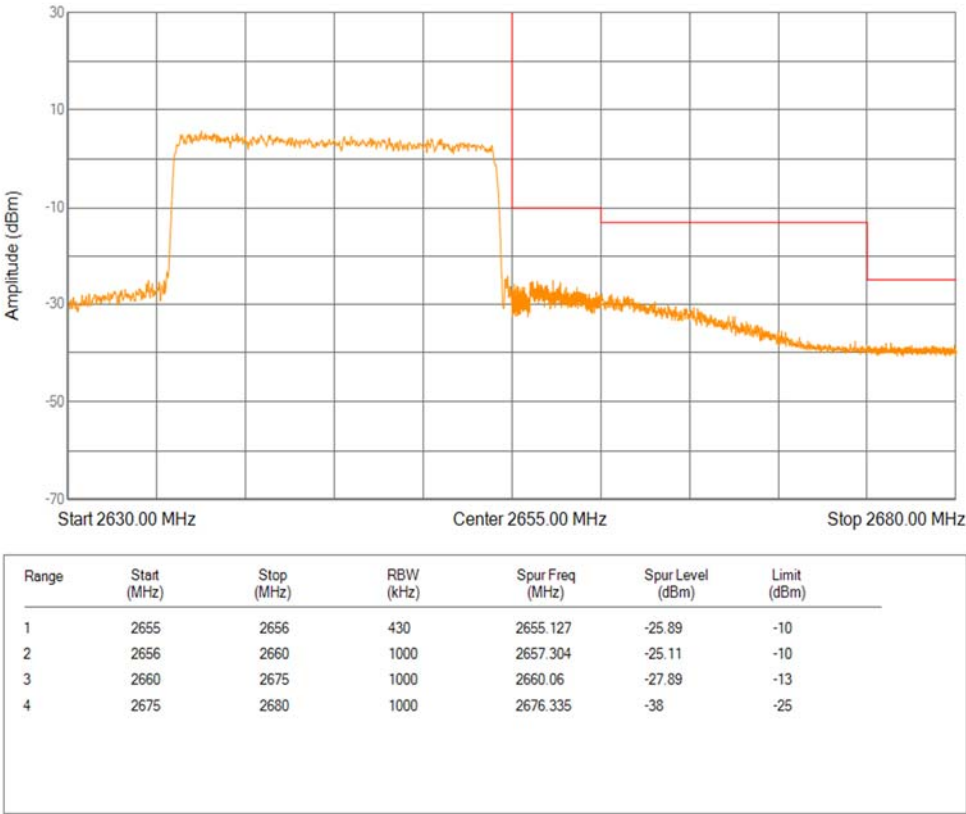
Band41(2535-2655) 16QAM BW=20MHz Channel=41140 RB Size=100 Position=#0 Extended
