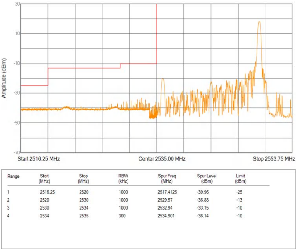
Band41(2535-2655) 16QAM BW=15MHz Channel=40115 RB Size=1 Position=#Max Extended
