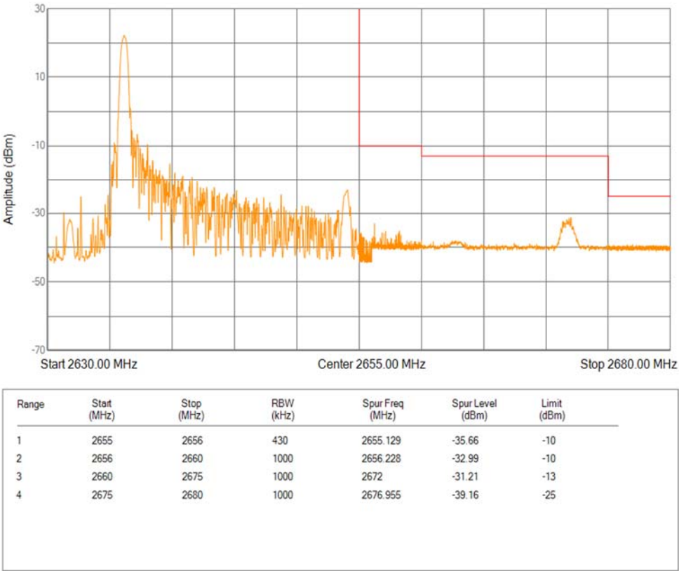
Band41(2535-2655) QPSK BW=20MHz Channel=41140 RB Size=1 Position=#0 Extended
