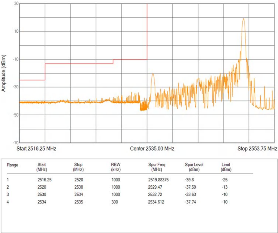
Band41(2535-2655) QPSK BW=15MHz Channel=40115 RB Size=1 Position=#Max Extended
