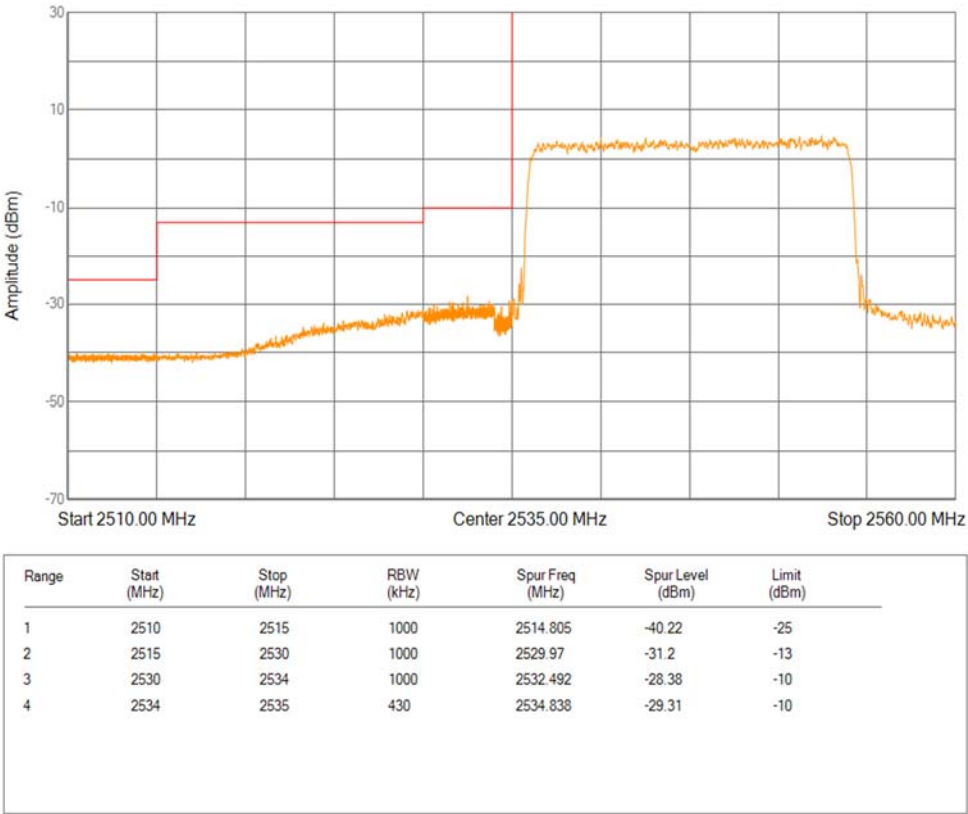
Band41(2535-2655) QPSK BW=20MHz Channel=40140 RB Size=100 Position=#0 Extended
