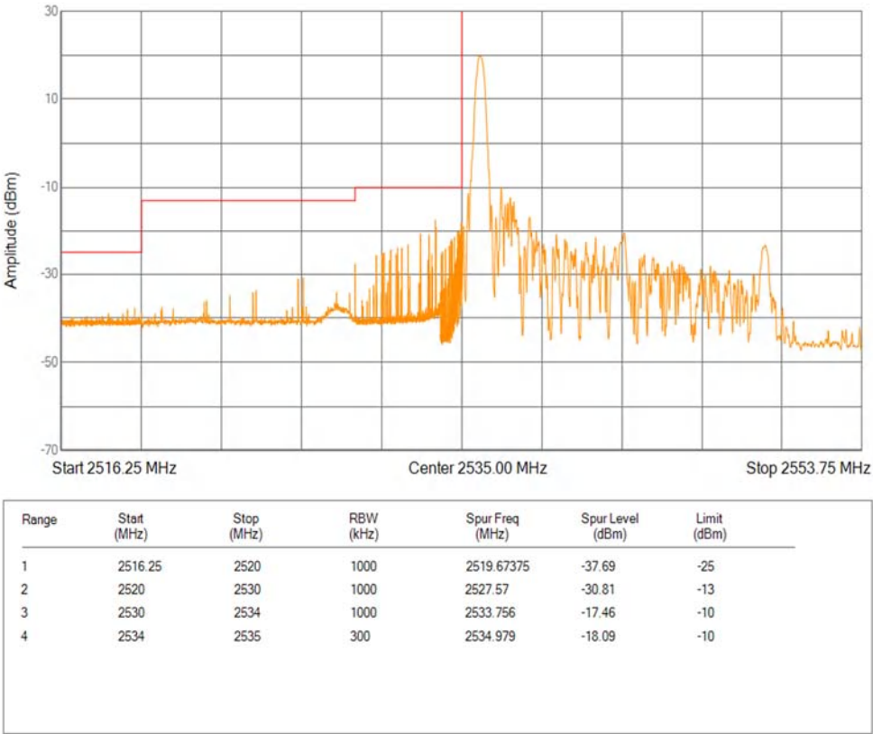
Band41(2535-2655) QPSK BW=15MHz Channel=40115 RB Size=1 Position=#0 Extended
