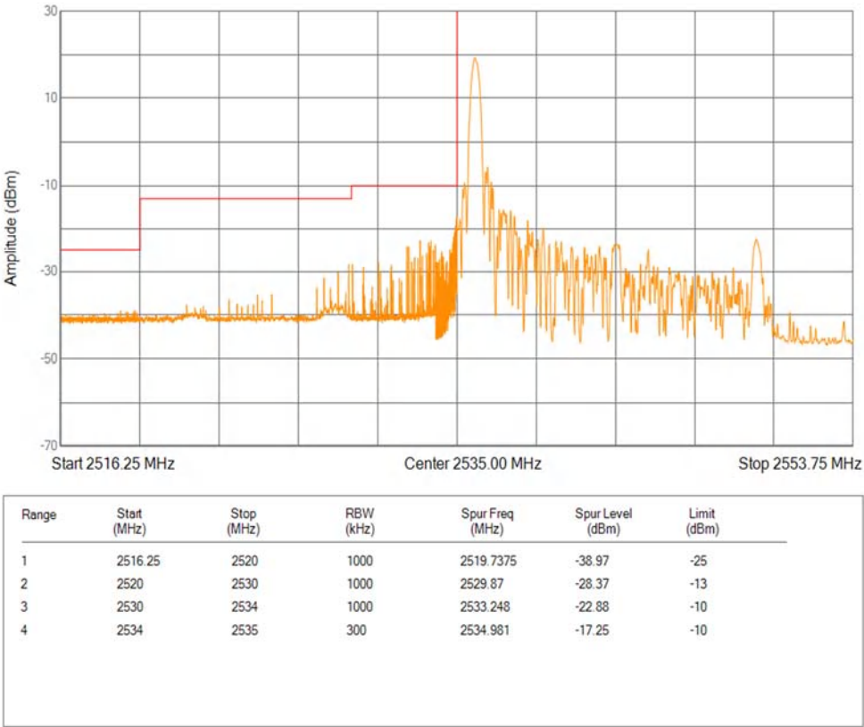
Band41(2535-2655) 16QAM BW=15MHz Channel=40115 RB Size=1 Position=#0 Extended
