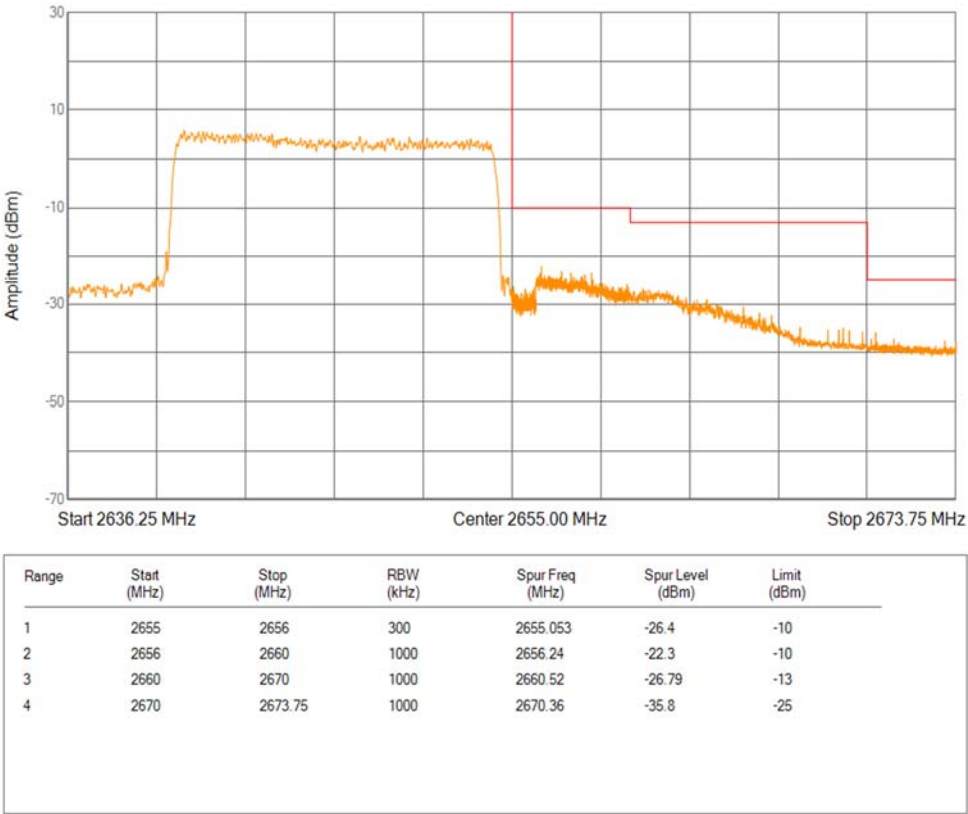
Band41(2535-2655) 16QAM BW=15MHz Channel=41165 RB Size=75 Position=#0 Extended
