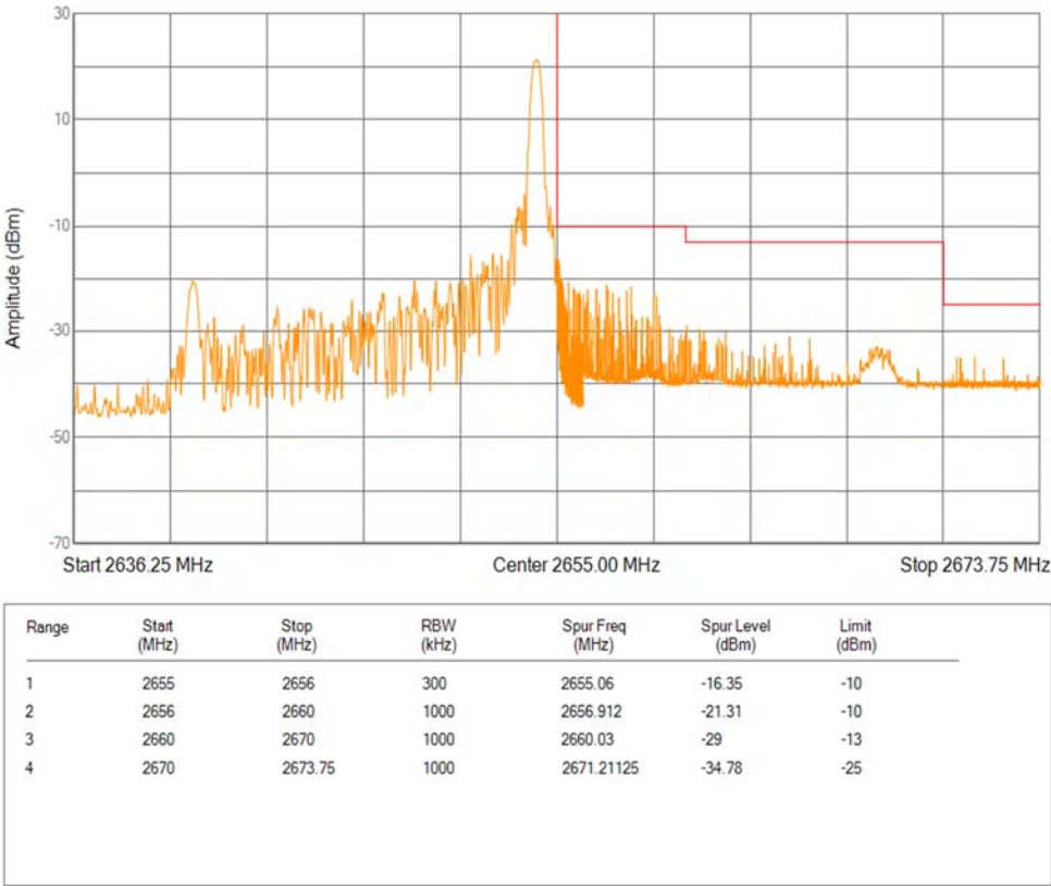
Band41(2535-2655) 16QAM BW=15MHz Channel=41165 RB Size=1 Position=#Max Extended
