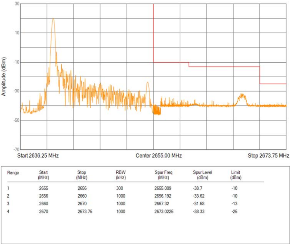
Band41(2535-2655) 16QAM BW=15MHz Channel=41165 RB Size=1 Position=#0 Extended
