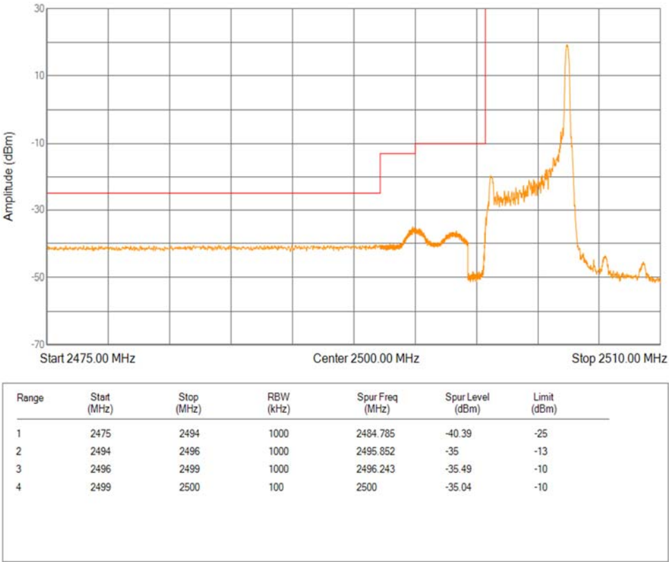
Band7 16QAM BW=5MHz Channel=20775 RB Size=1 Position=#Max Extended
