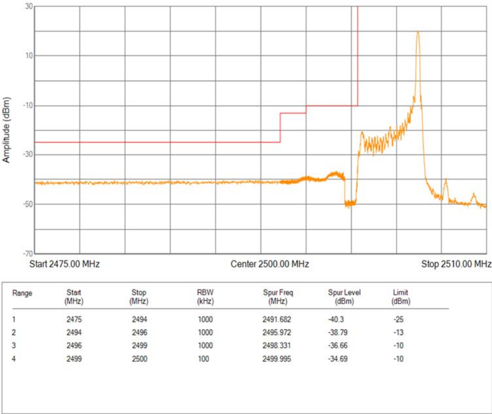
Band7 QPSK BW=5MHz Channel=20775 RB Size=1 Position=#Max Extended
