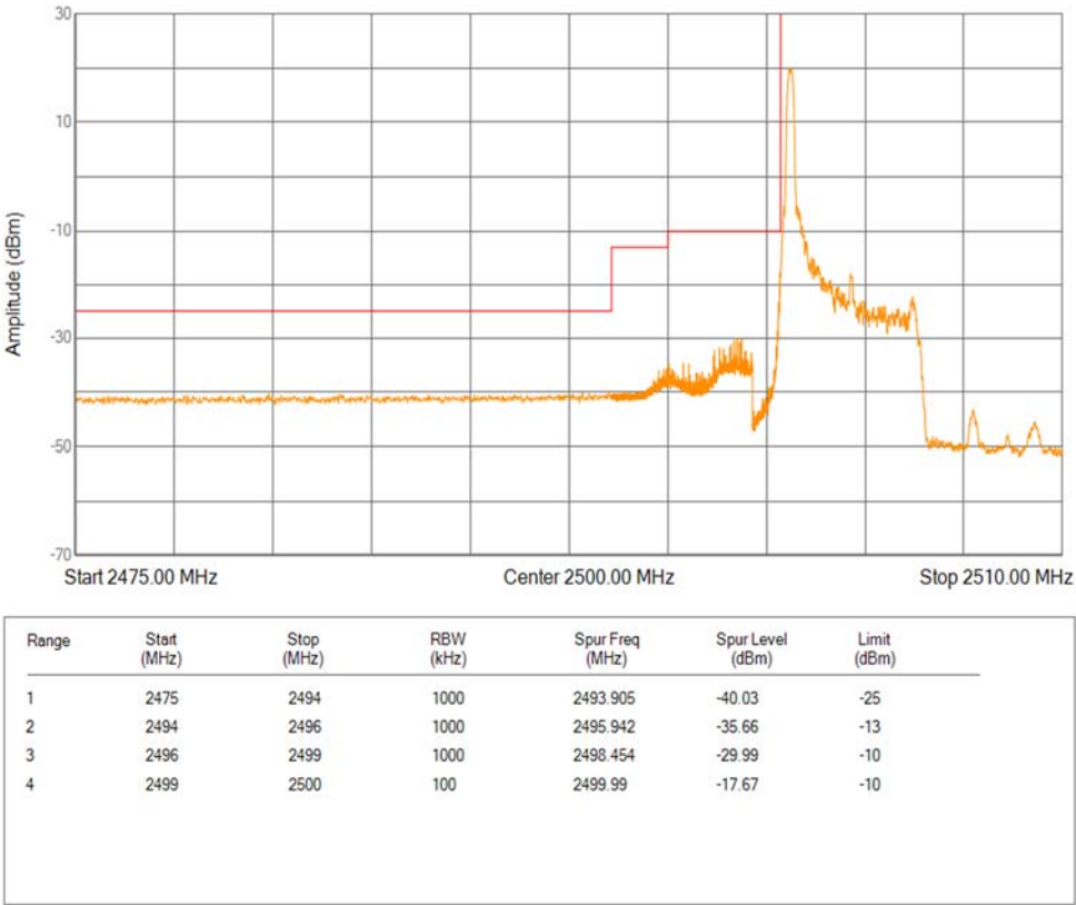
Band7 QPSK BW=5MHz Channel=20775 RB Size=1 Position=#0 Extended
