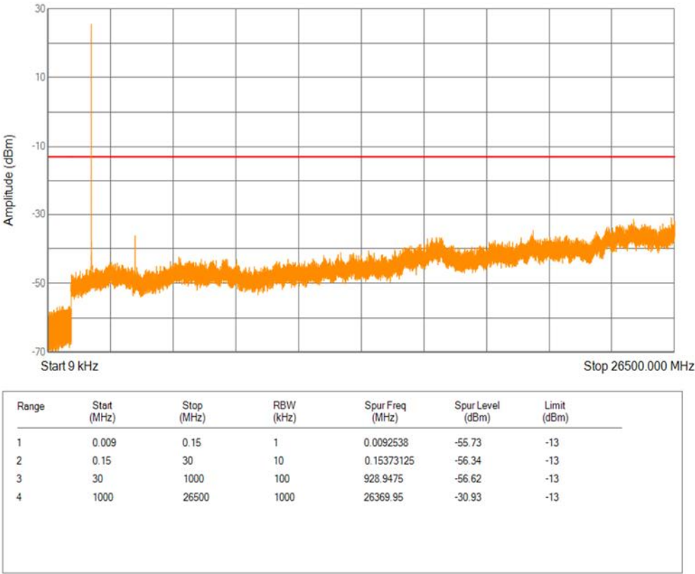
Band2 QPSK BW=1.4MHz Channel=18900 RB Size=1 Position=#0
