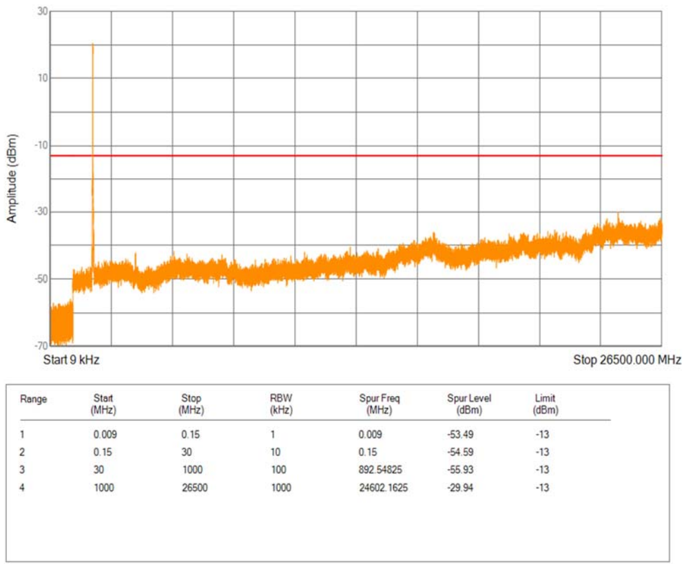
Band2 16QAM BW=15MHz Channel=18675 RB Size=1 Position=#0
