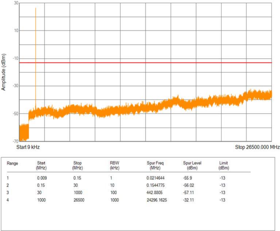
Band4 16QAM BW=1.4MHz Channel=20175 RB Size=1 Position=#0
