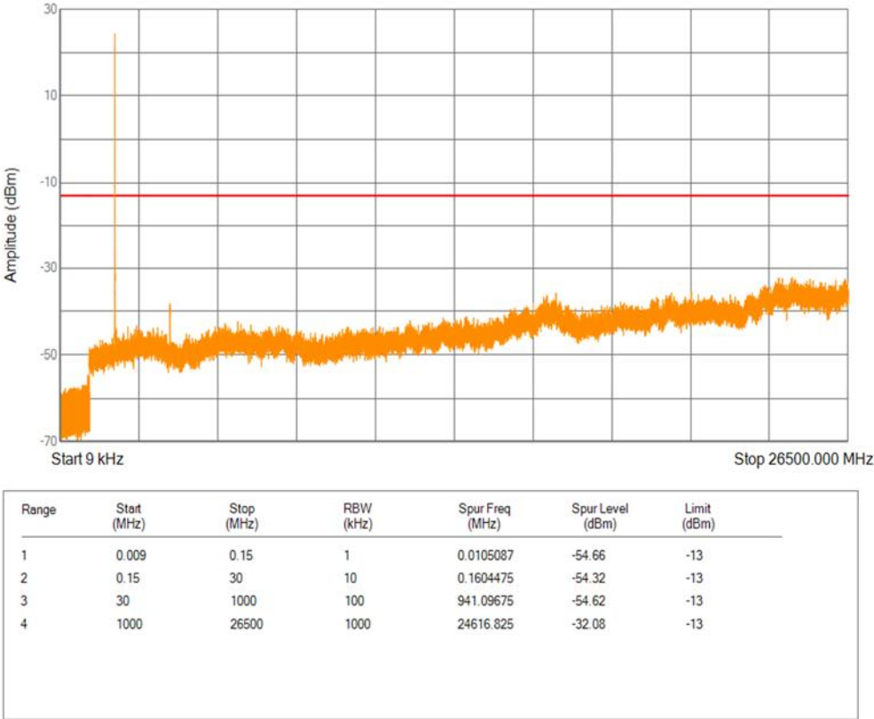
Band2 16QAM BW=3MHz Channel=18615 RB Size=1 Position=#0
