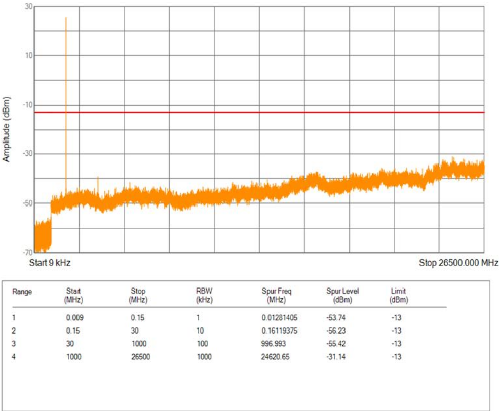
Band2 QPSK BW=1.4MHz Channel=19193 RB Size=1 Position=#0
