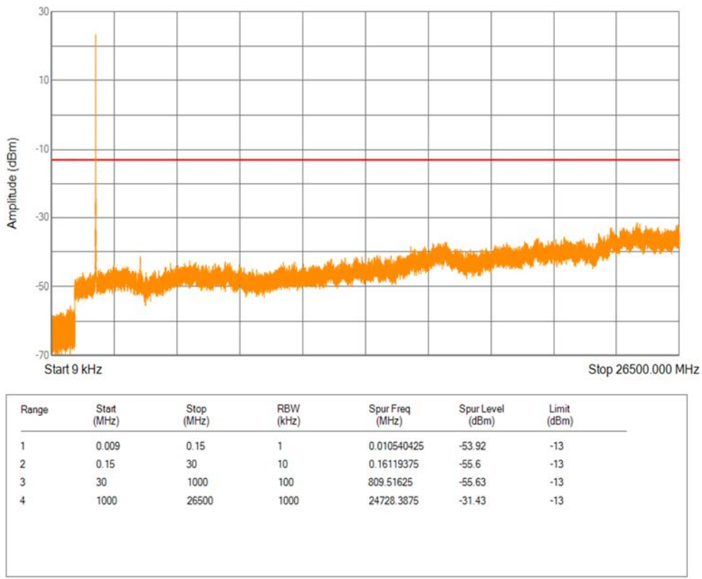
Band2 16QAM BW=5MHz Channel=18900 RB Size=1 Position=#0
