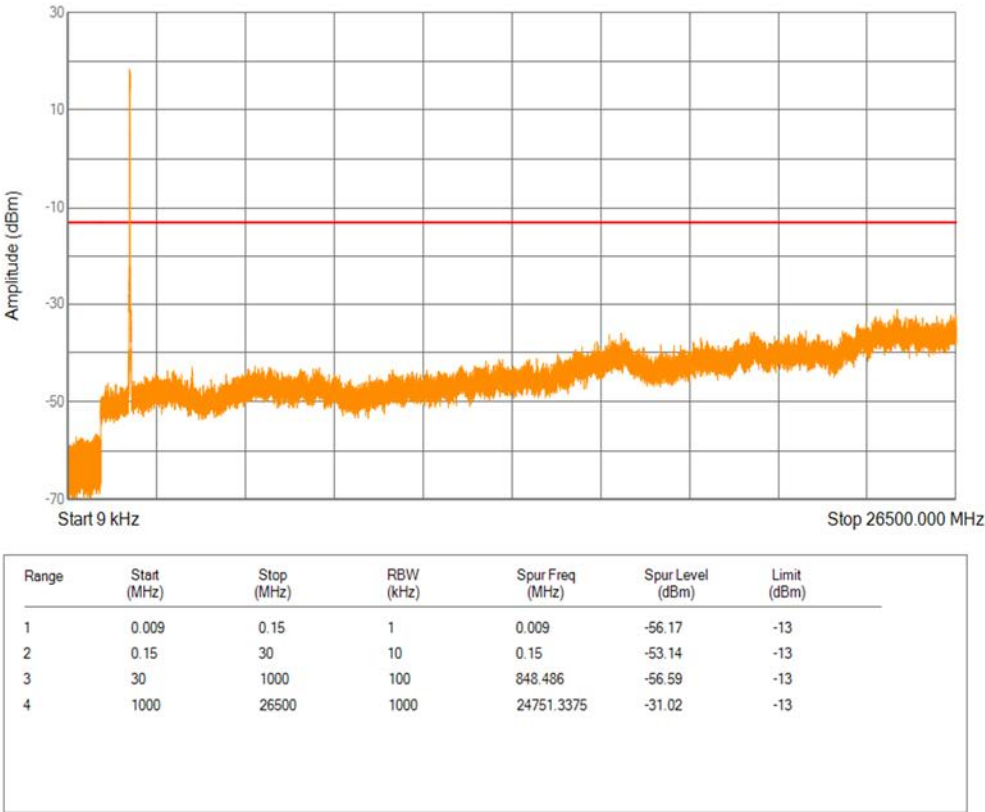
Band2 QPSK BW=20MHz Channel=18900 RB Size=1 Position=#0
