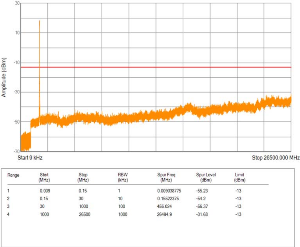
Band2 QPSK BW=15MHz Channel=18900 RB Size=1 Position=#0
