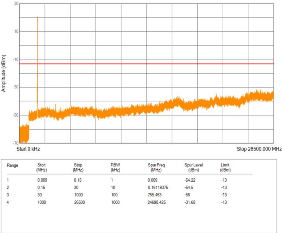
Band2 16QAM BW=15MHz Channel=19125 RB Size=1 Position=#0
