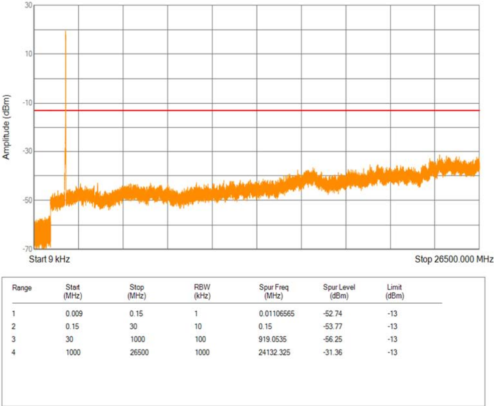
Band2 16QAM BW=20MHz Channel=19100 RB Size=1 Position=#0
