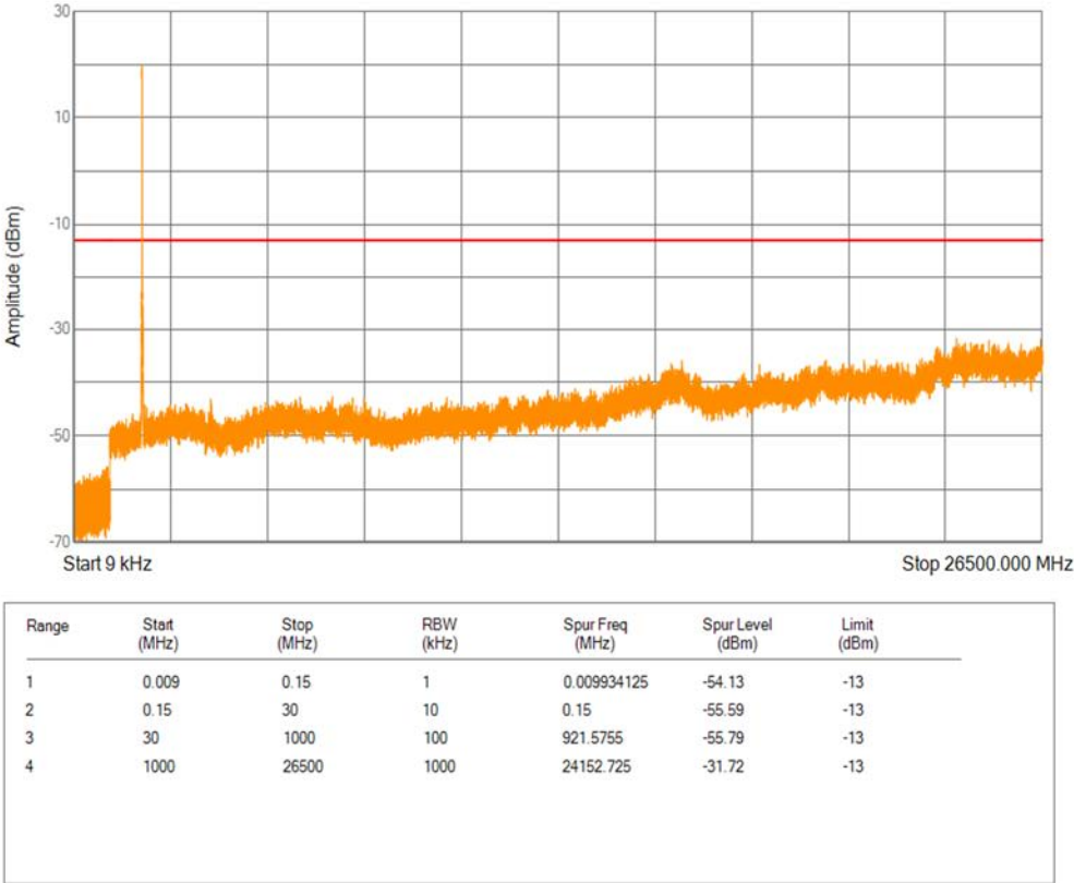
Band2 QPSK BW=10MHz Channel=19150 RB Size=1 Position=#0
