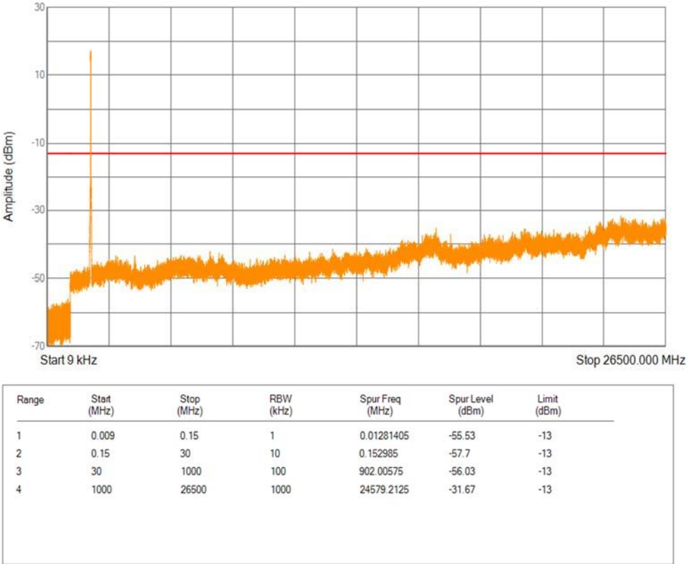
Band2 QPSK BW=20MHz Channel=19100 RB Size=1 Position=#0
