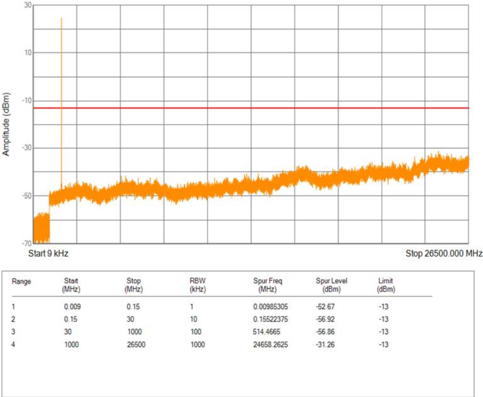
Band4 QPSK BW=1.4MHz Channel=20393 RB Size=1 Position=#0
