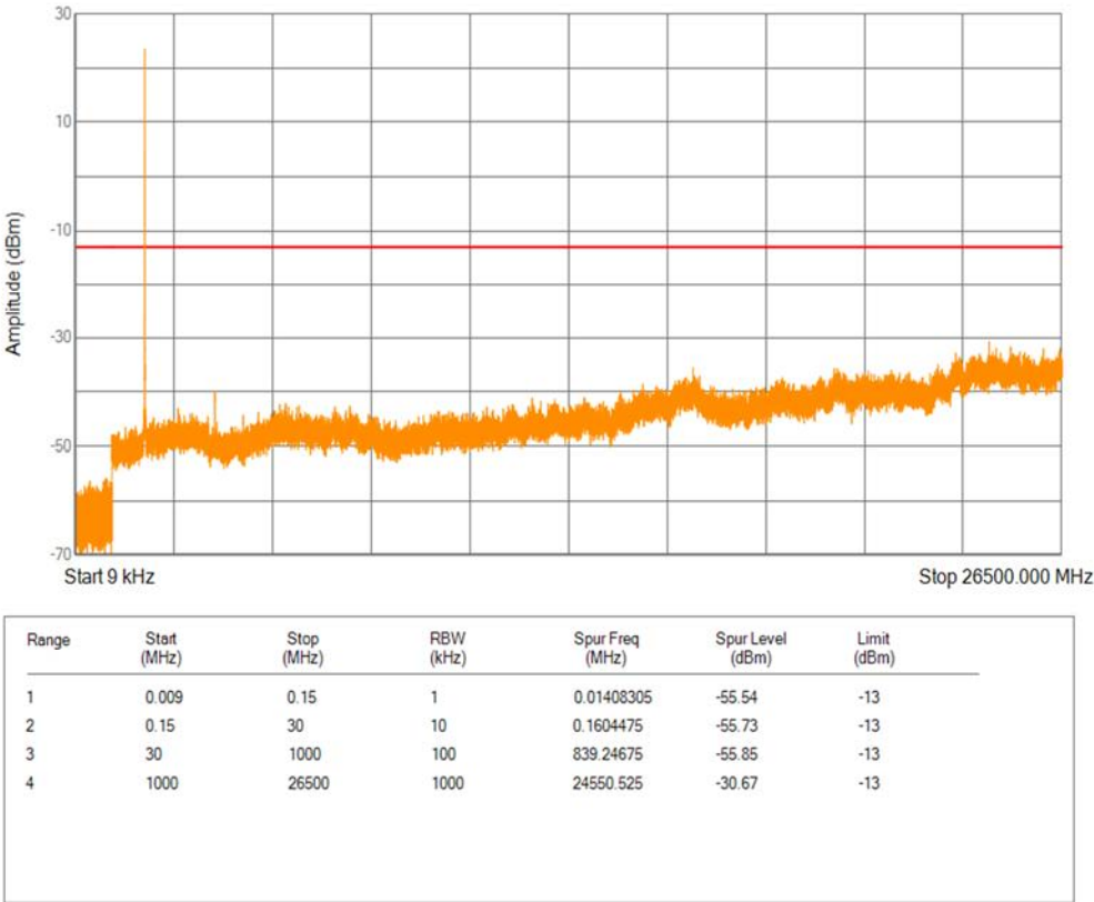
Band2 16QAM BW=3MHz Channel=18900 RB Size=1 Position=#0
