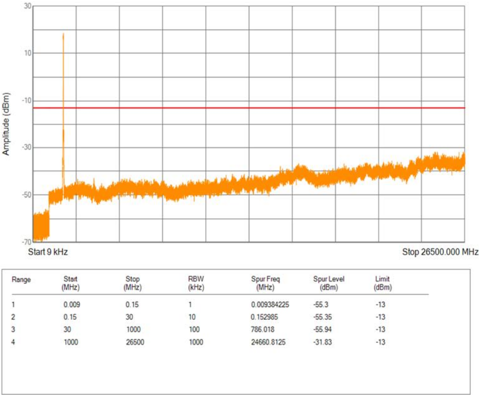
Band2 16QAM BW=20MHz Channel=18900 RB Size=1 Position=#0
