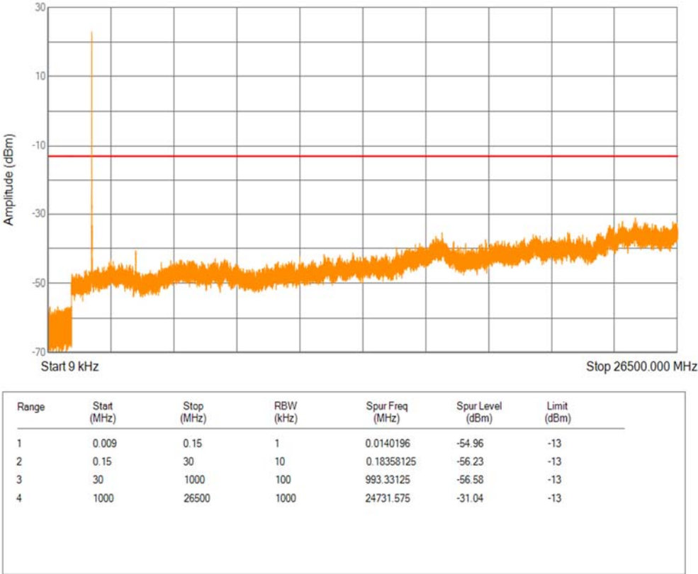
Band2 QPSK BW=5MHz Channel=18900 RB Size=1 Position=#0
