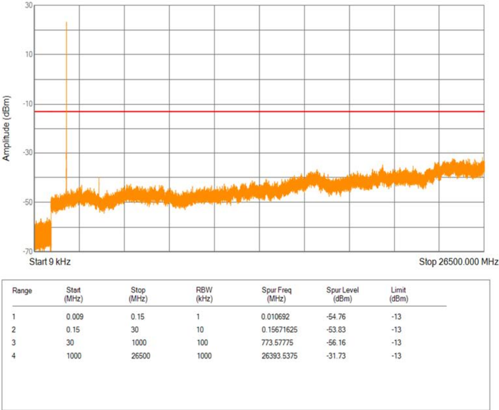
Band2 QPSK BW=5MHz Channel=18625 RB Size=1 Position=#0
