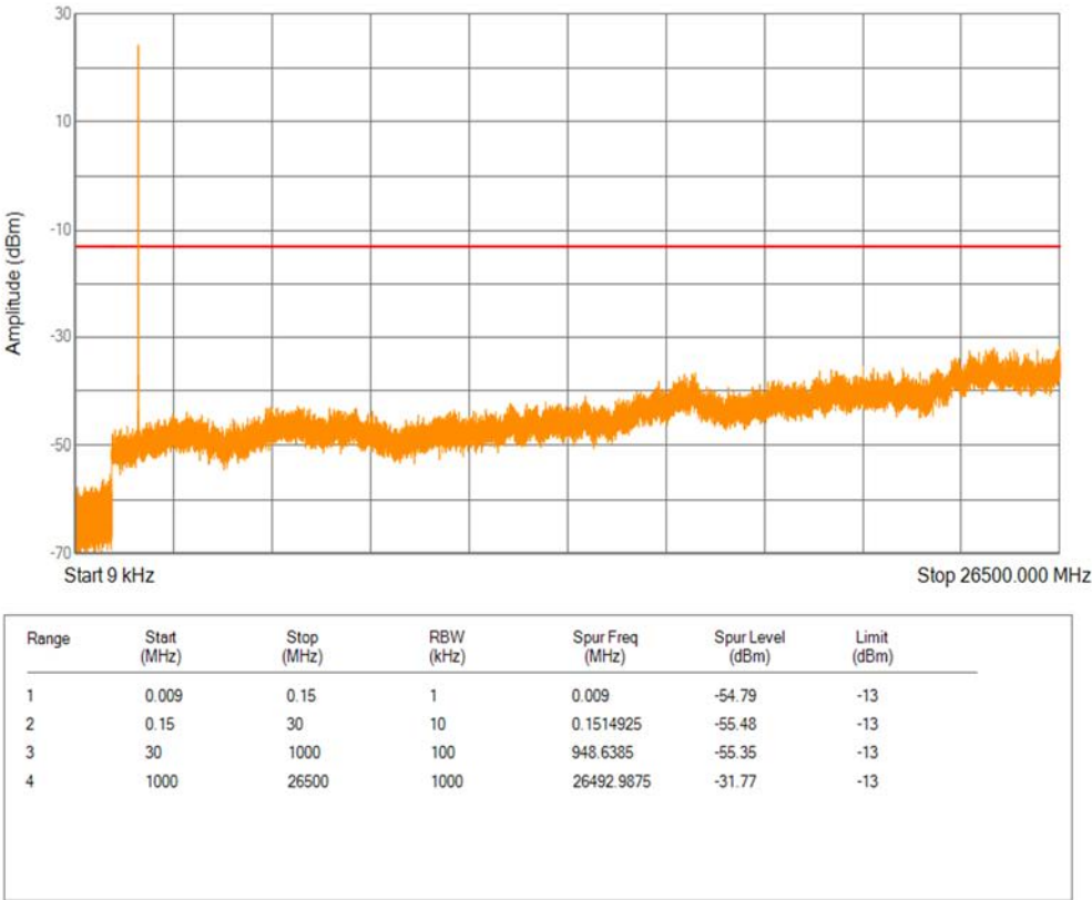
Band4 QPSK BW=1.4MHz Channel=20175 RB Size=1 Position=#0
