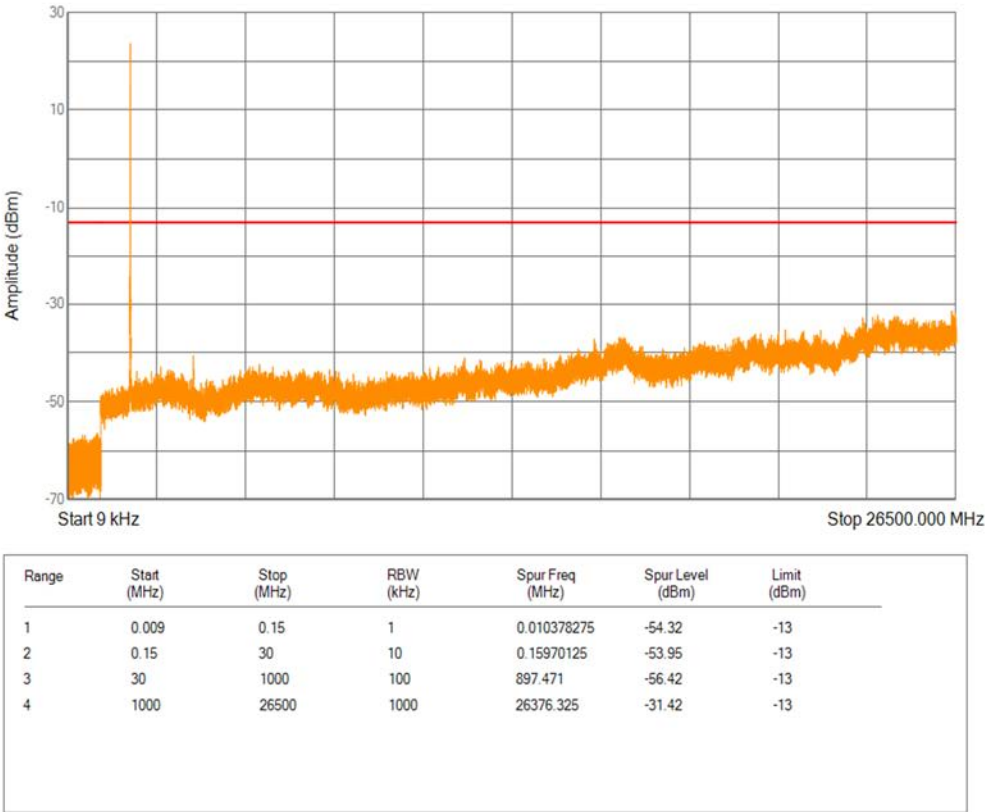
Band2 QPSK BW=5MHz Channel=19175 RB Size=1 Position=#0
