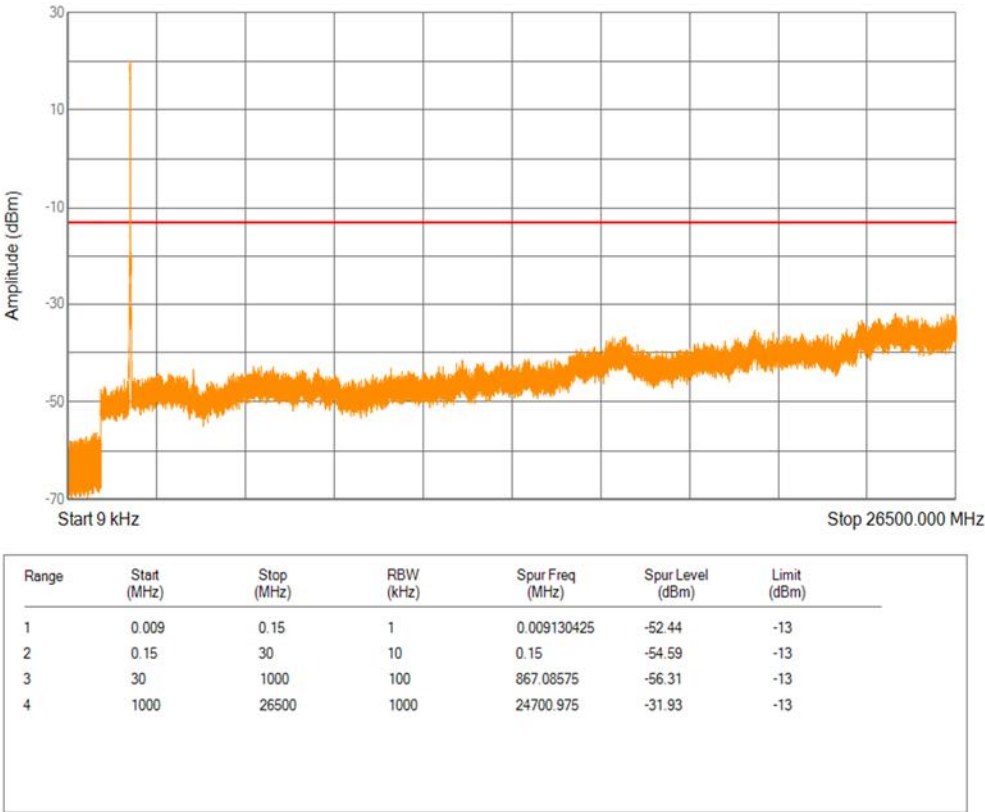
Band2 16QAM BW=15MHz Channel=18900 RB Size=1 Position=#0
