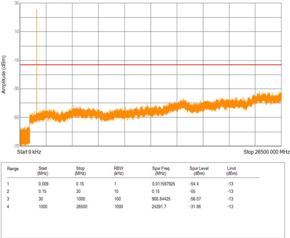
Band4 16QAM BW=1.4MHz Channel=19957 RB Size=1 Position=#0
