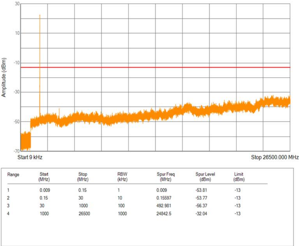
Band2 16QAM BW=5MHz Channel=19175 RB Size=1 Position=#0
