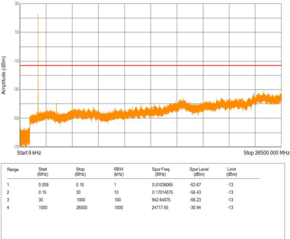
Band2 QPSK BW=3MHz Channel=18900 RB Size=1 Position=#0
