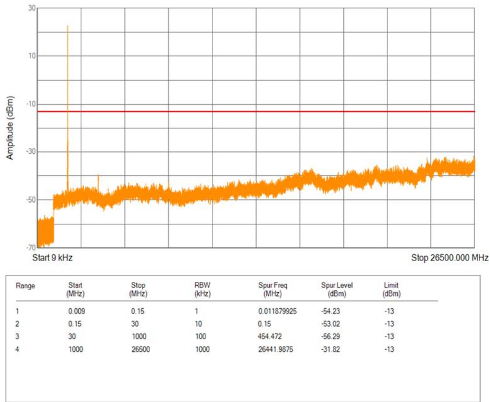
Band2 16QAM BW=5MHz Channel=18625 RB Size=1 Position=#0
