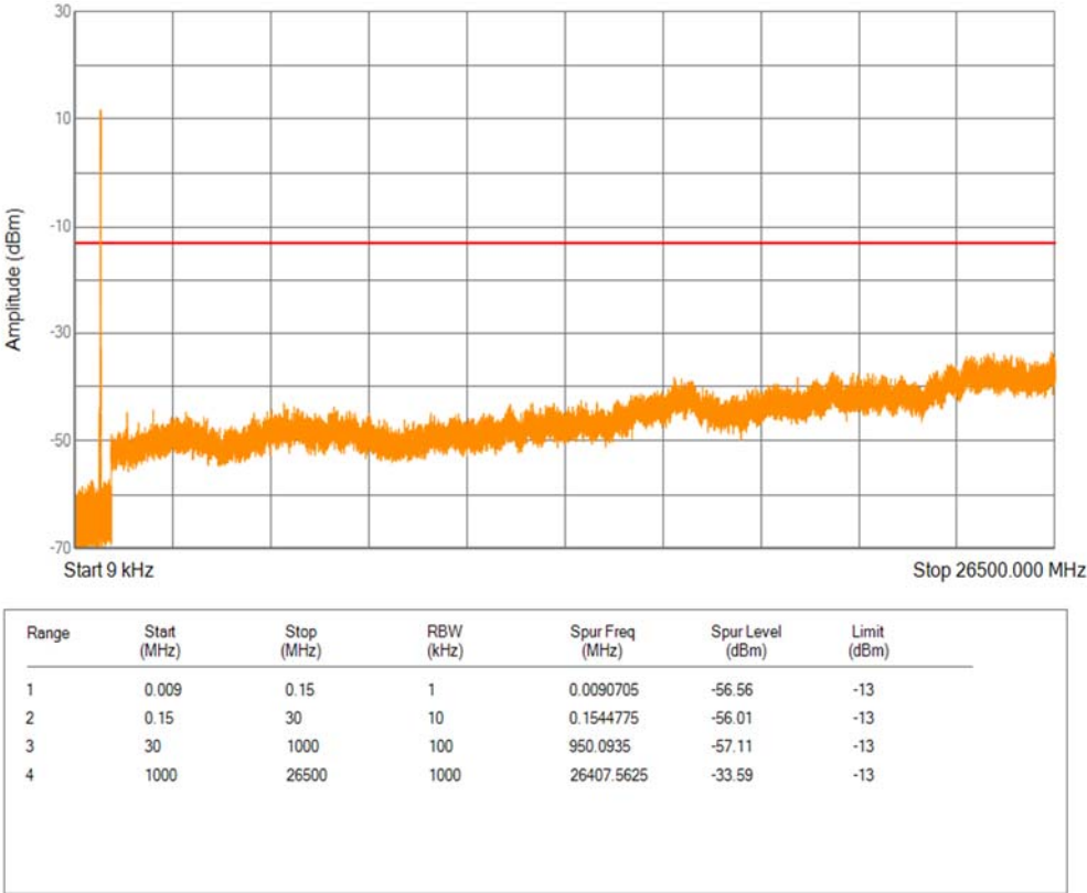
Band2 QPSK BW=1.4MHz Channel=18607 RB Size=1 Position=#0
