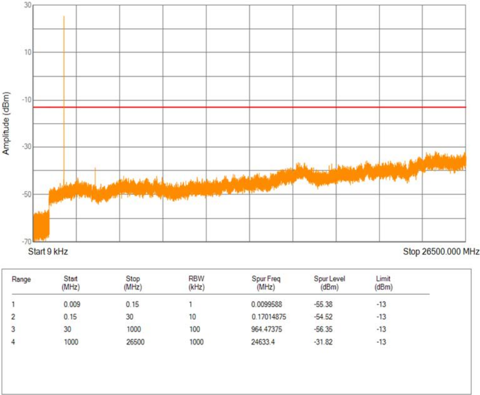
Band2 QPSK BW=3MHz Channel=18615 RB Size=1 Position=#0
