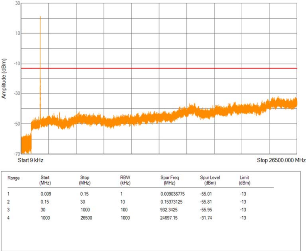
Band2 QPSK BW=10MHz Channel=18900 RB Size=1 Position=#0
