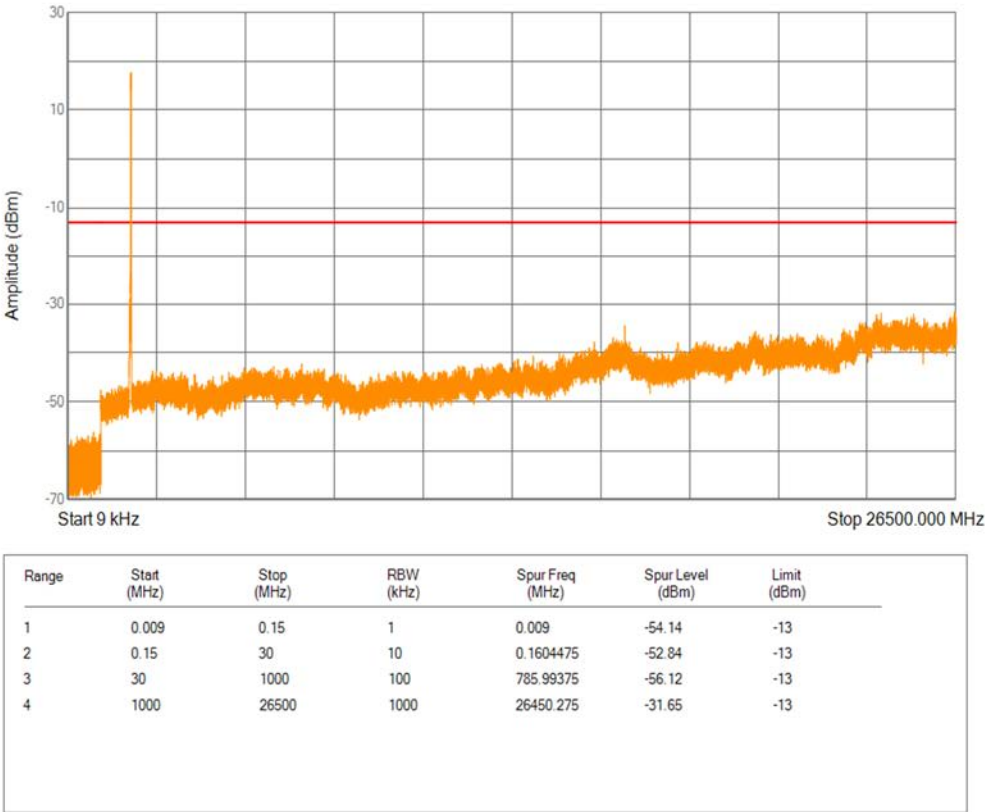
Band4 QPSK BW=1.4MHz Channel=19957 RB Size=1 Position=#0
