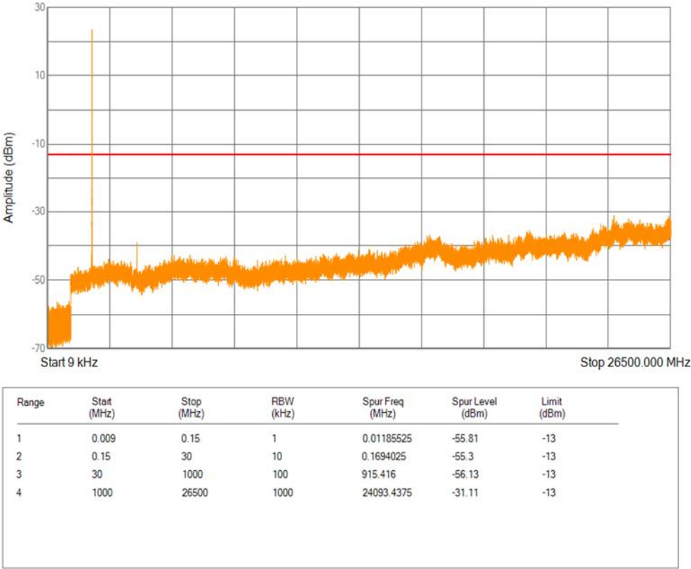
Band2 16QAM BW=3MHz Channel=19185 RB Size=1 Position=#0
