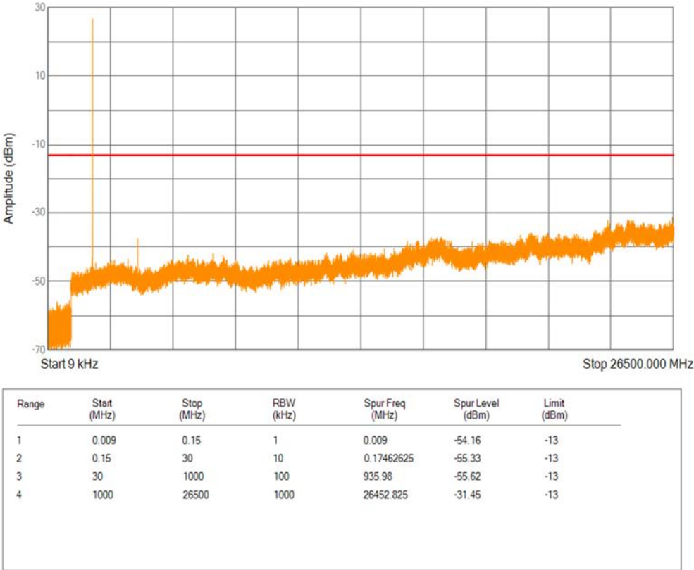
Band2 16QAM BW=1.4MHz Channel=19193 RB Size=1 Position=#0
