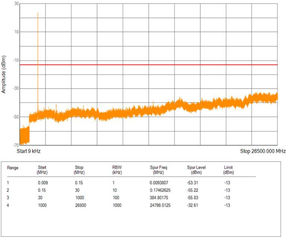
Band2 QPSK BW=3MHz Channel=19185 RB Size=1 Position=#0
