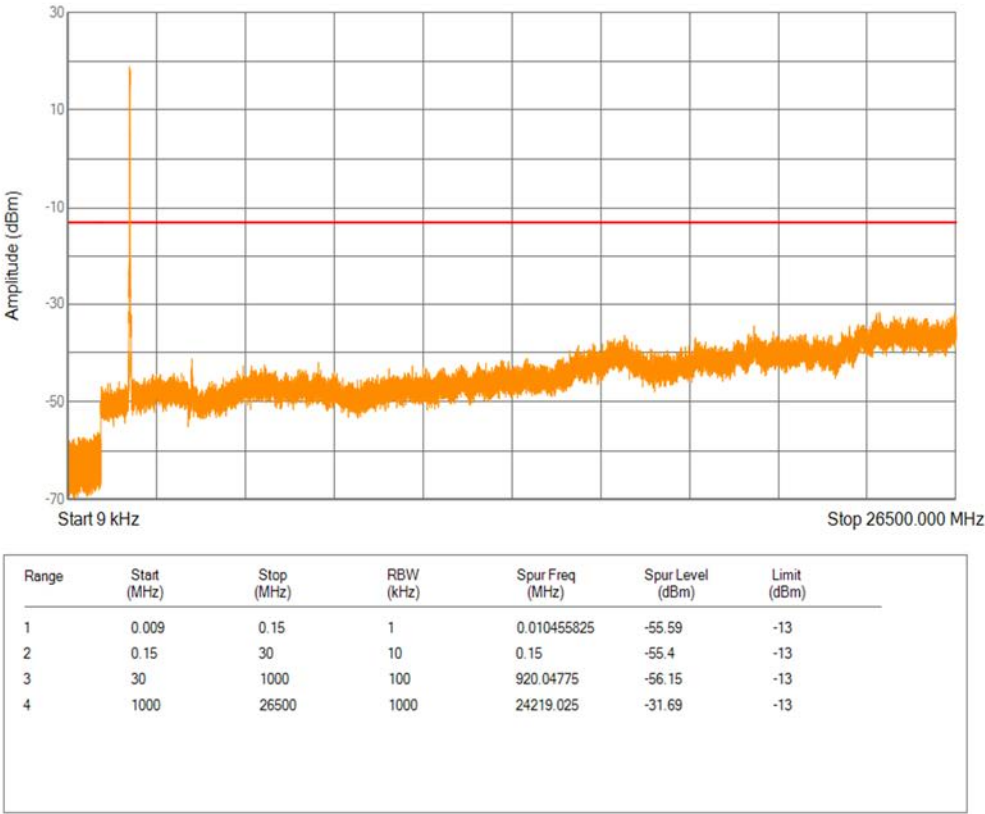
Band2 16QAM BW=20MHz Channel=18700 RB Size=1 Position=#0
