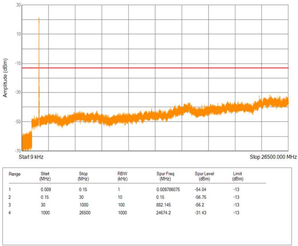
Band4 16QAM BW=10MHz Channel=20000 RB Size=1 Position=#0
