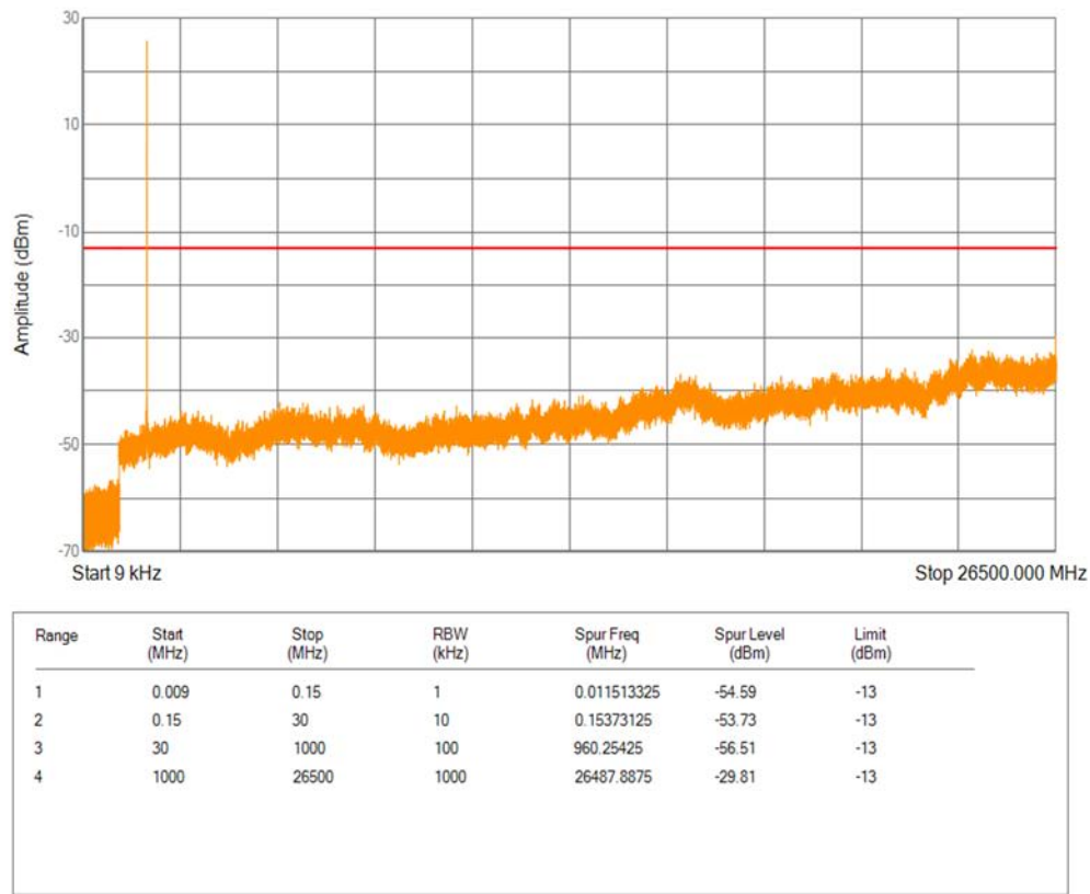
Band4 16QAM BW=1.4MHz Channel=20393 RB Size=1 Position=#0
