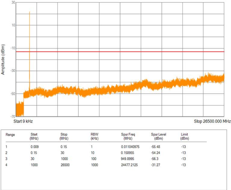
Band4 QPSK BW=10MHz Channel=20000 RB Size=1 Position=#0
