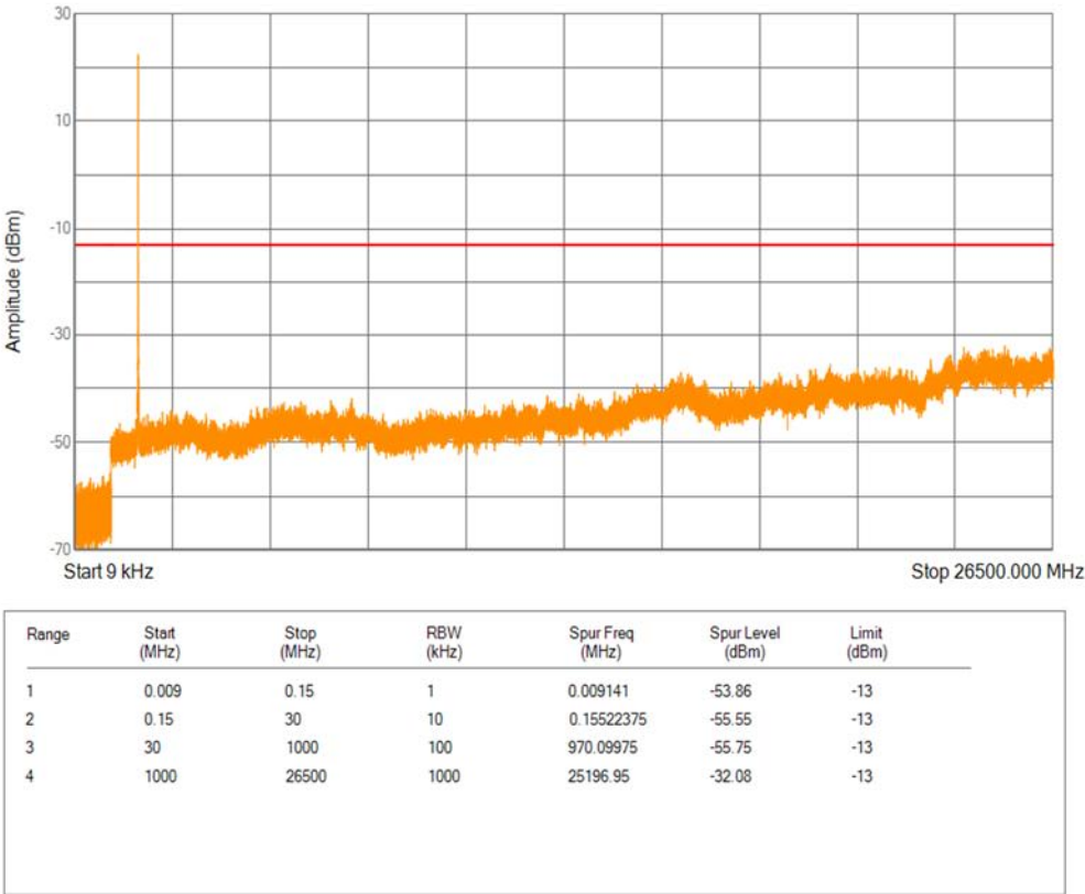
Band4 QPSK BW=5MHz Channel=20375 RB Size=1 Position=#0
