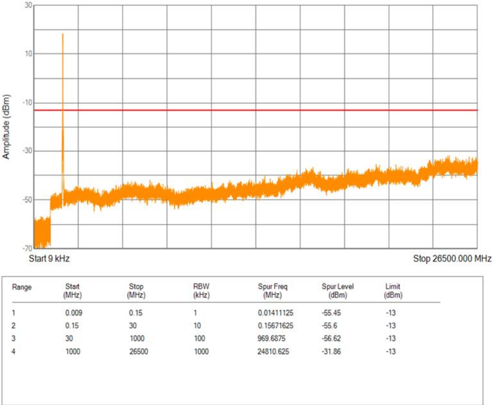
Band4 16QAM BW=20MHz Channel=20300 RB Size=1 Position=#0
