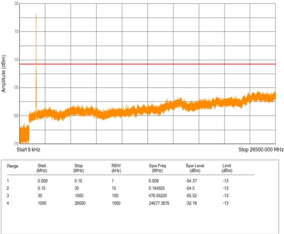
Band4 16QAM BW=10MHz Channel=20175 RB Size=1 Position=#0
