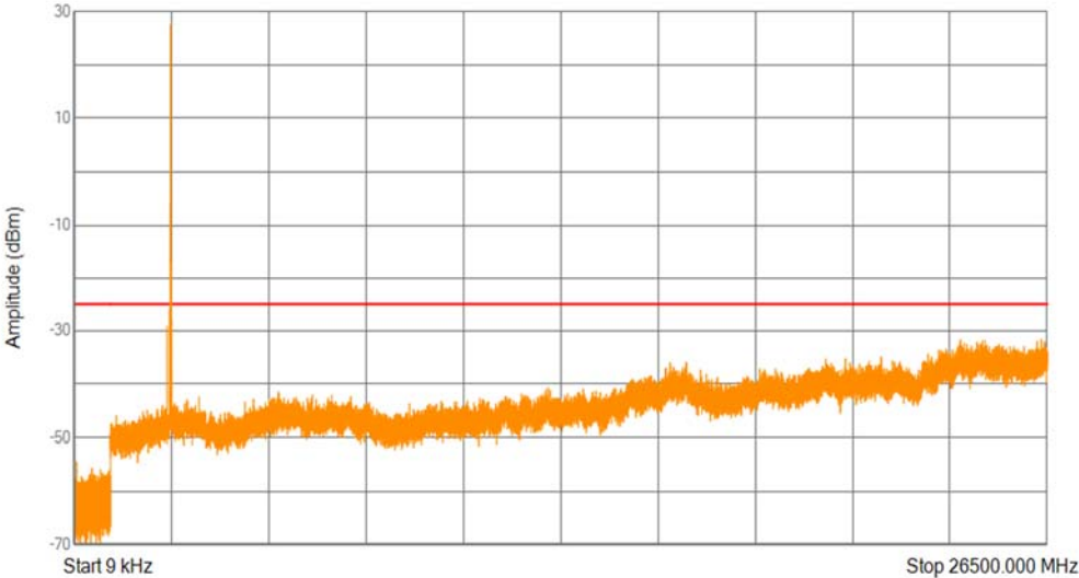
Band41(2535-2655) 16QAM BW=15MHz Channel=41165 RB Size=1 Position=#0
