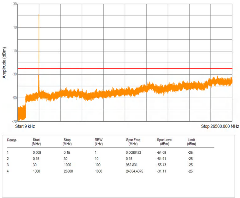
Band41(2535-2655) QPSK BW=15MHz Channel=40115 RB Size=1 Position=#0
