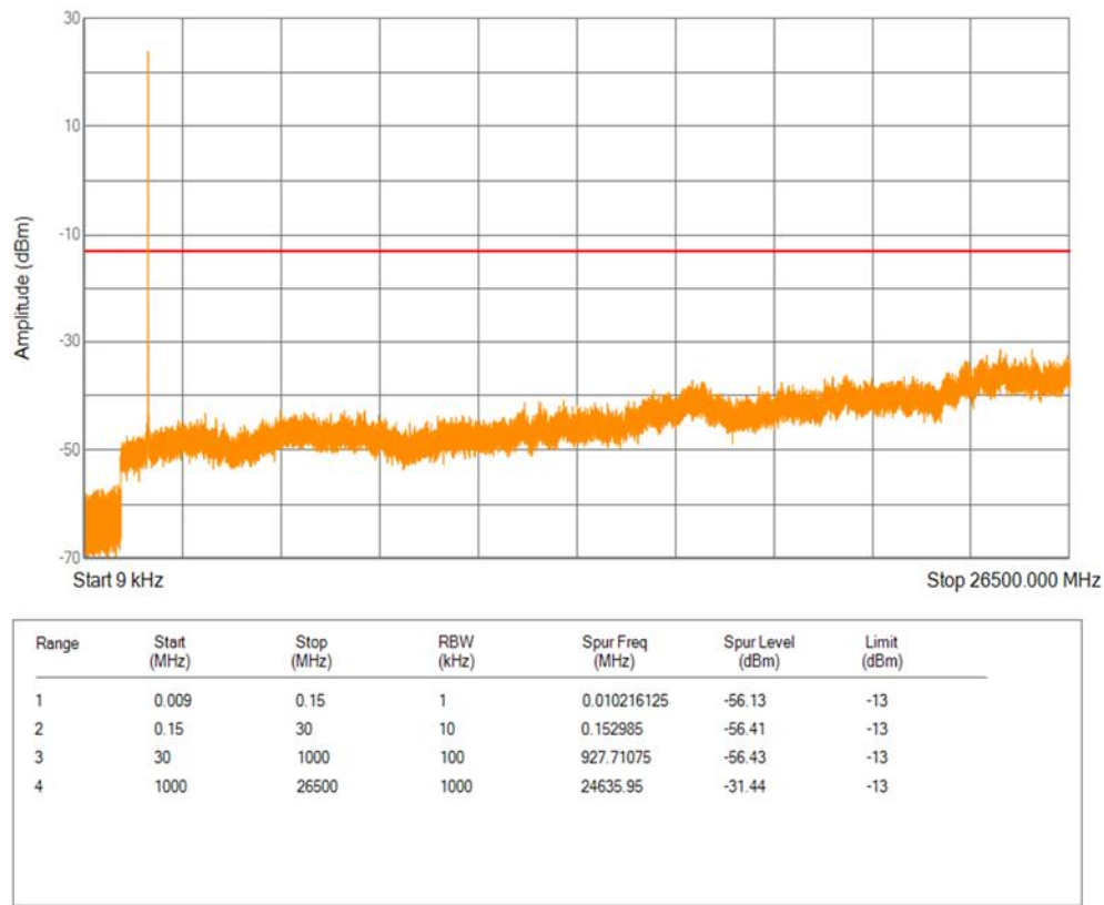
Band4 16QAM BW=3MHz Channel=20175 RB Size=1 Position=#0
