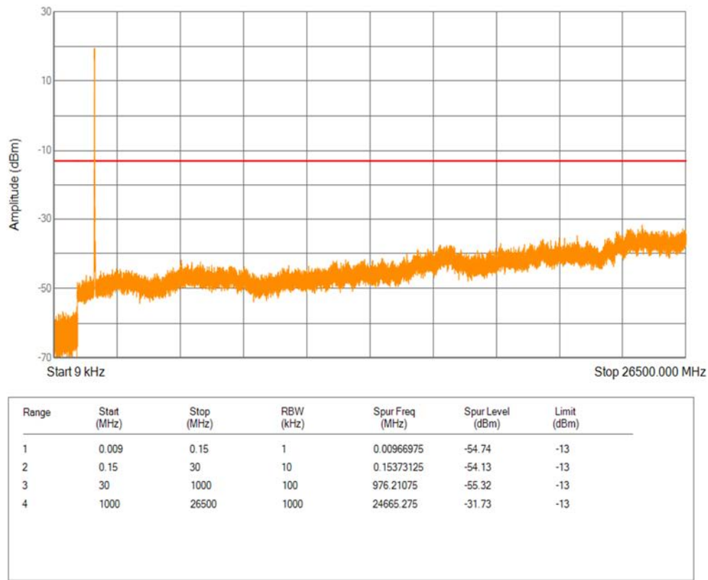
Band4 QPSK BW=10MHz Channel=20175 RB Size=1 Position=#0
