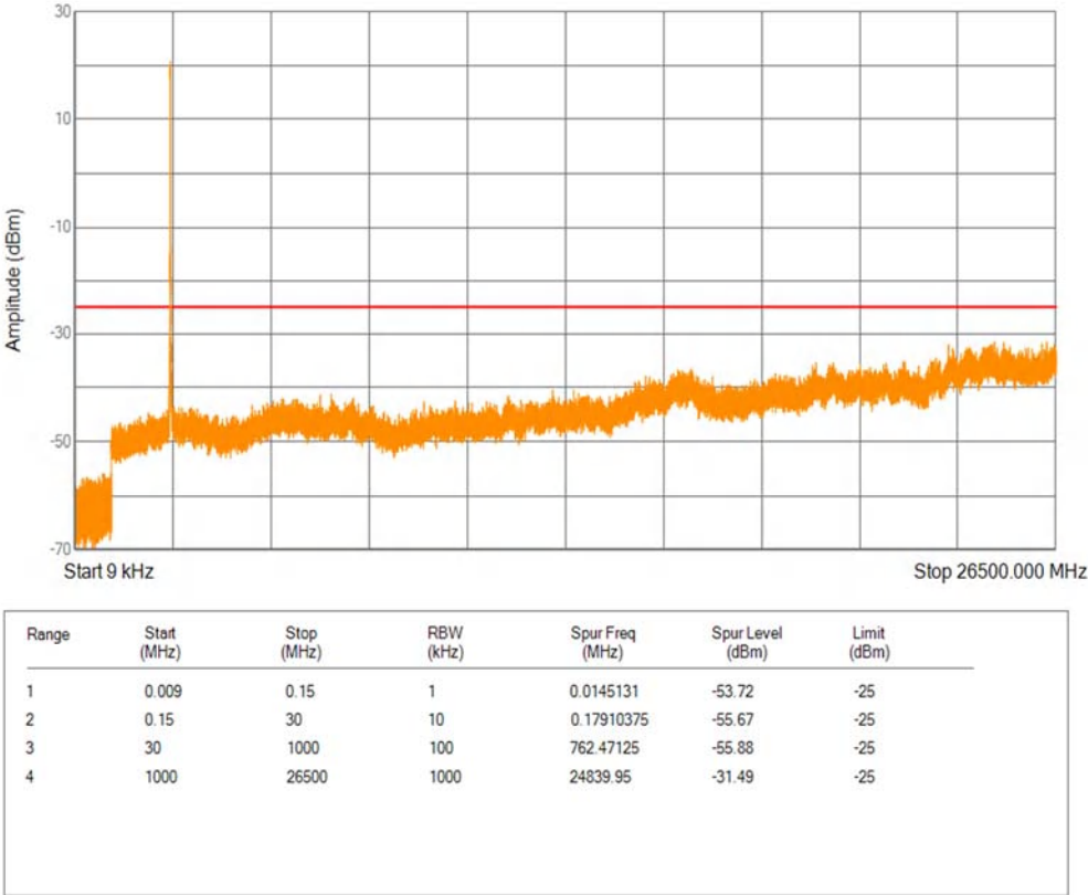
Band41(2535-2655) QPSK BW=10MHz Channel=41190 RB Size=1 Position=#0
