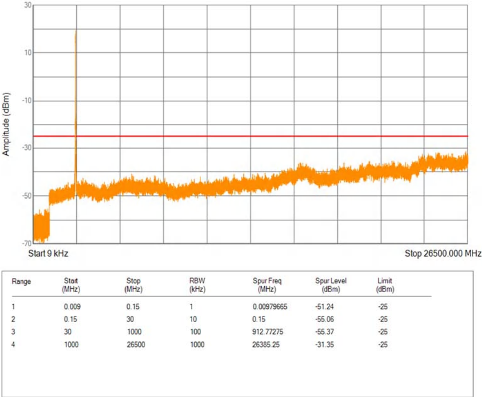
Band41(2535-2655) QPSK BW=15MHz Channel=41165 RB Size=1 Position=#0
