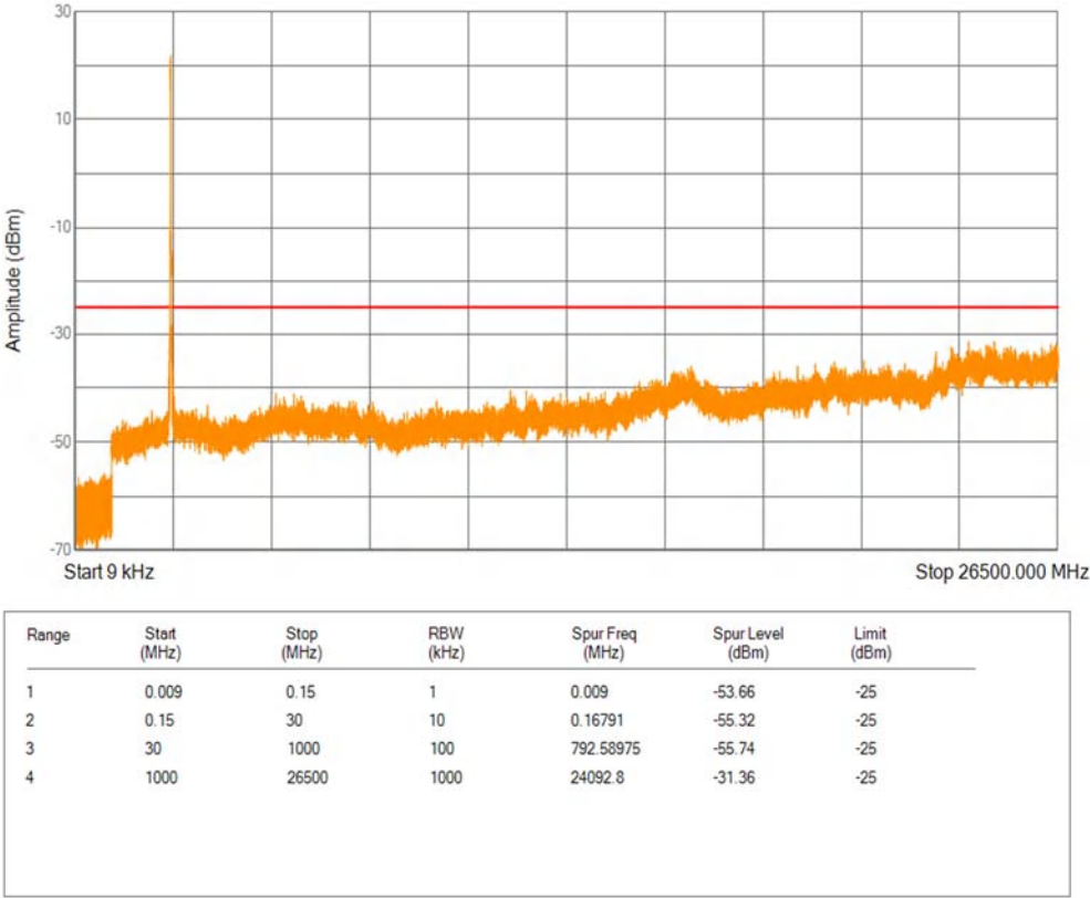
Band41(2535-2655) 16QAM BW=15MHz Channel=40640 RB Size=1 Position=#0
