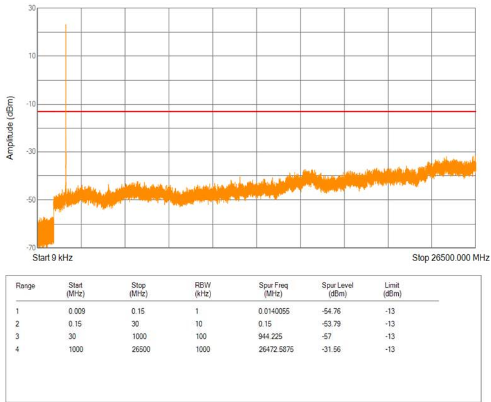
Band4 QPSK BW=3MHz Channel=20385 RB Size=1 Position=#0
