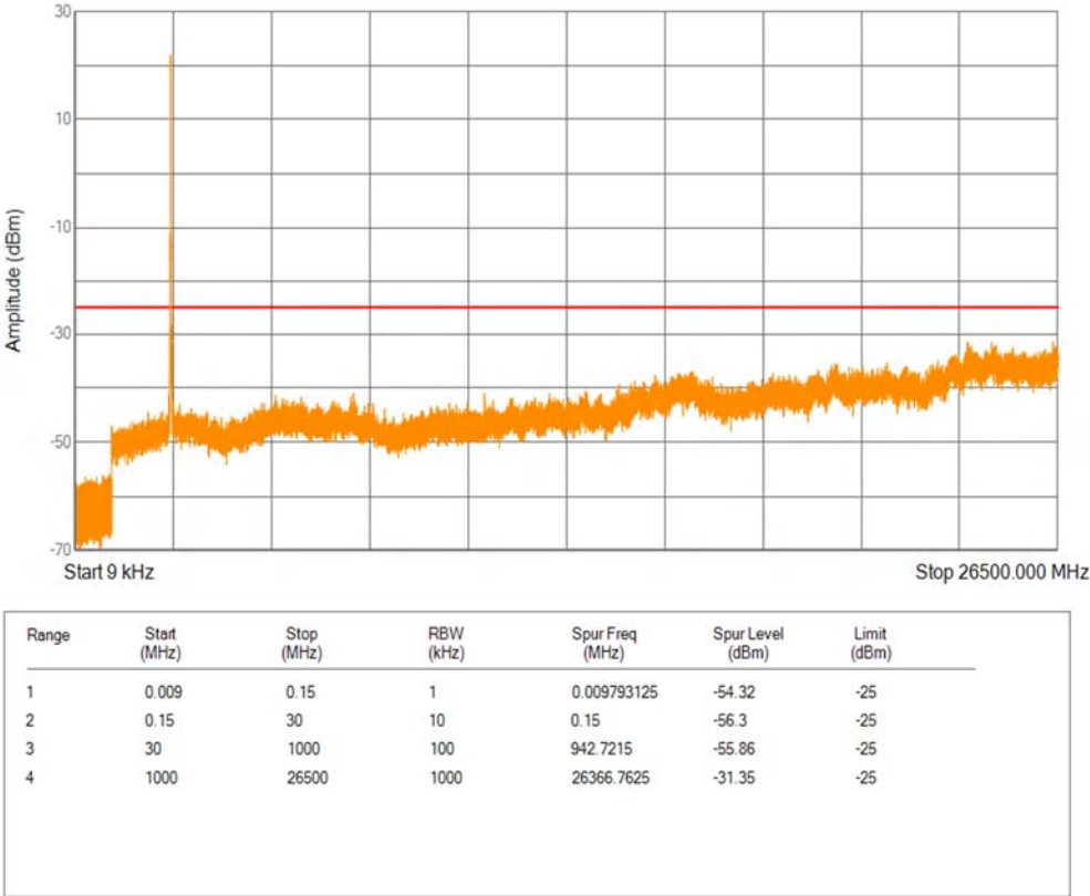
Band41(2535-2655) 16QAM BW=10MHz Channel=40640 RB Size=1 Position=#0
