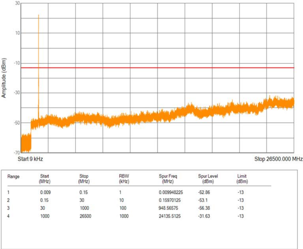
Band4 16QAM BW=5MHz Channel=20175 RB Size=1 Position=#0
