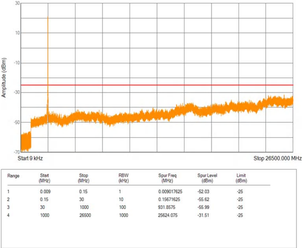
Band41(2535-2655) QPSK BW=20MHz Channel=40140 RB Size=1 Position=#0
