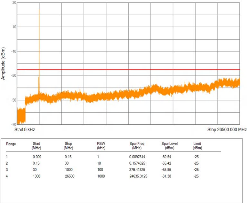
Band41(2535-2655) QPSK BW=10MHz Channel=40090 RB Size=1 Position=#0
