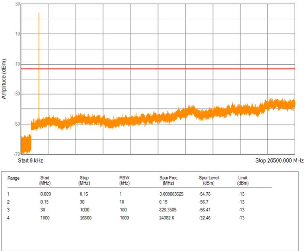
Band66 QPSK BW=3MHz Channel=132657 RB Size=1 Position=#0
