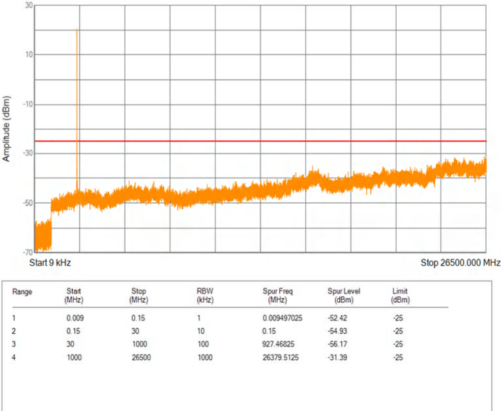
Band7 16QAM BW=5MHz Channel=21100 RB Size=1 Position=#0
