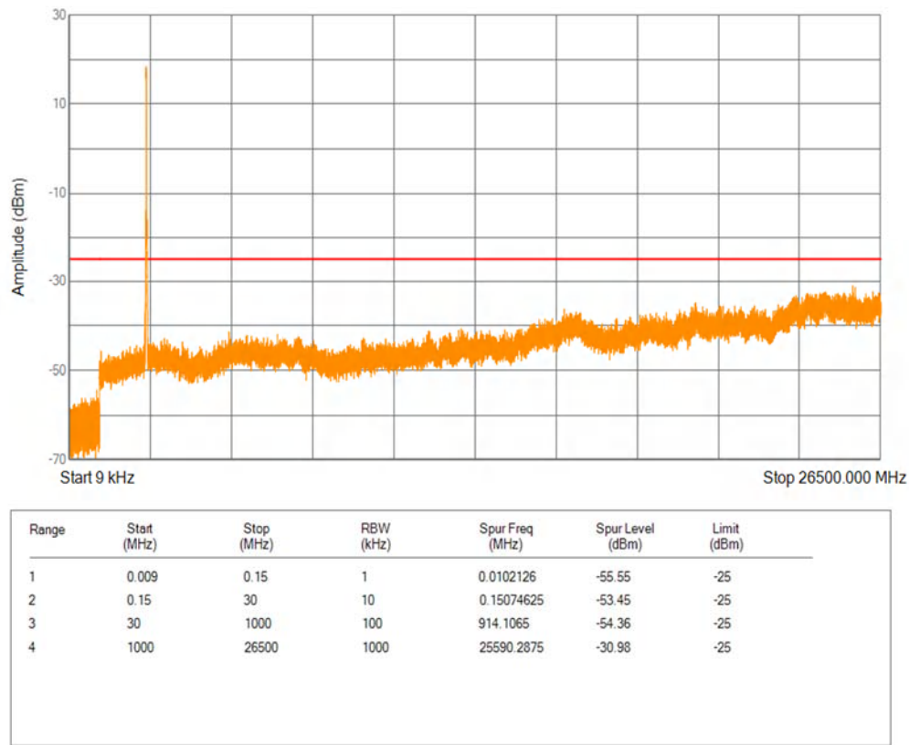
Band7 16QAM BW=20MHz Channel=21100 RB Size=1 Position=#0
