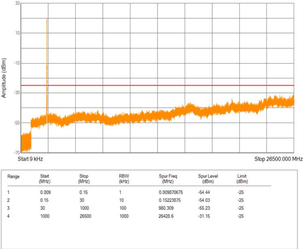
Band7 16QAM BW=15MHz Channel=21100 RB Size=1 Position=#0
