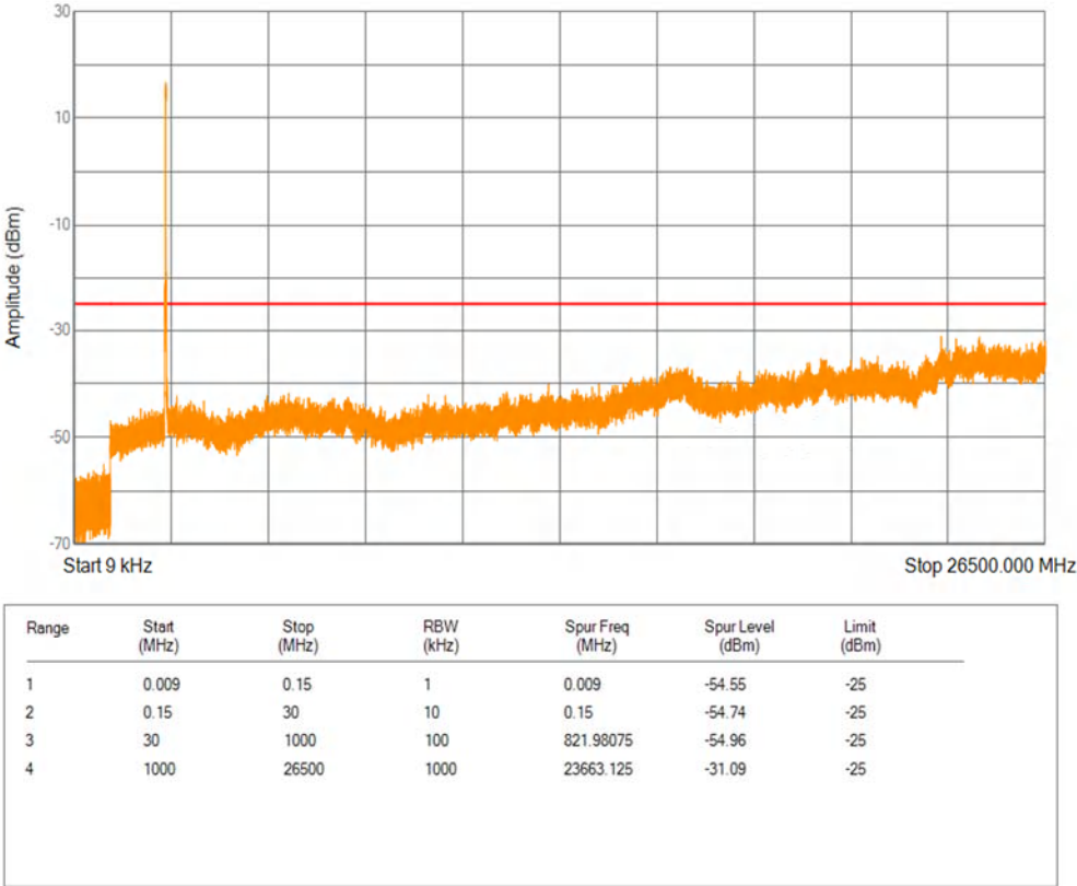
Band7 QPSK BW=20MHz Channel=21100 RB Size=1 Position=#0
