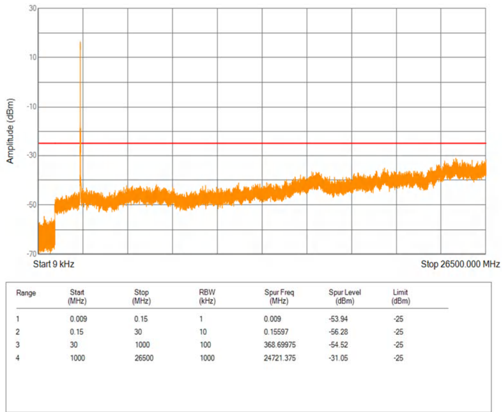
Band7 QPSK BW=15MHz Channel=21100 RB Size=1 Position=#0
