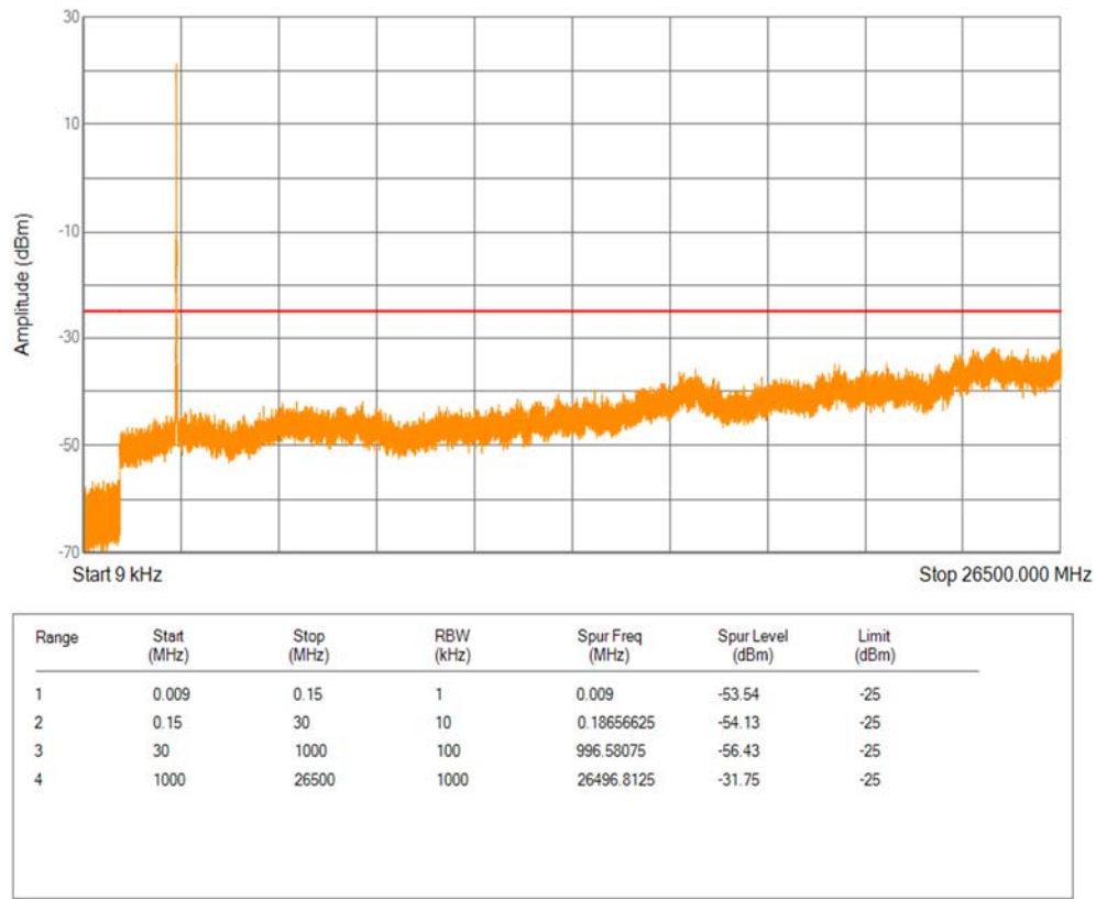
Band7 QPSK BW=10MHz Channel=21100 RB Size=1 Position=#0
