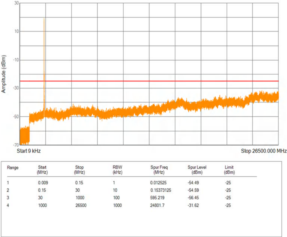
Band7 16QAM BW=10MHz Channel=21100 RB Size=1 Position=#0
