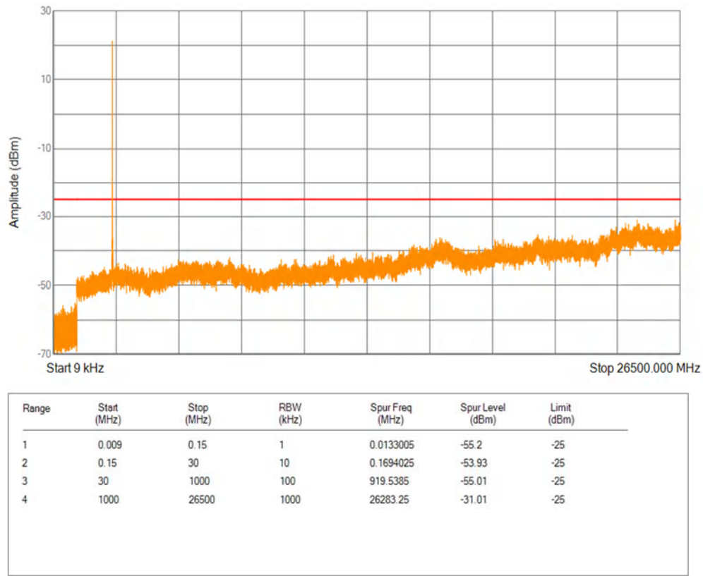
Band7 QPSK BW=5MHz Channel=21100 RB Size=1 Position=#0
