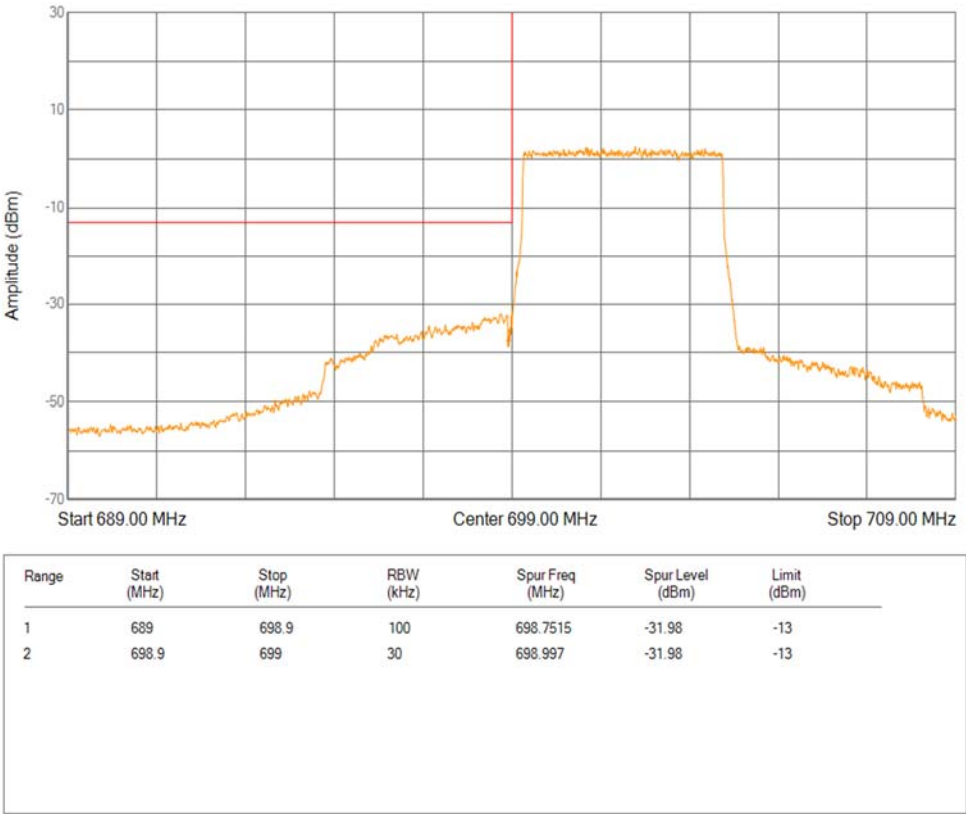
Band12 QPSK BW=5MHz Channel=23035 RB Size=25 Position=#0 Extended
