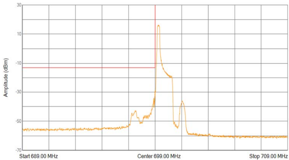
Band12 QPSK BW=1.4MHz Channel=23017 RB Size=1 Position=#0 Normal
