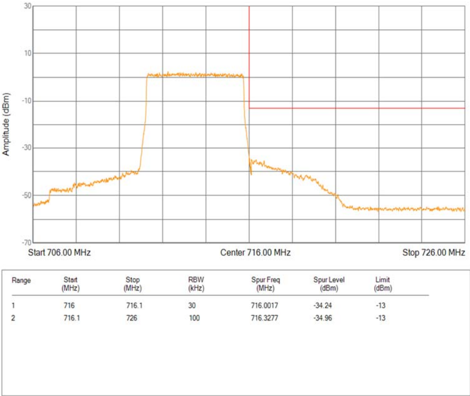
Band12 QPSK BW=5MHz Channel=23155 RB Size=25 Position=#0 Extended
