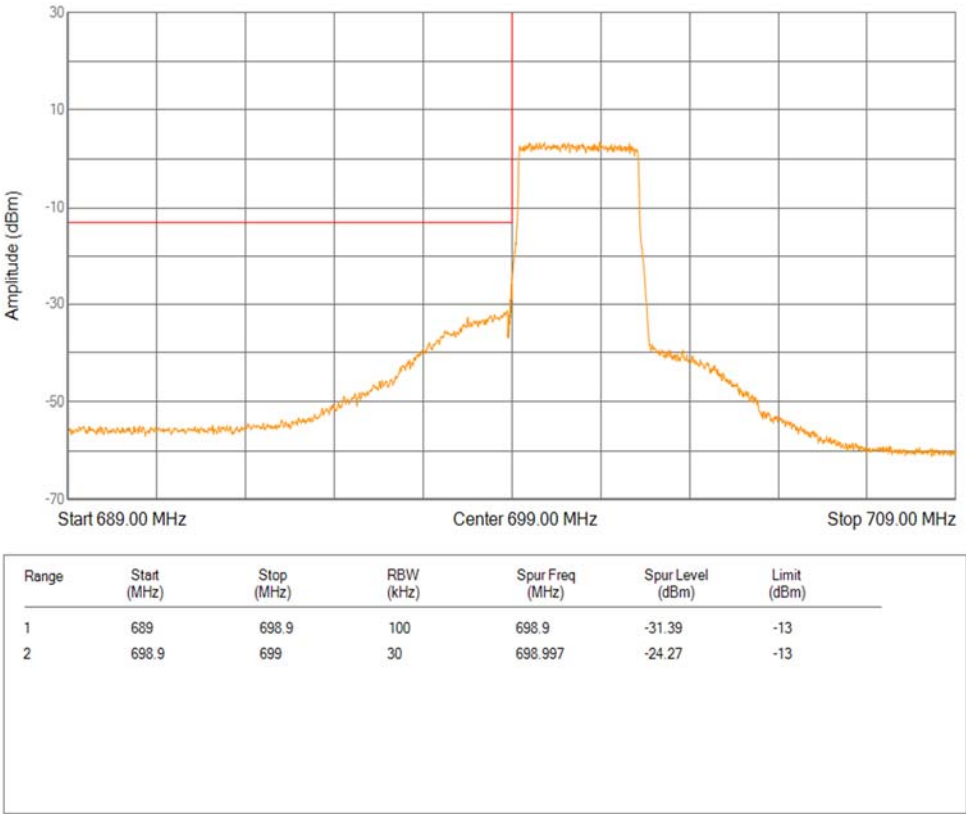
Band12 16QAM BW=3MHz Channel=23025 RB Size=15 Position=#0 Extended
