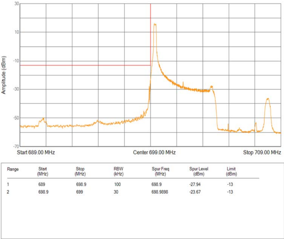
Band12 QPSK BW=5MHz Channel=23035 RB Size=1 Position=#0 Extended
