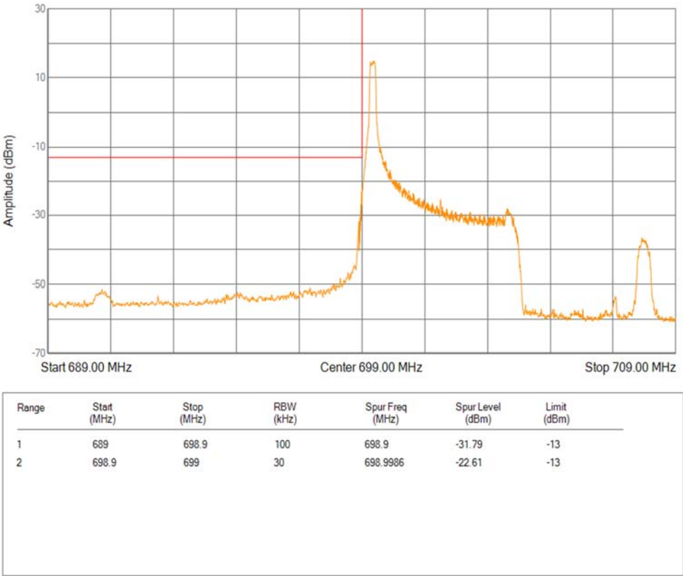
Band12 16QAM BW=5MHz Channel=23035 RB Size=1 Position=#0 Extended
