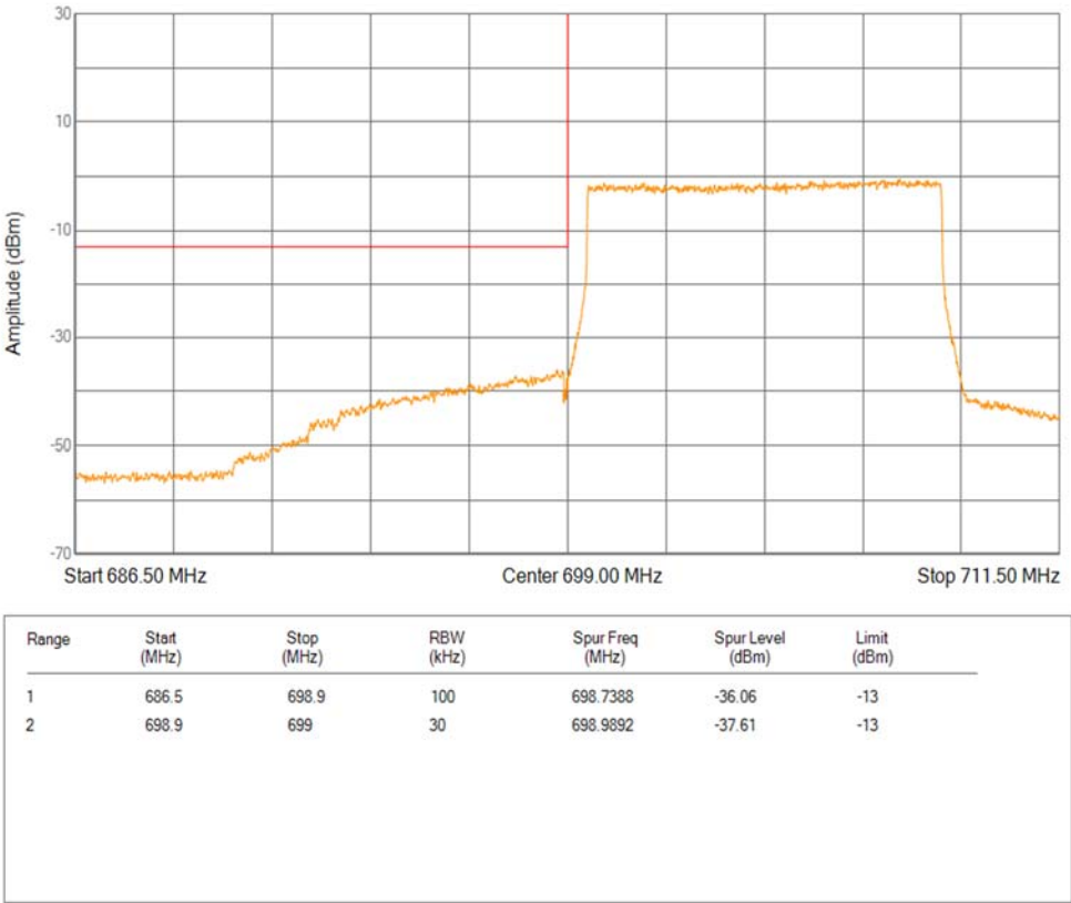
Band12 QPSK BW=10MHz Channel=23060 RB Size=50 Position=#0 Extended
