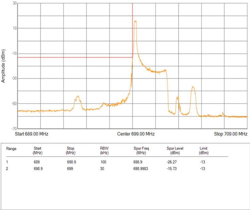
Band12 QPSK BW=3MHz Channel=23025 RB Size=1 Position=#0 Extended
