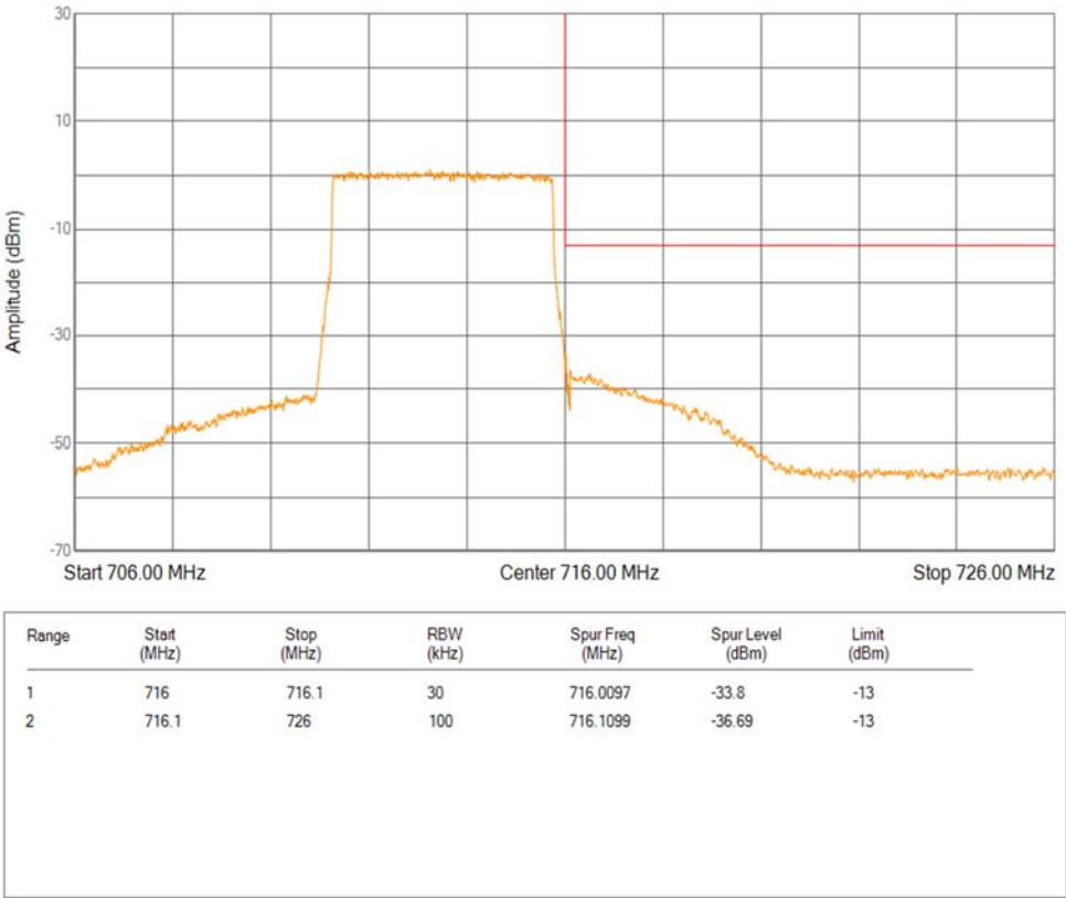
Band12 16QAM BW=5MHz Channel=23155 RB Size=25 Position=#0 Extended
