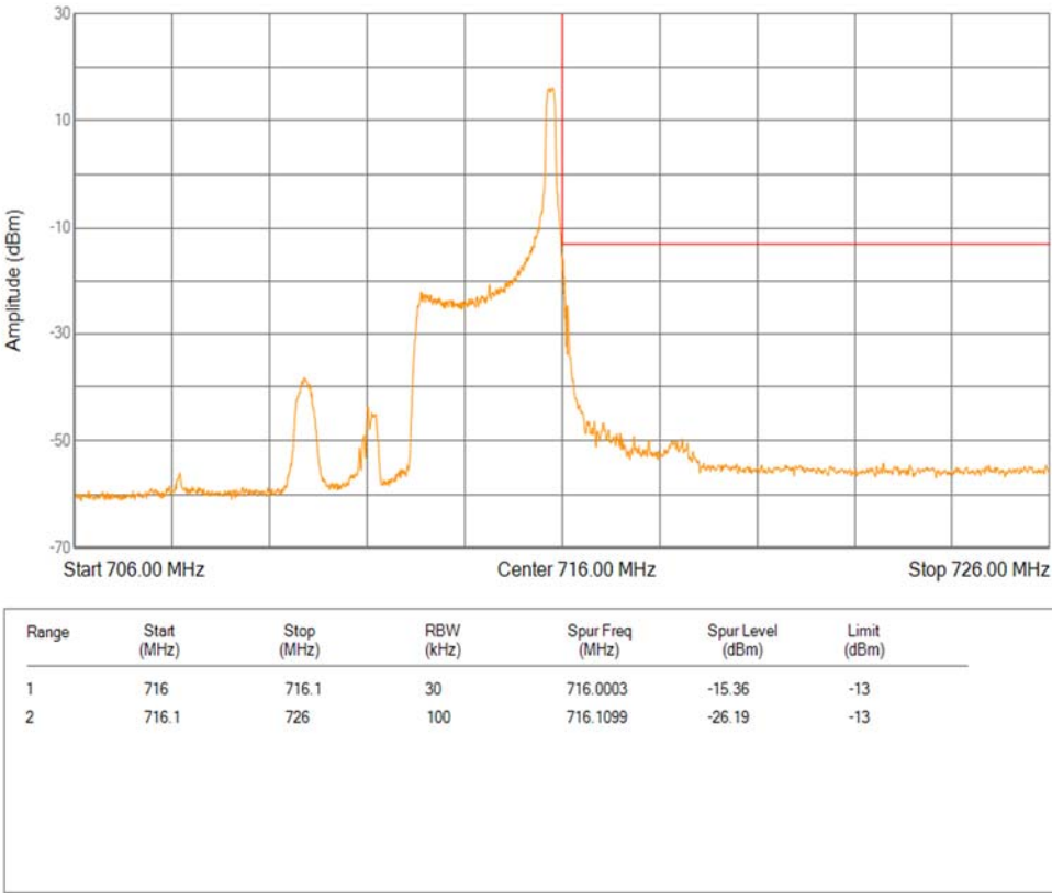
Band12 QPSK BW=3MHz Channel=23165 RB Size=1 Position=#Max Extended
