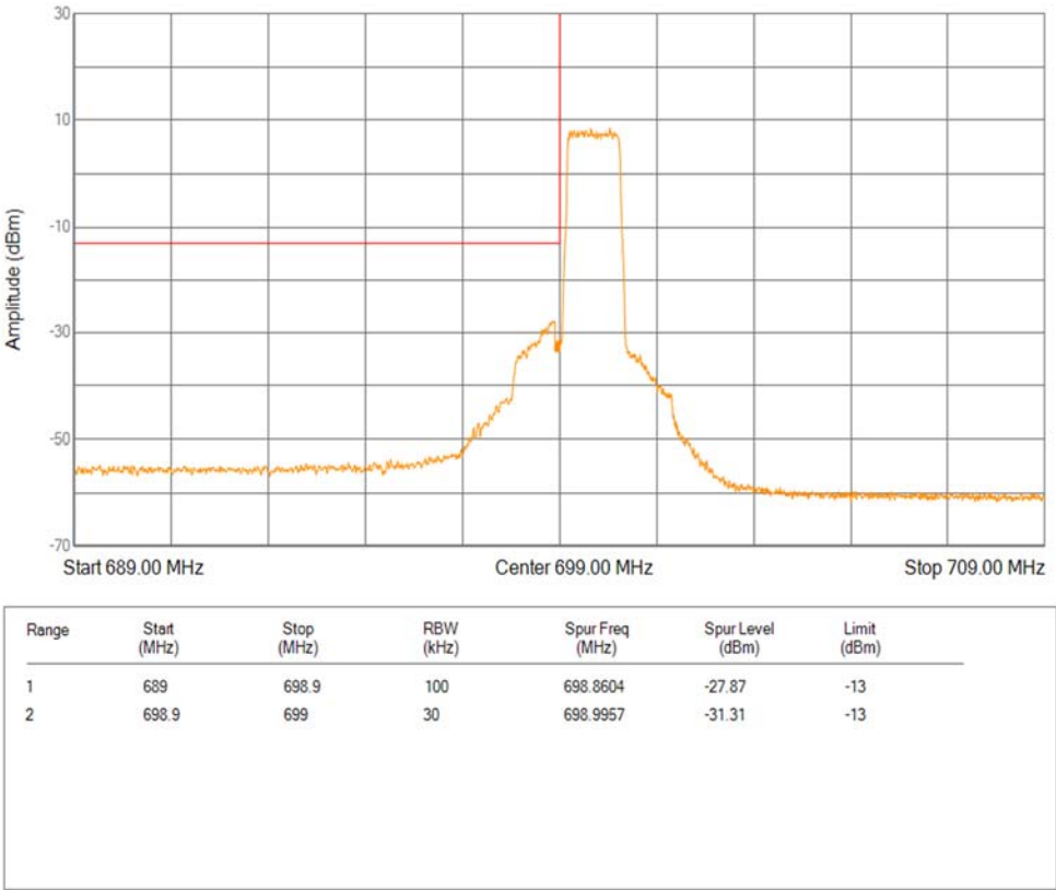
Band12 QPSK BW=1.4MHz Channel=23017 RB Size=6 Position=#0 Extended
