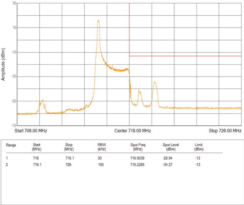
Band12 QPSK BW=3MHz Channel=23165 RB Size=1 Position=#0 Extended
