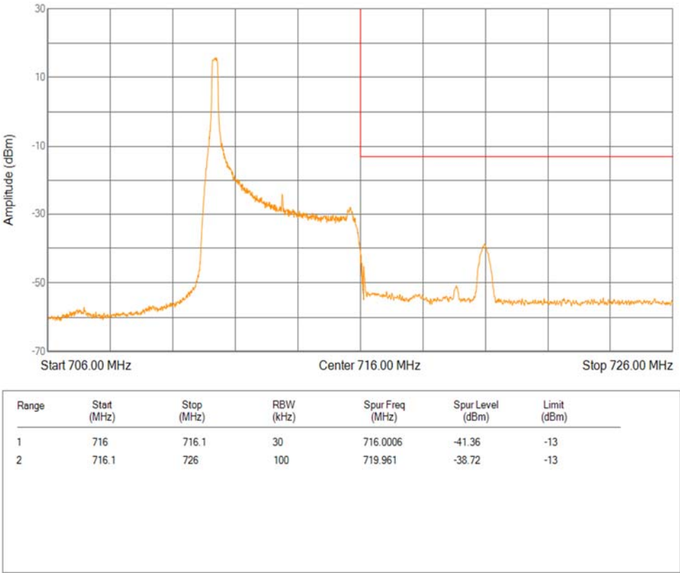
Band12 QPSK BW=5MHz Channel=23155 RB Size=1 Position=#0 Extended
