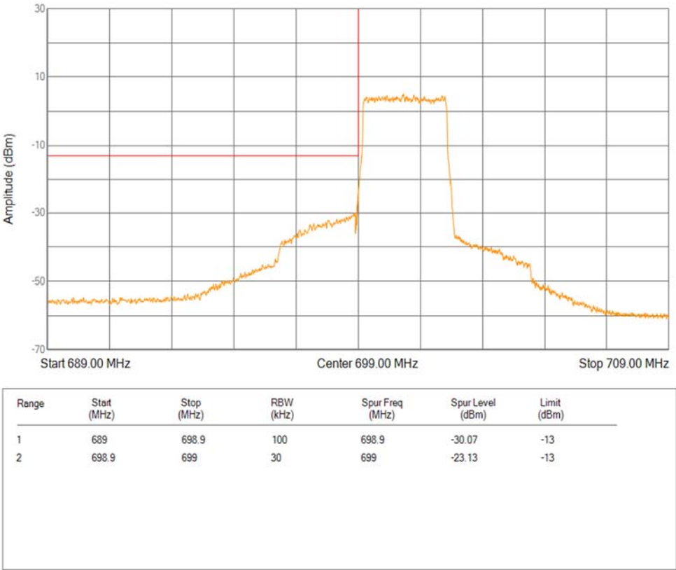
Band12 QPSK BW=3MHz Channel=23025 RB Size=15 Position=#0 Extended
