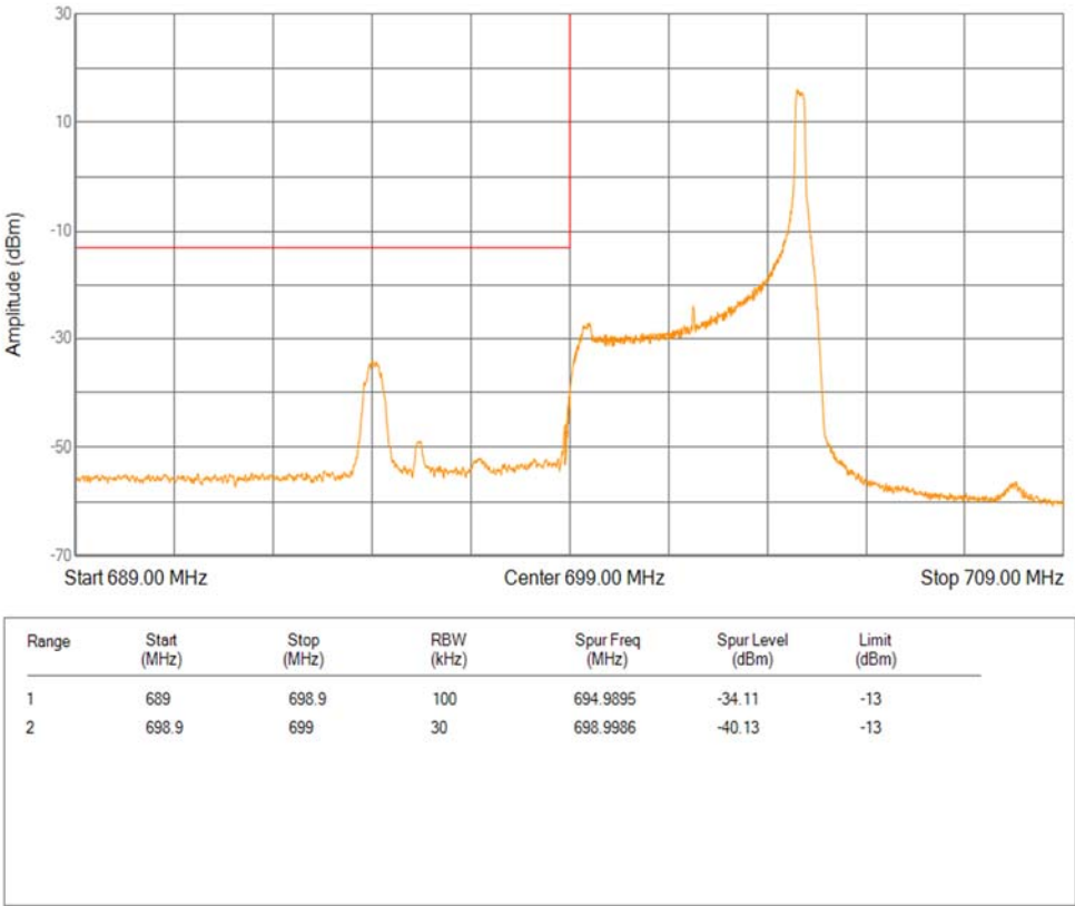
Band12 QPSK BW=5MHz Channel=23035 RB Size=1 Position=#Max Extended
