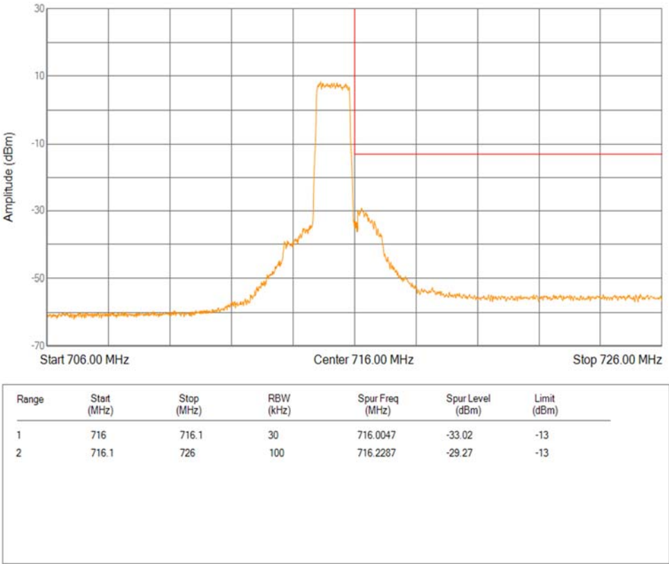
Band12 QPSK BW=1.4MHz Channel=23173 RB Size=6 Position=#0 Extended
