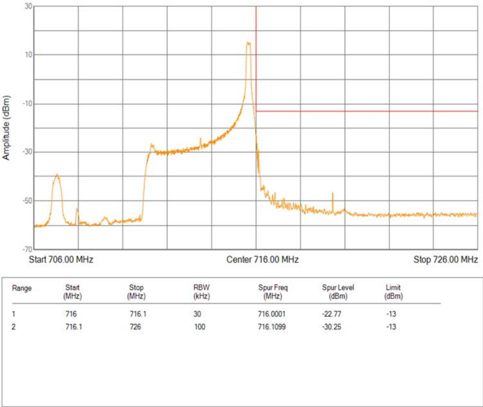
Band12 16QAM BW=5MHz Channel=23155 RB Size=1 Position=#Max Extended
