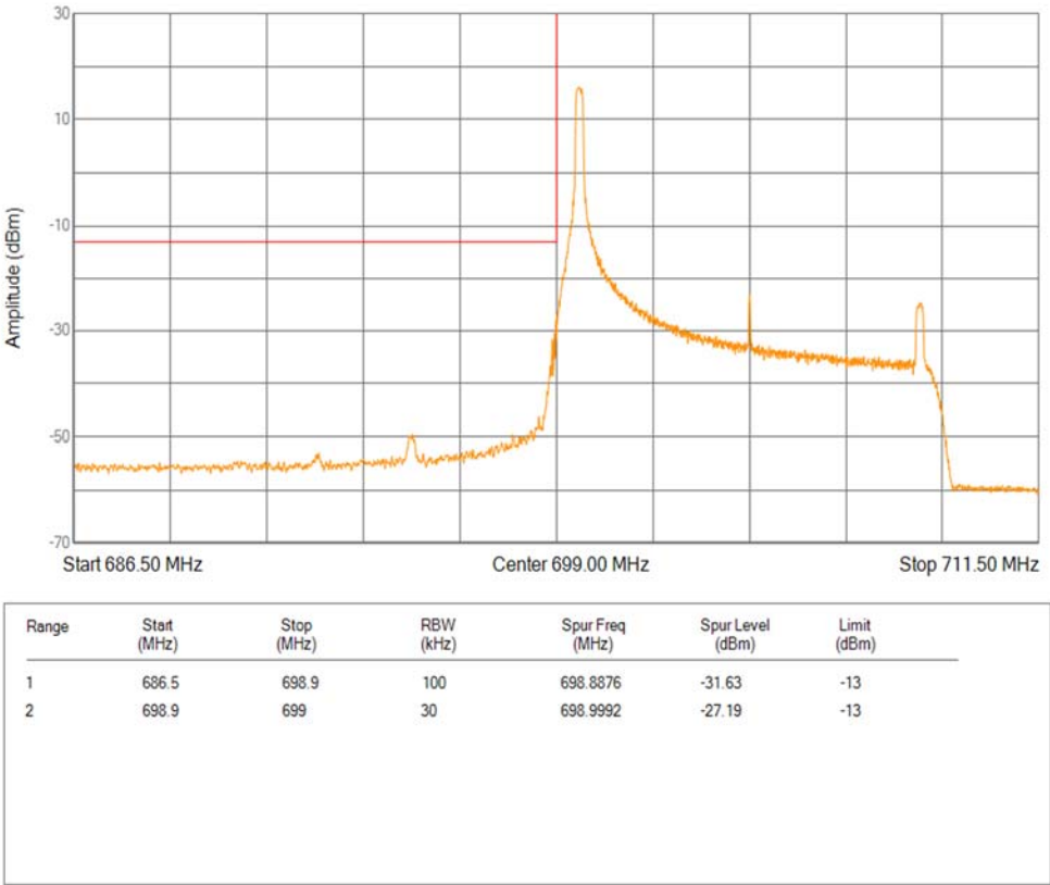
Band12 QPSK BW=10MHz Channel=23060 RB Size=1 Position=#0 Extended
