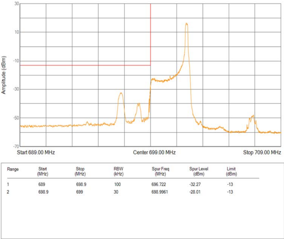
Band12 QPSK BW=3MHz Channel=23025 RB Size=1 Position=#Max Extended
