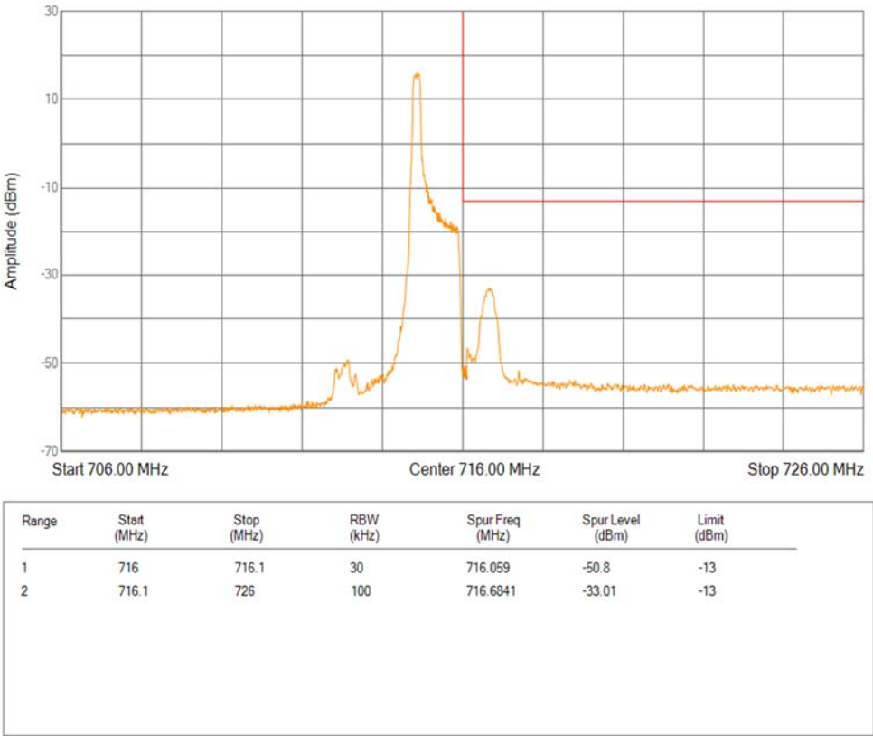
Band12 QPSK BW=1.4MHz Channel=23173 RB Size=1 Position=#0 Extended
