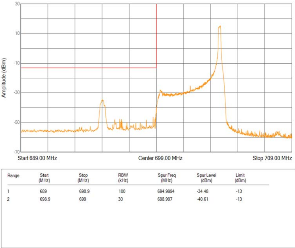
Band12 16QAM BW=5MHz Channel=23035 RB Size=1 Position=#Max Extended
