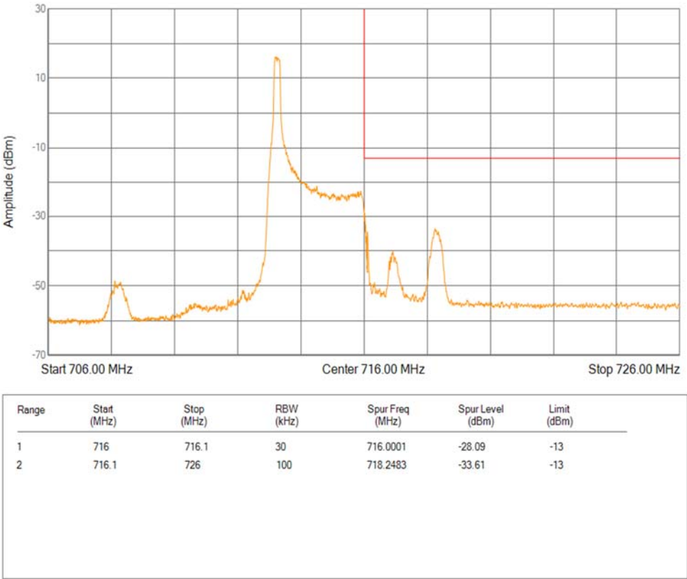
Band12 16QAM BW=3MHz Channel=23165 RB Size=1 Position=#0 Extended
