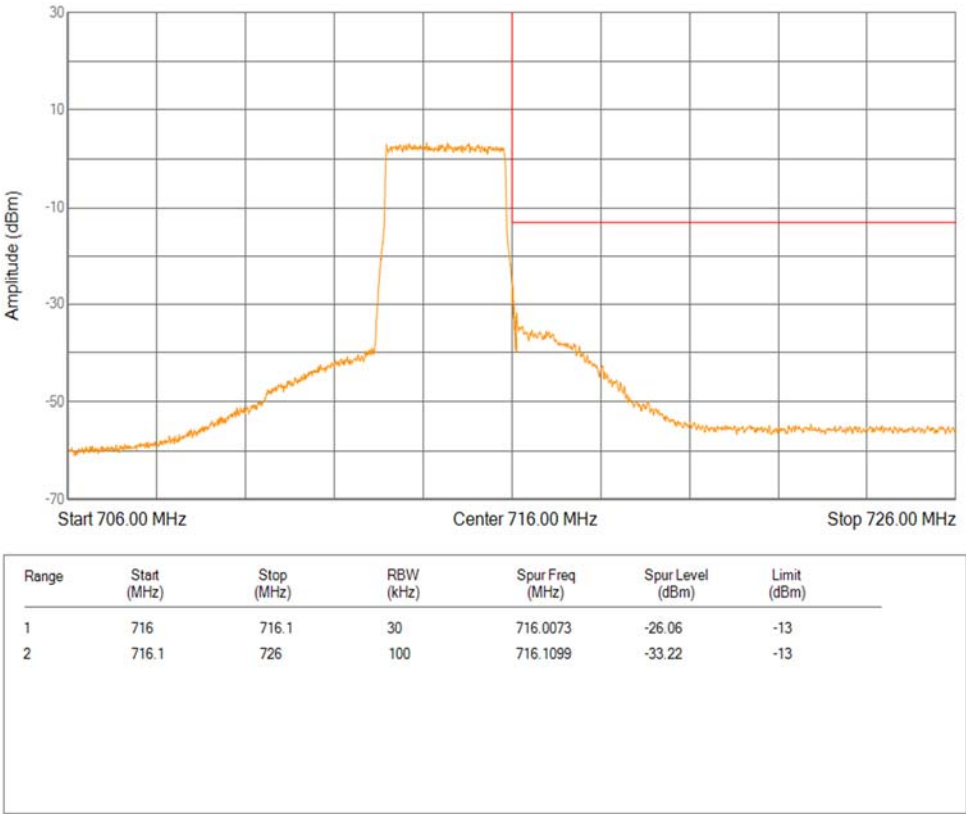
Band12 16QAM BW=3MHz Channel=23165 RB Size=15 Position=#0 Extended
