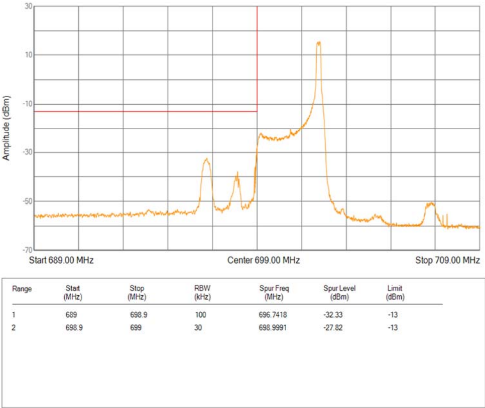
Band12 16QAM BW=3MHz Channel=23025 RB Size=1 Position=#Max Extended
