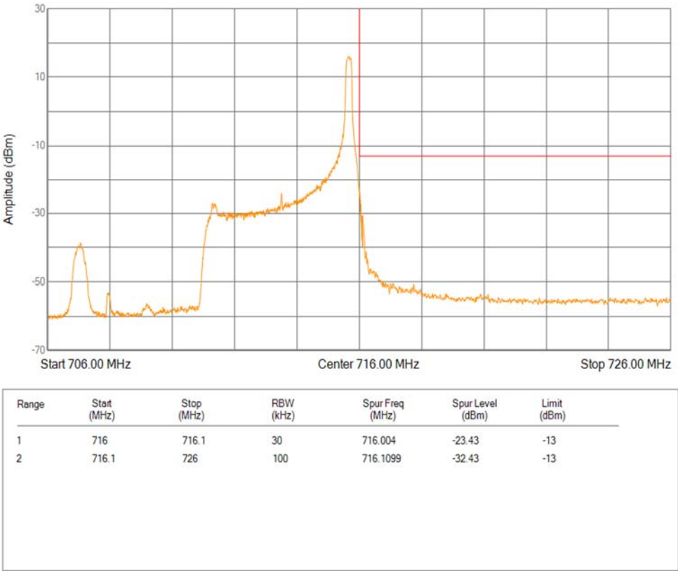
Band12 QPSK BW=5MHz Channel=23155 RB Size=1 Position=#Max Extended
