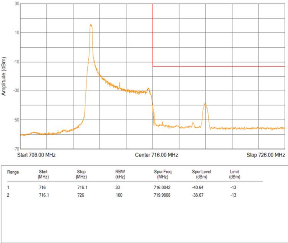
Band12 16QAM BW=5MHz Channel=23155 RB Size=1 Position=#0 Extended
