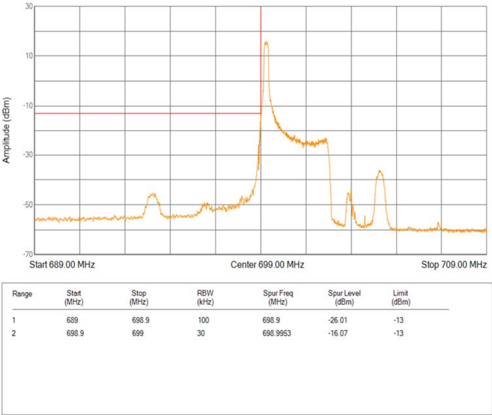
Band12 16QAM BW=3MHz Channel=23025 RB Size=1 Position=#0 Extended
