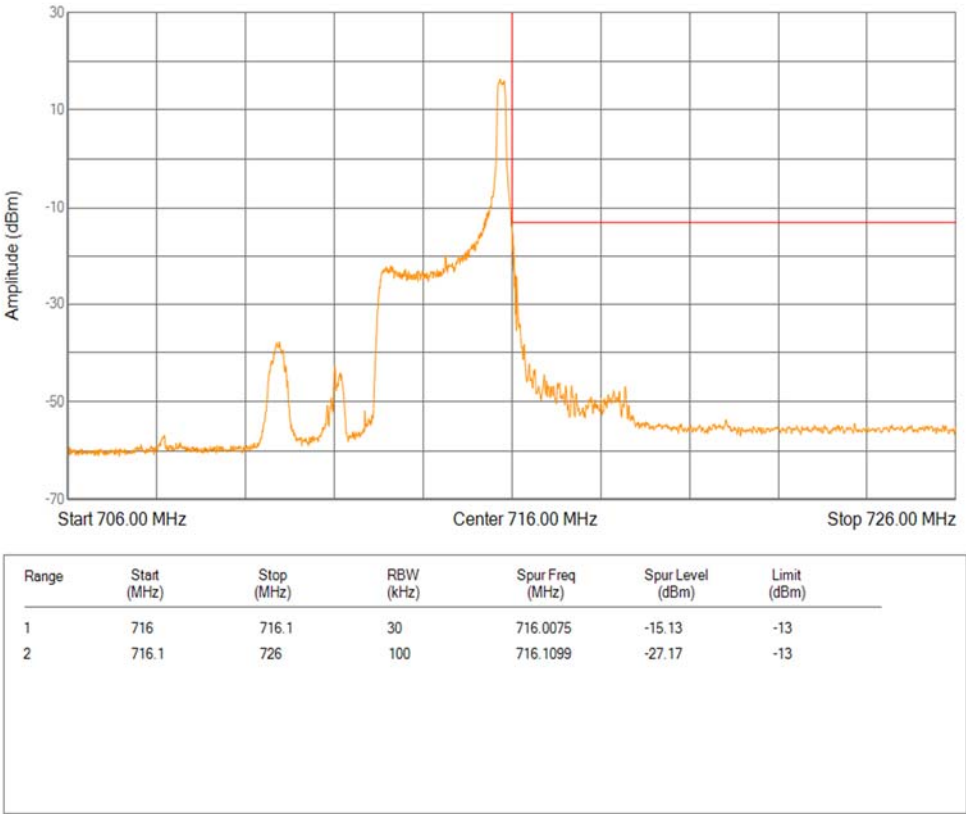
Band12 16QAM BW=3MHz Channel=23165 RB Size=1 Position=#Max Extended
