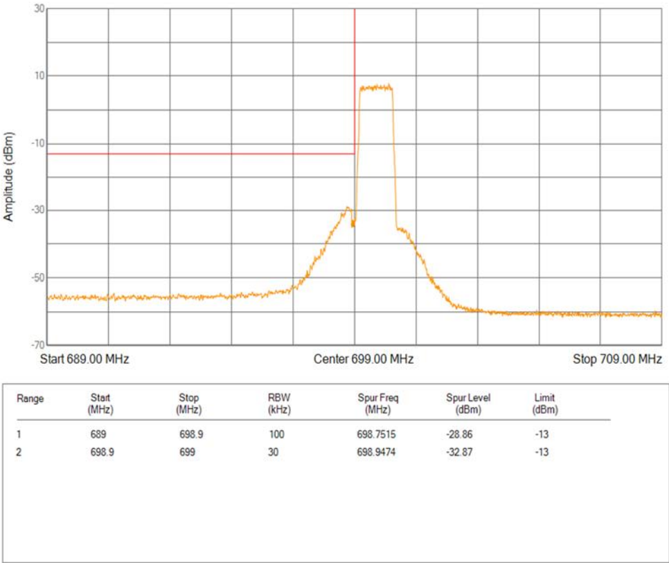
Band12 16QAM BW=1.4MHz Channel=23017 RB Size=6 Position=#0 Extended
