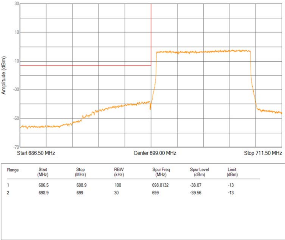
Band12 16QAM BW=10MHz Channel=23060 RB Size=50 Position=#0 Extended
