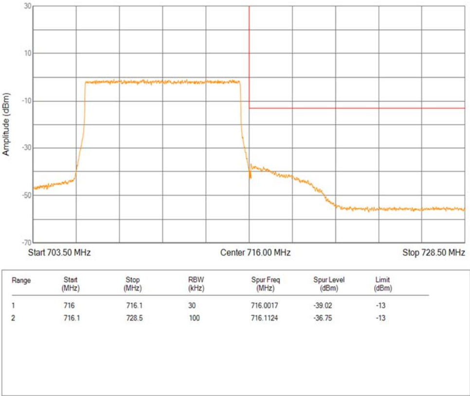
Band12 QPSK BW=10MHz Channel=23130 RB Size=50 Position=#0 Extended
