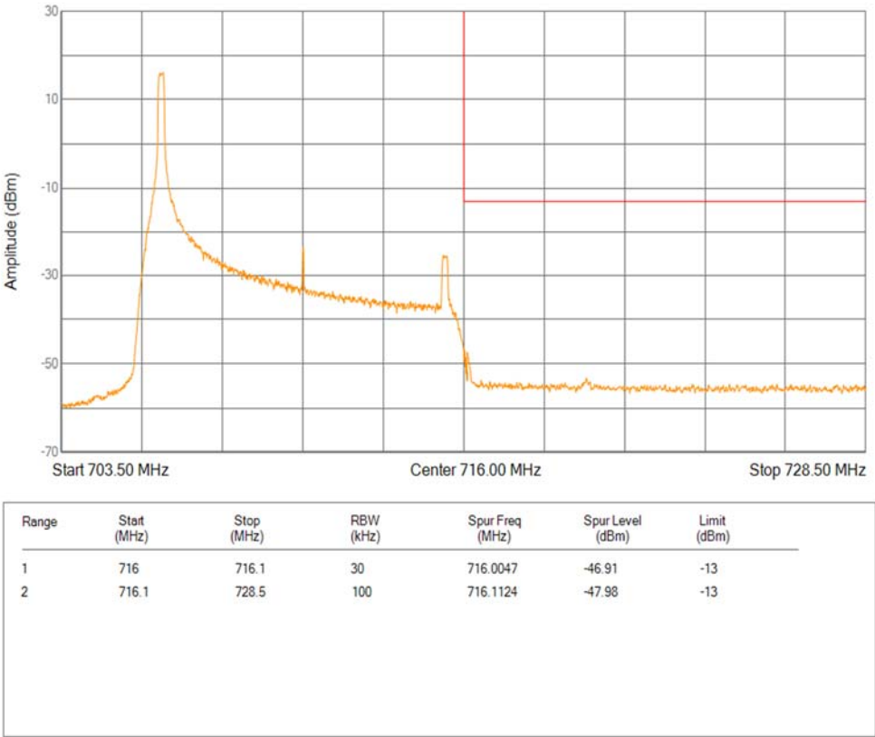
Band12 QPSK BW=10MHz Channel=23130 RB Size=1 Position=#0 Extended
