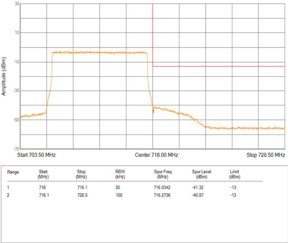
Band12 16QAM BW=10MHz Channel=23130 RB Size=50 Position=#0 Extended
