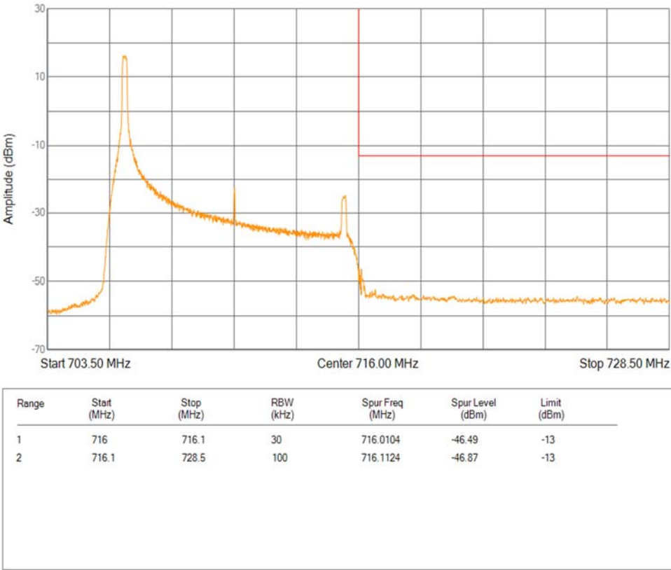
Band12 16QAM BW=10MHz Channel=23130 RB Size=1 Position=#0 Extended
