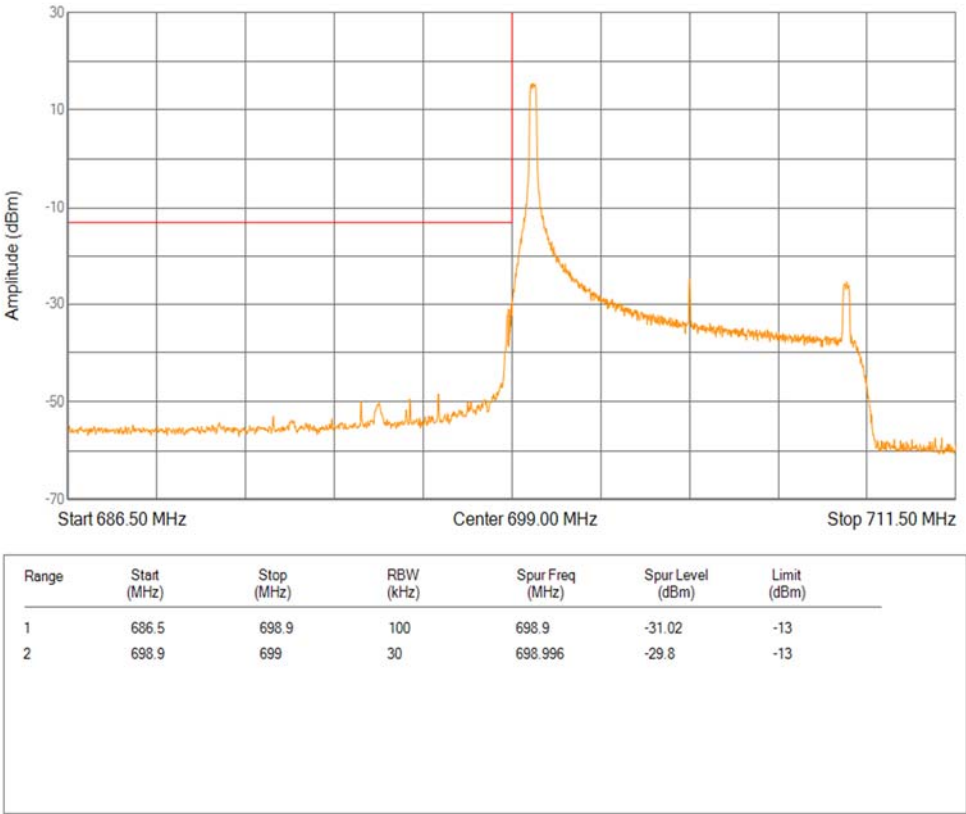
Band12 16QAM BW=10MHz Channel=23060 RB Size=1 Position=#0 Extended
