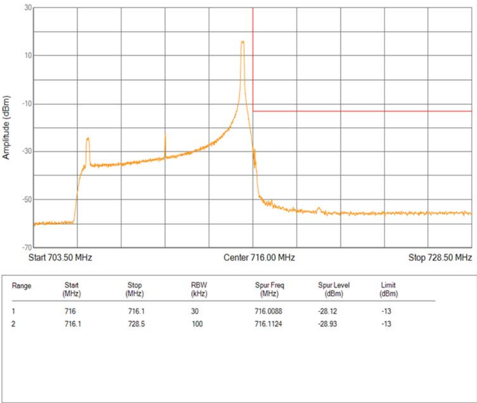
Band12 QPSK BW=10MHz Channel=23130 RB Size=1 Position=#Max Extended
