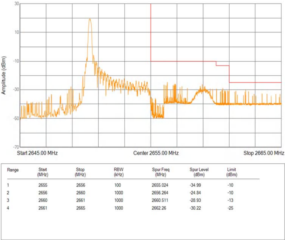
Band41(2535-2655) QPSK BW=5MHz Channel=41215 RB Size=1 Position=#0 Extended
