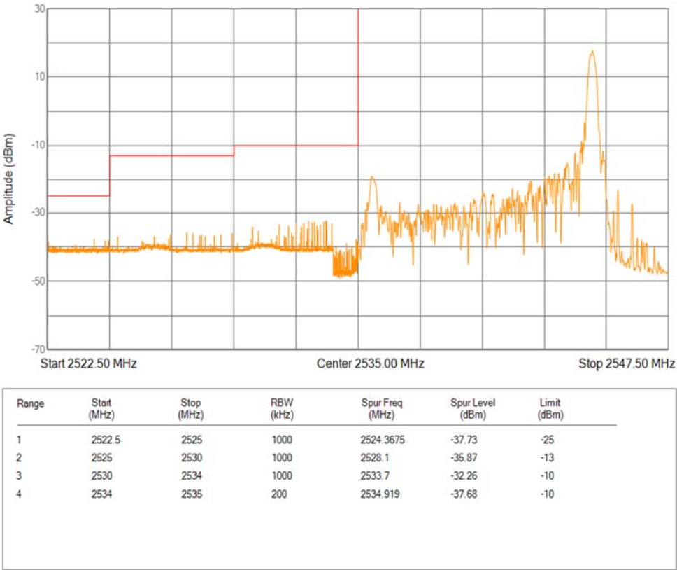
Band41(2535-2655) QPSK BW=10MHz Channel=40090 RB Size=1 Position=#Max Extended
