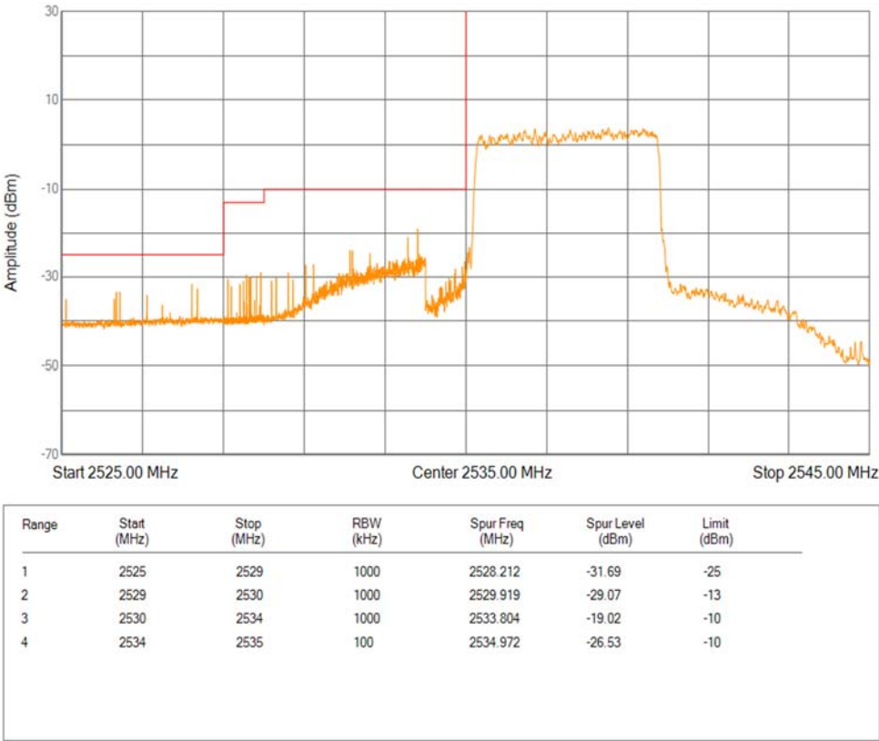
Band41(2535-2655) QPSK BW=5MHz Channel=40065 RB Size=25 Position=#0 Extended
