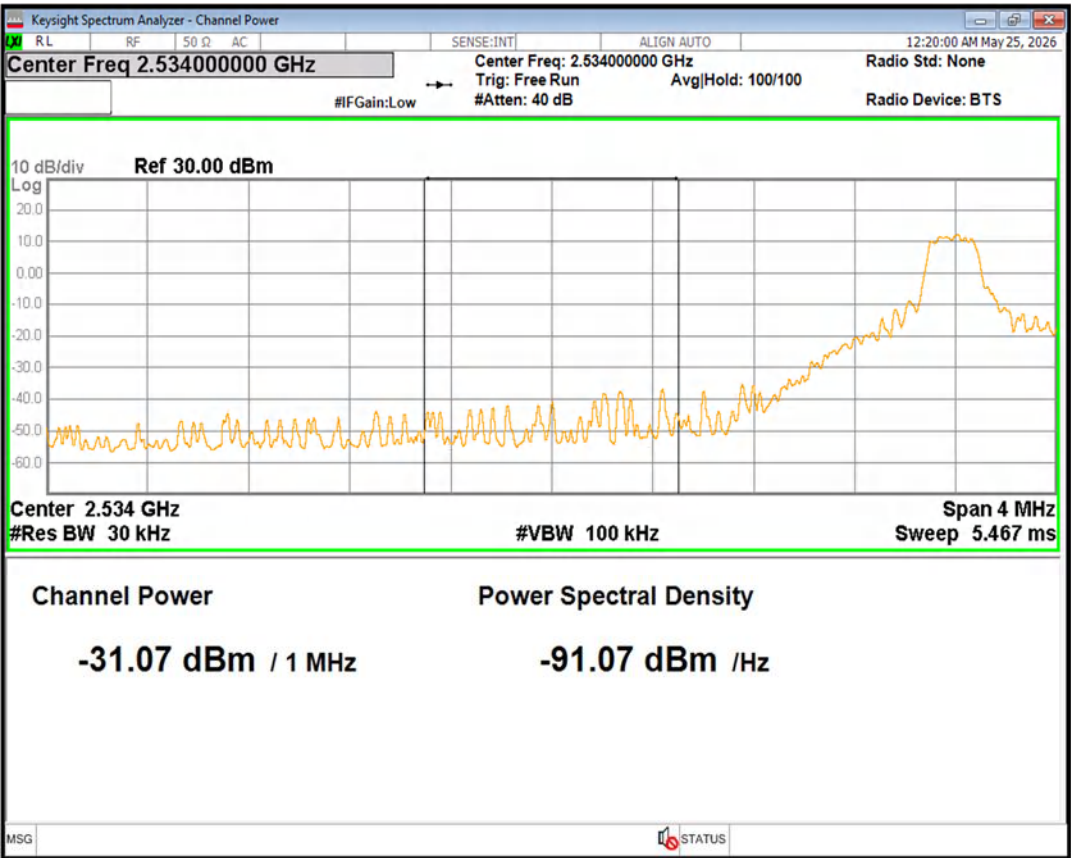
Band41(2535-2655) QPSK BW=10MHz Channel=40090 RB Size=1 Position=#Max Normal
