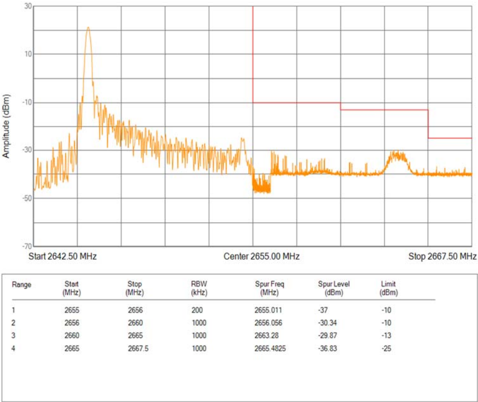
Band41(2535-2655) 16QAM BW=10MHz Channel=41190 RB Size=1 Position=#0 Extended
