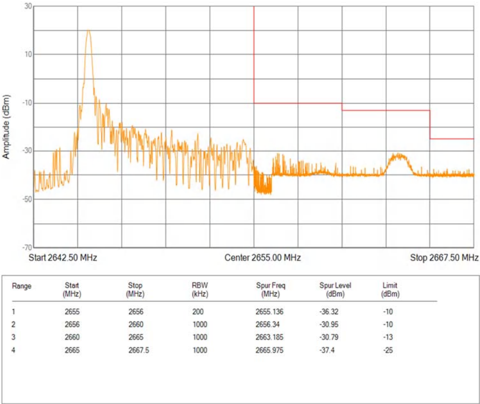
Band41(2535-2655) QPSK BW=10MHz Channel=41190 RB Size=1 Position=#0 Extended
