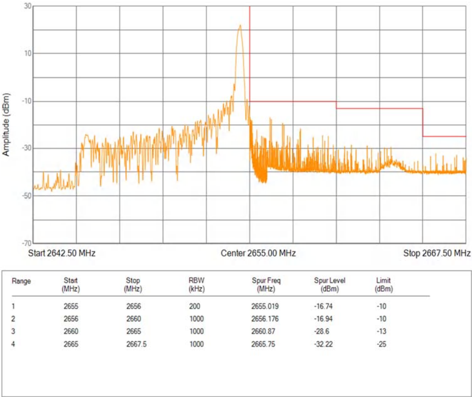
Band41(2535-2655) 16QAM BW=10MHz Channel=41190 RB Size=1 Position=#Max Extended
