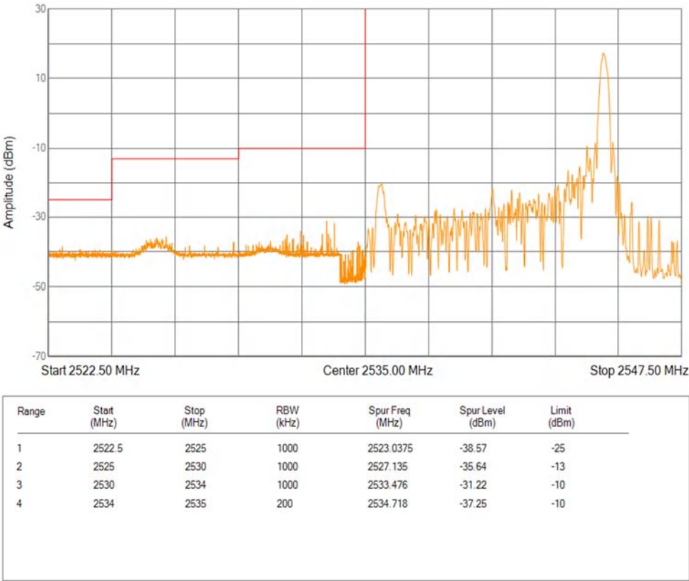
Band41(2535-2655) 16QAM BW=10MHz Channel=40090 RB Size=1 Position=#Max Extended
