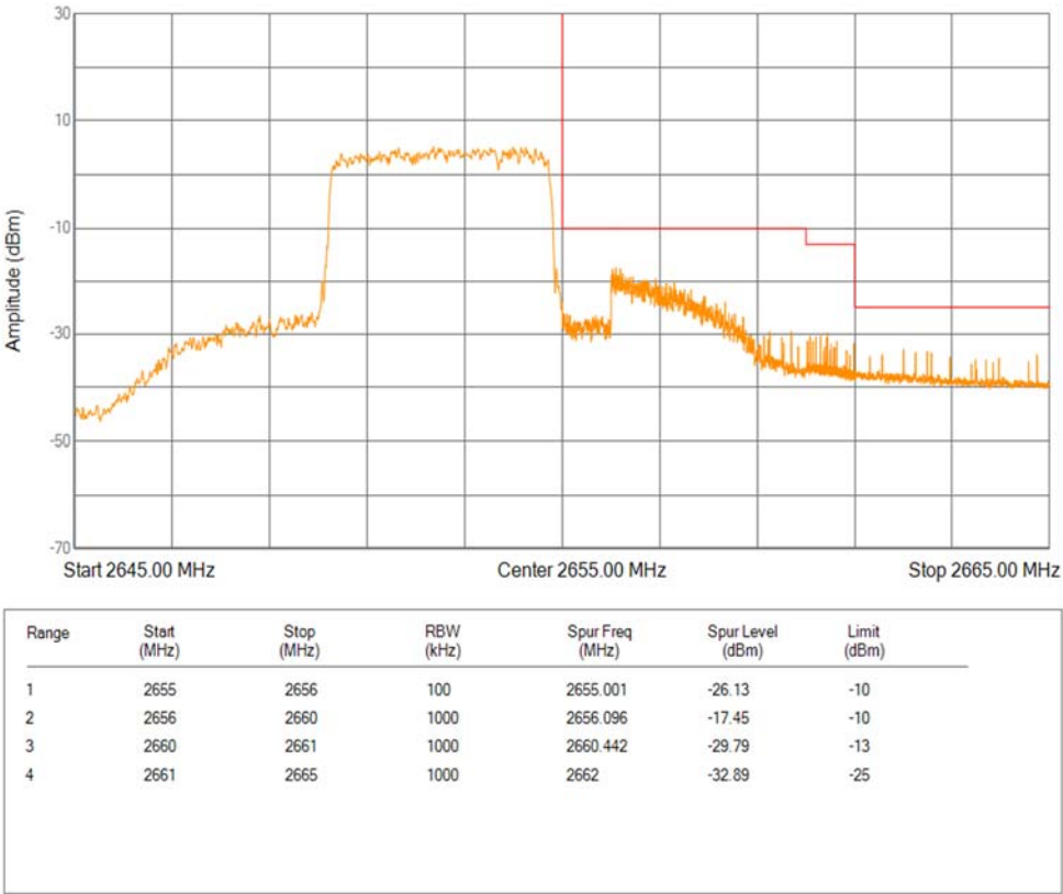
Band41(2535-2655) 16QAM BW=5MHz Channel=41215 RB Size=25 Position=#0 Extended
