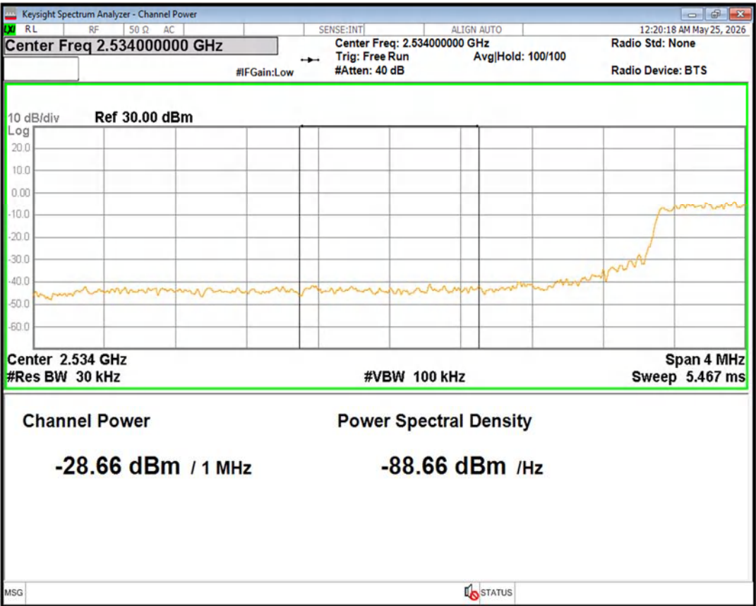
Band41(2535-2655) 16QAM BW=10MHz Channel=40090 RB Size=1 Position=#0 Normal
