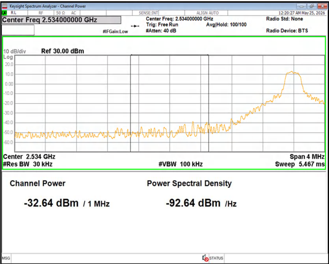
Band41(2535-2655) 16QAM BW=10MHz Channel=40090 RB Size=1 Position=#Max Normal
