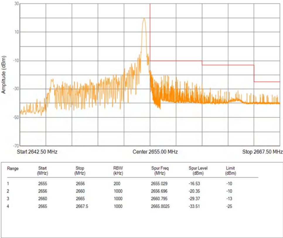
Band41(2535-2655) QPSK BW=10MHz Channel=41190 RB Size=1 Position=#Max Extended
