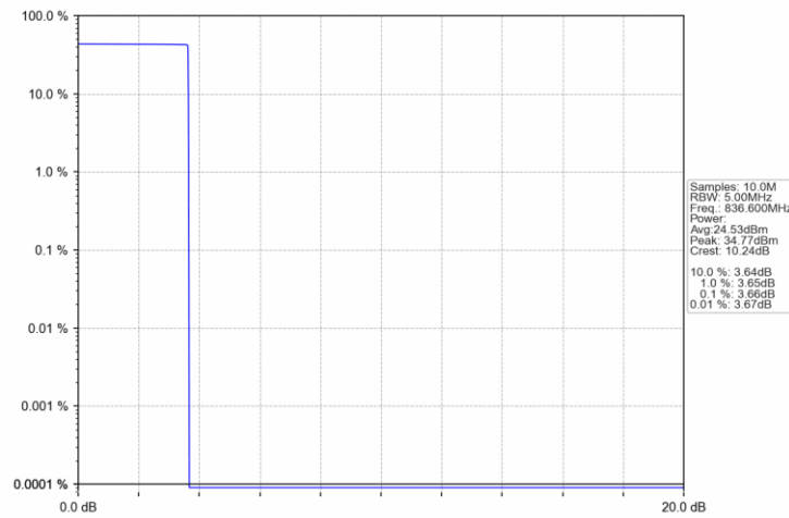
GSM850_GPRS_MCH_836.6MHz_4 TX Slots_NTNV
