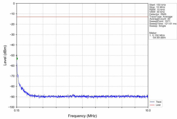
Band17_10MHz_16QAM_HCH_711MHz_RB_1_0_NTNV
