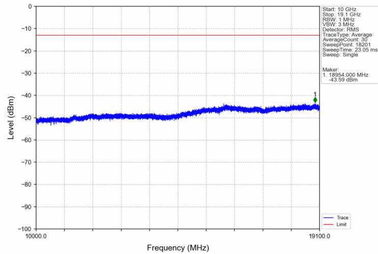
Band2_5MHz_QPSK_HCH_1907.5MHz_RB_1_24_NTNV
