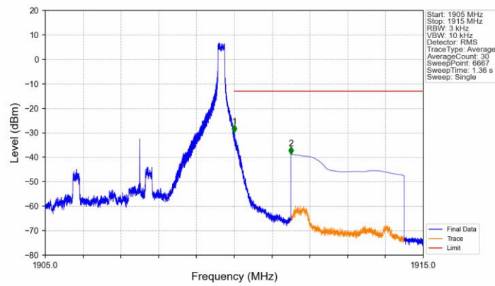
Band2_5MHz_QPSK_HCH_1907.5MHz_RB_1_24_NTNV
