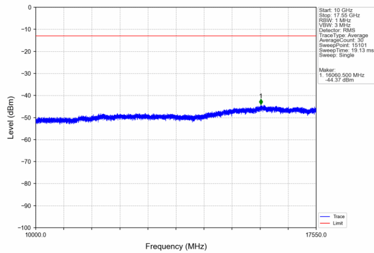
Band4_1.4MHz_QPSK_LCH_1710.7MHz_RB_1_0_NTNV
