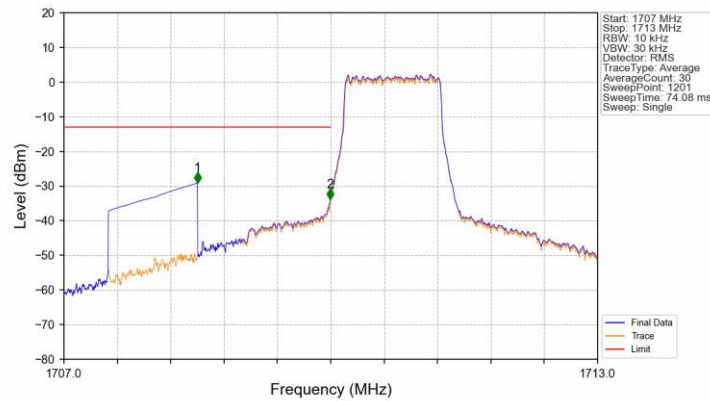
Band66_1.4MHz_16QAM_LCH_1710.7MHz_RB_6_0_NTNV
