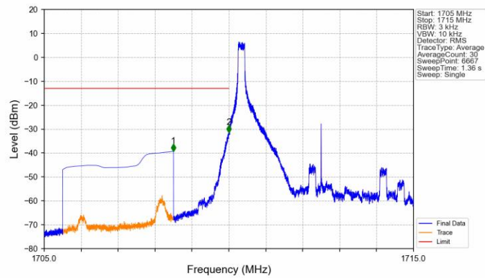
Band66_5MHz_QPSK_LCH_1712.5MHz_RB_1_0_NTNV
