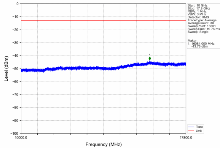
Band66_1.4MHz_16QAM_LCH_1710.7MHz_RB_6_0_NTNV
