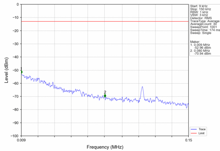
Band66_1.4MHz_16QAM_HCH_1779.3MHz_RB_1_0_NTNV
