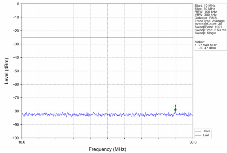
Band7_15MHz_16QAM_MCH_2535MHz_RB_1_0_NTNV
