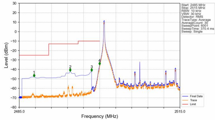
Band7_15MHz_QPSK_LCH_2507.5MHz_RB_1_0_NTNV
