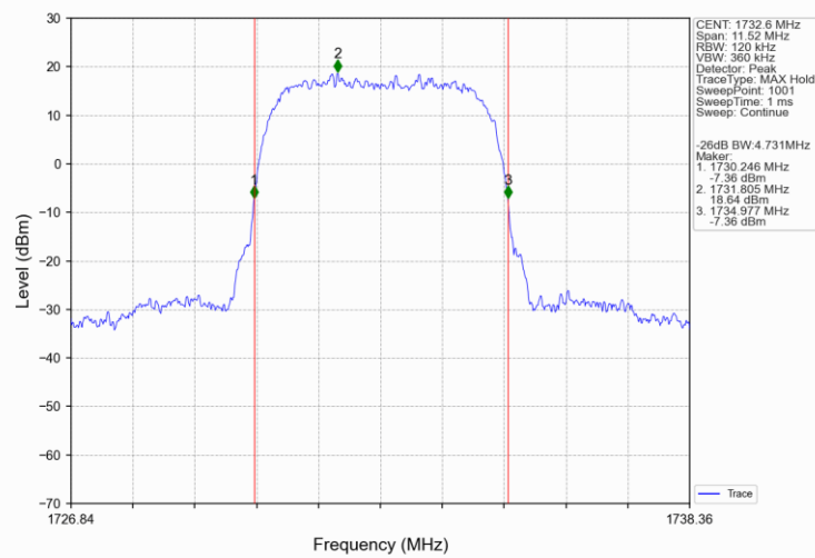
Band4_RMC_MCH_1732.6MHz_12.2kbps RMC_NTNV
