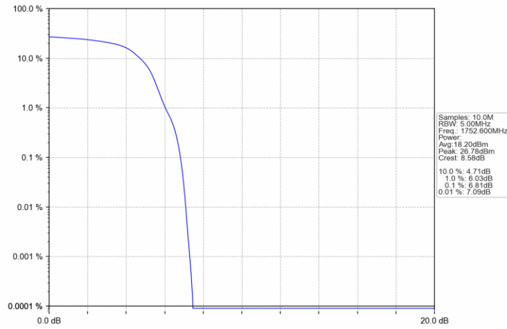
Band4_HSUPA_HCH_1752.6MHz_Subtest 1_NTNV
