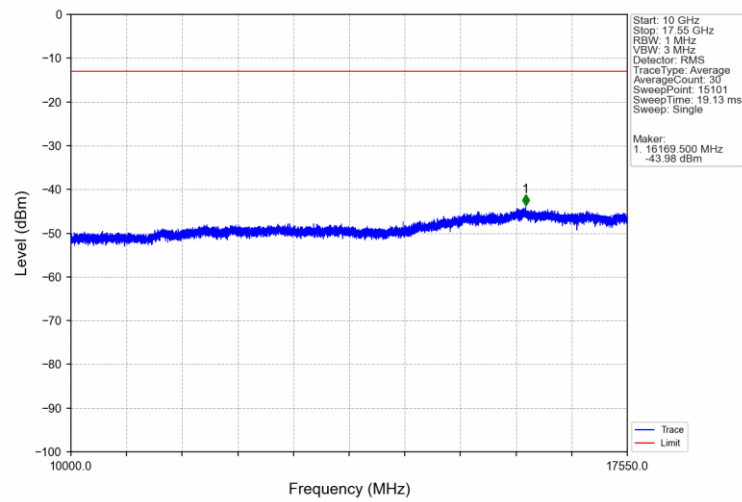
Band4_HSDPA_MCH_1732.6MHz_Subtest 1_NTNV
