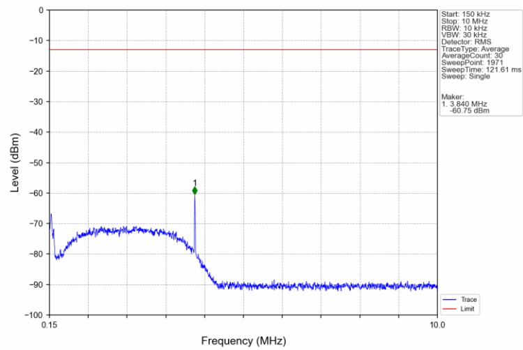
Band5_RMC_HCH_846.6MHz_12.2kbps RMC_NTNV
