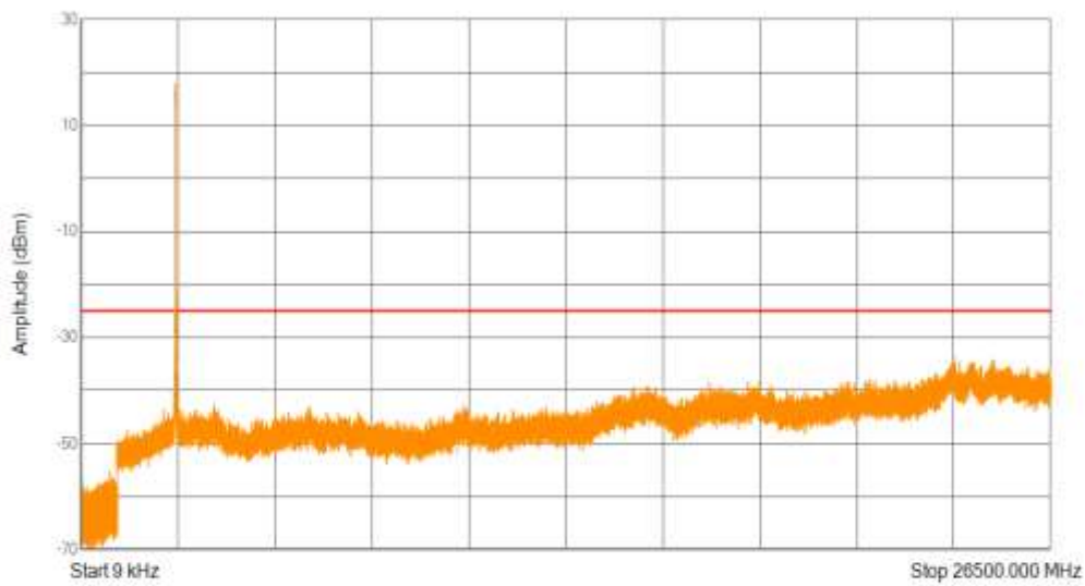
Band41(2535-2655) QPSK BW=10MHz Channel=40640 RB Size=50 Position=#0
