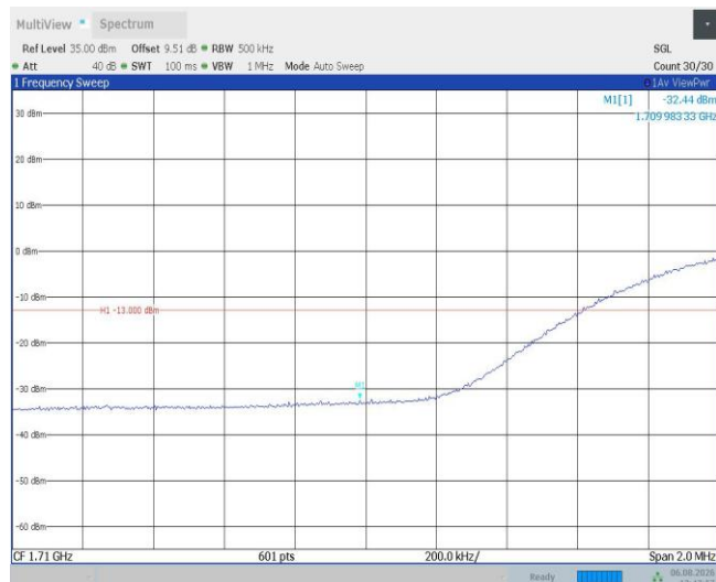
Band66-20MHz-16QAM-132572-1RB#0
