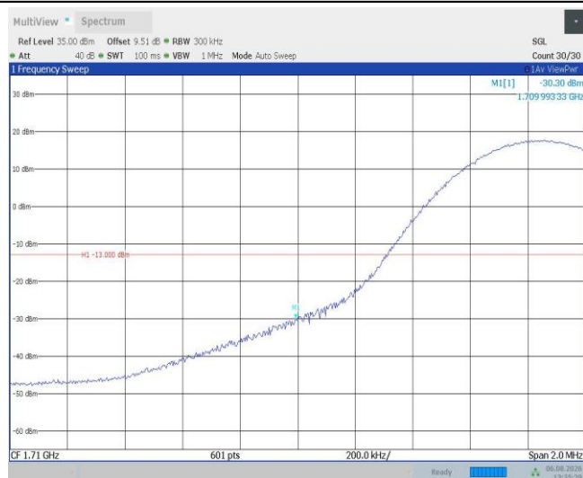
Band66-15MHz-16QAM-132047-1RB#74
