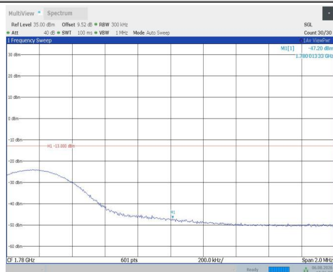
Band66-15MHz-QPSK-132597-1RB#74
