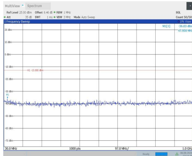
Band66-5MHz-16QAM-131997-1RB#0-Range2:1000~10000MHz
