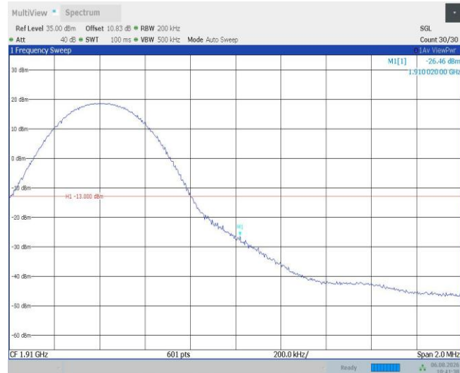
Band2-10MHz-QPSK-19150-50RB#0
