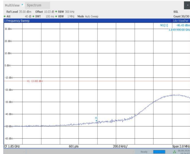
Band2-15MHz-16QAM-18675-75RB#0
