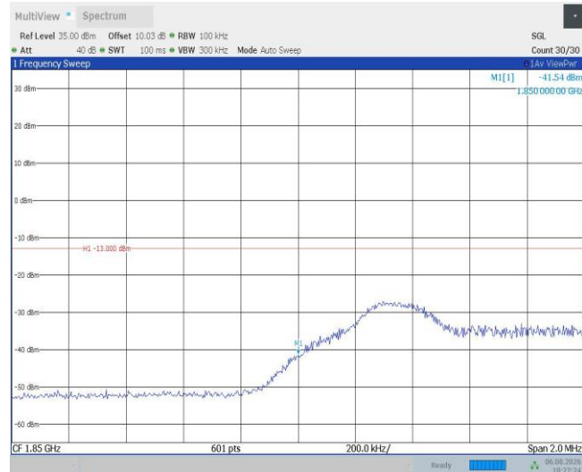
Band2-5MHz-16QAM-18625-25RB#0
