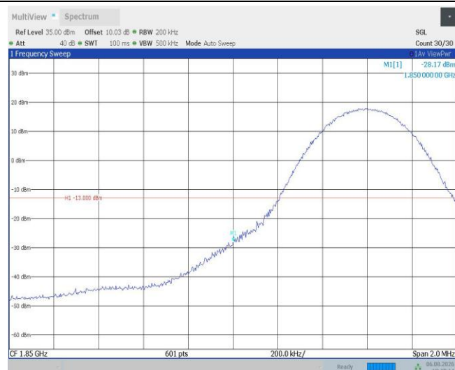
Band2-10MHz-16QAM-18650-1RB#49
