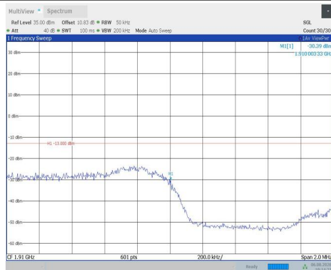
Band2-3MHz-16QAM-19185-1RB#14
