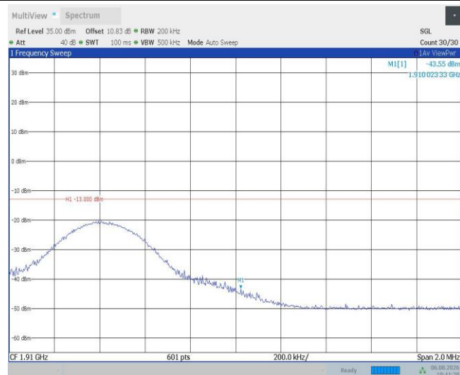
Band2-10MHz-16QAM-19150-1RB#49
