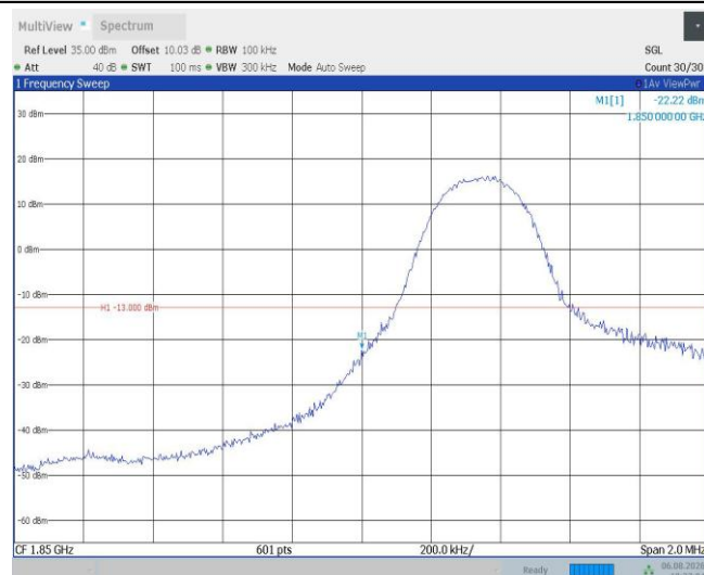
Band2-5MHz-16QAM-18625-1RB#24
