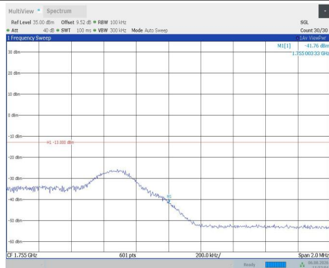
Band4-5MHz-QPSK-20375-1RB#24
