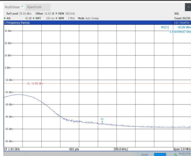
Band2-15MHz-QPSK-19125-1RB#74
