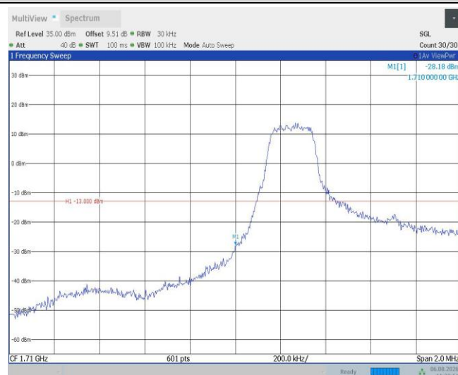
Band4-1.4MHz-16QAM-19957-1RB#5
