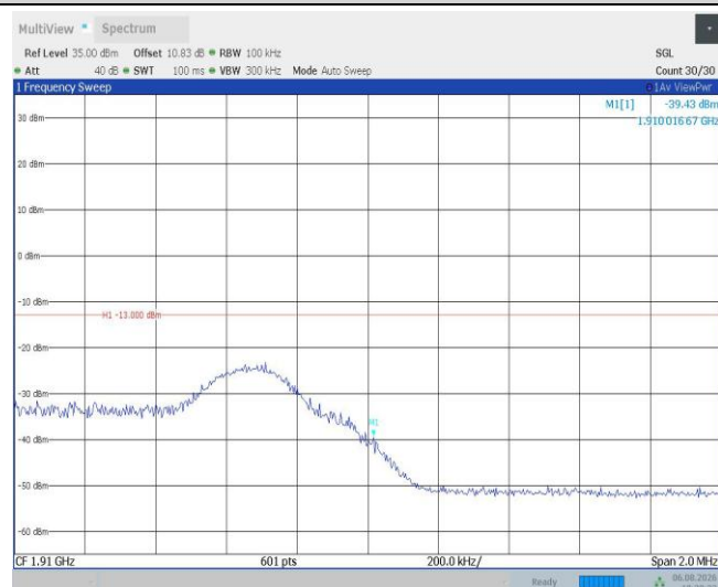
Band2-5MHz-16QAM-19175-1RB#24
