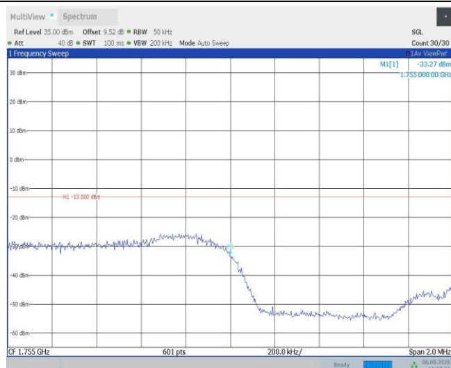
Band4-3MHz-QPSK-20385-1RB#14
