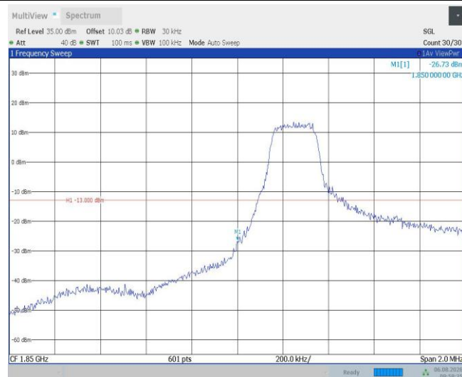
Band2-1.4MHz-16QAM-18607-1RB#5
