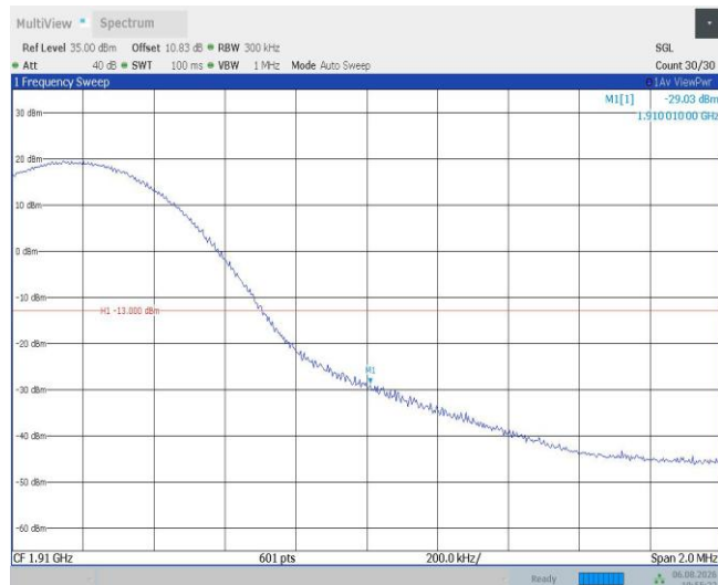
Band2-15MHz-16QAM-19125-75RB#0
