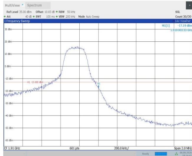
Band2-3MHz-16QAM-19185-15RB#0
