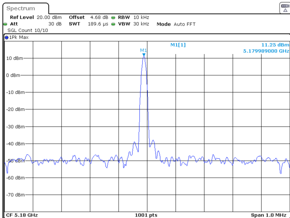
Freq. Stability 0C 120V ac20 5180MHz Ant1
