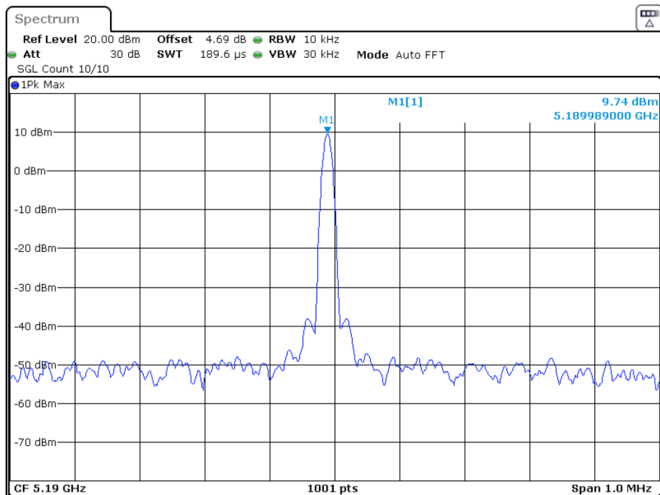
Freq. Stability 40C 120V n40 5190MHz Ant1
