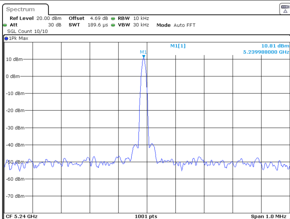
Freq. Stability 0C 120V ac20 5240MHz Ant1
