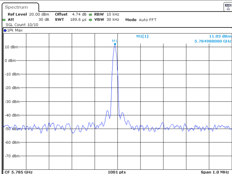
Freq. Stability 40C 120V n20 5785MHz Ant1
