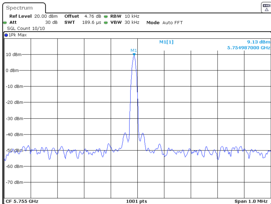
Freq. Stability 40C 120V n40 5755MHz Ant1
