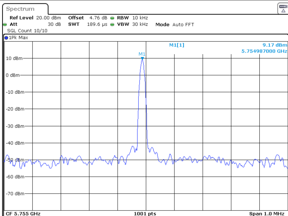
Freq. Stability 0C 120V n40 5755MHz Ant1
