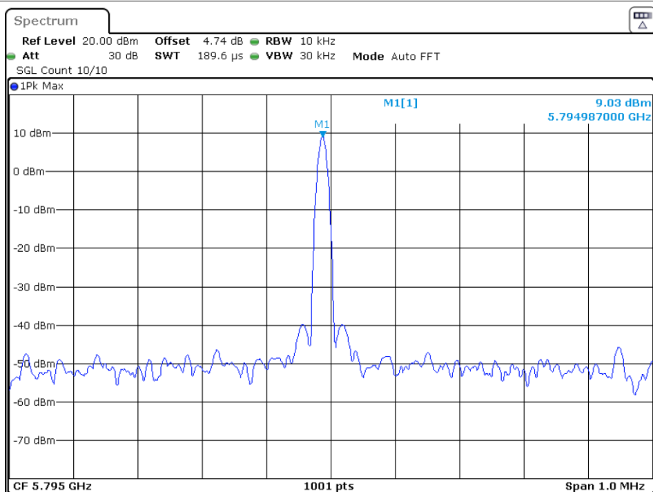
Freq. Stability 10C 120V n40 5795MHz Ant1
