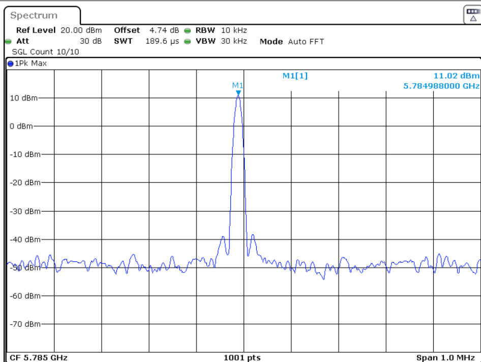
Freq. Stability 0C 120V ac20 5785MHz Ant1
