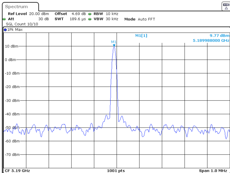
Freq. Stability 0C 120V n40 5190MHz Ant1
