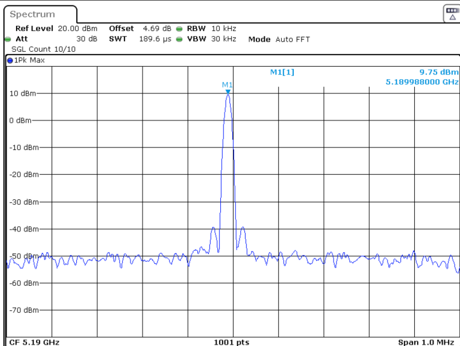
Freq. Stability 20C 120V n40 5190MHz Ant1
