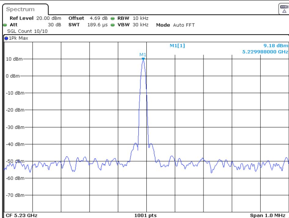
Freq. Stability 10C 120V n40 5230MHz Ant1
