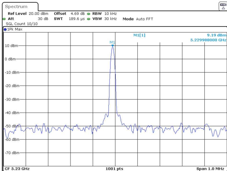
Freq. Stability 30C 120V n40 5230MHz Ant1
