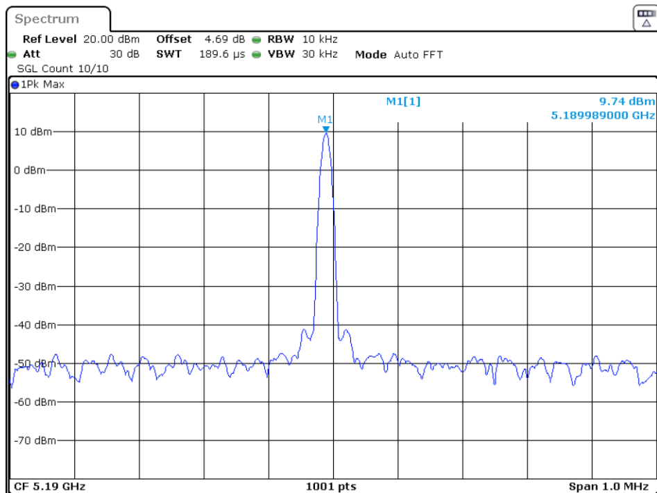
Freq. Stability 0C 120V ac40 5190MHz Ant1
