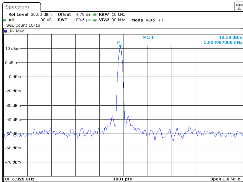
Freq. Stability 10C 120V ac20 5825MHz Ant1
