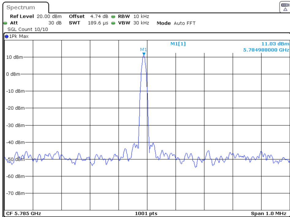
Freq. Stability 40C 120V ac20 5785MHz Ant1
