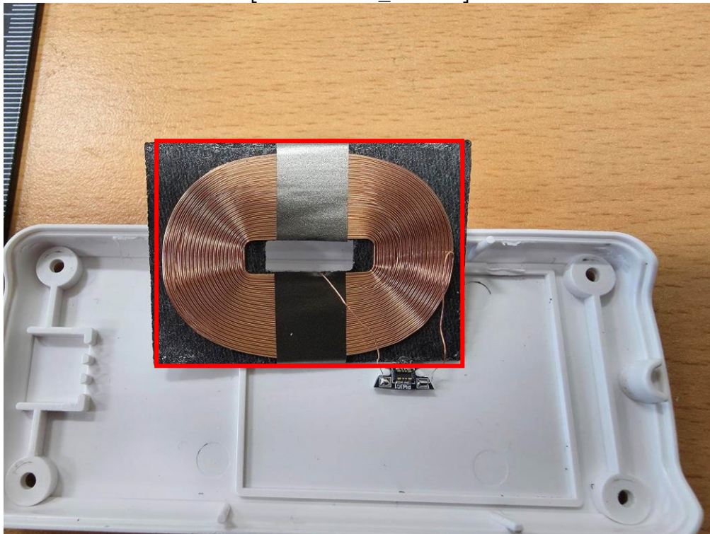
[Coil Antenna_125kHz]
