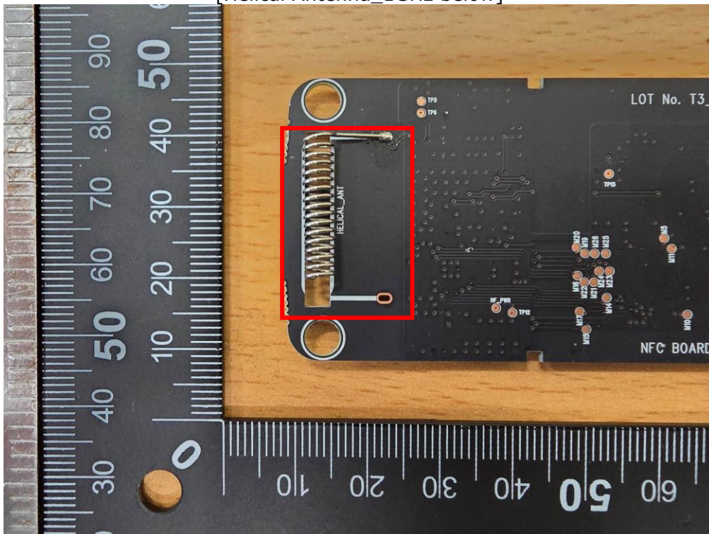
[Helical Antenna_1GHz below]
