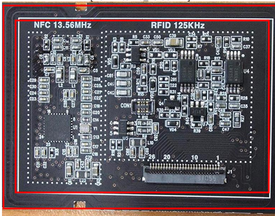
[PCB Antenna_13.56MHz]
