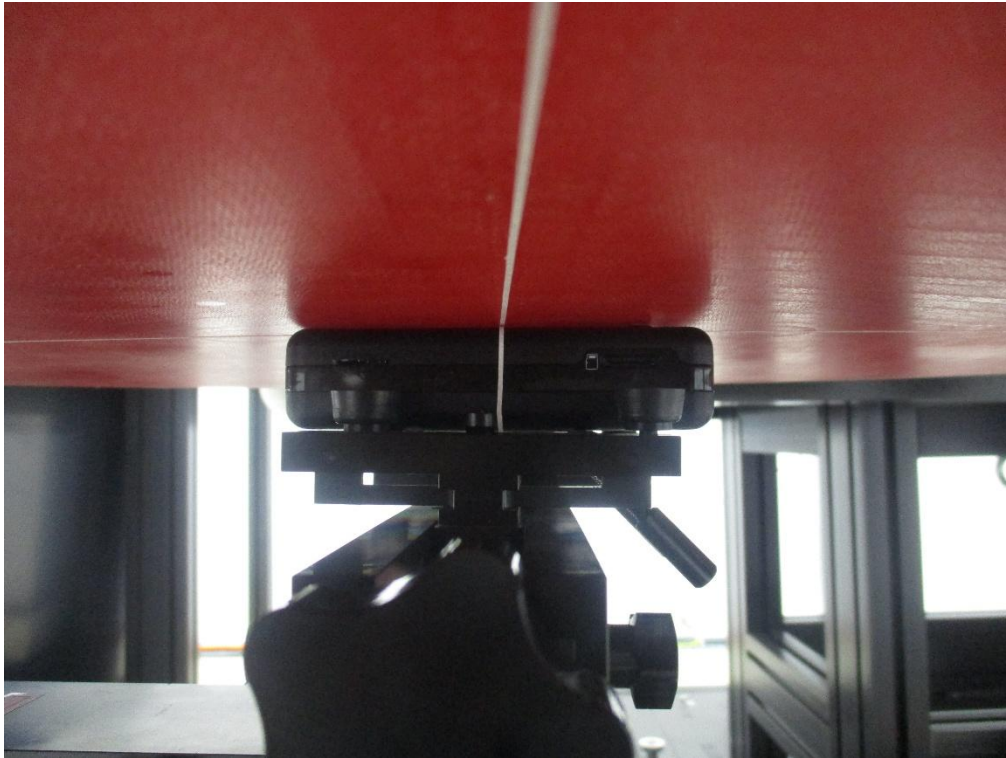
Front Side from Flat Phantom (Separation Distance: 0 cm) – Body SAR
