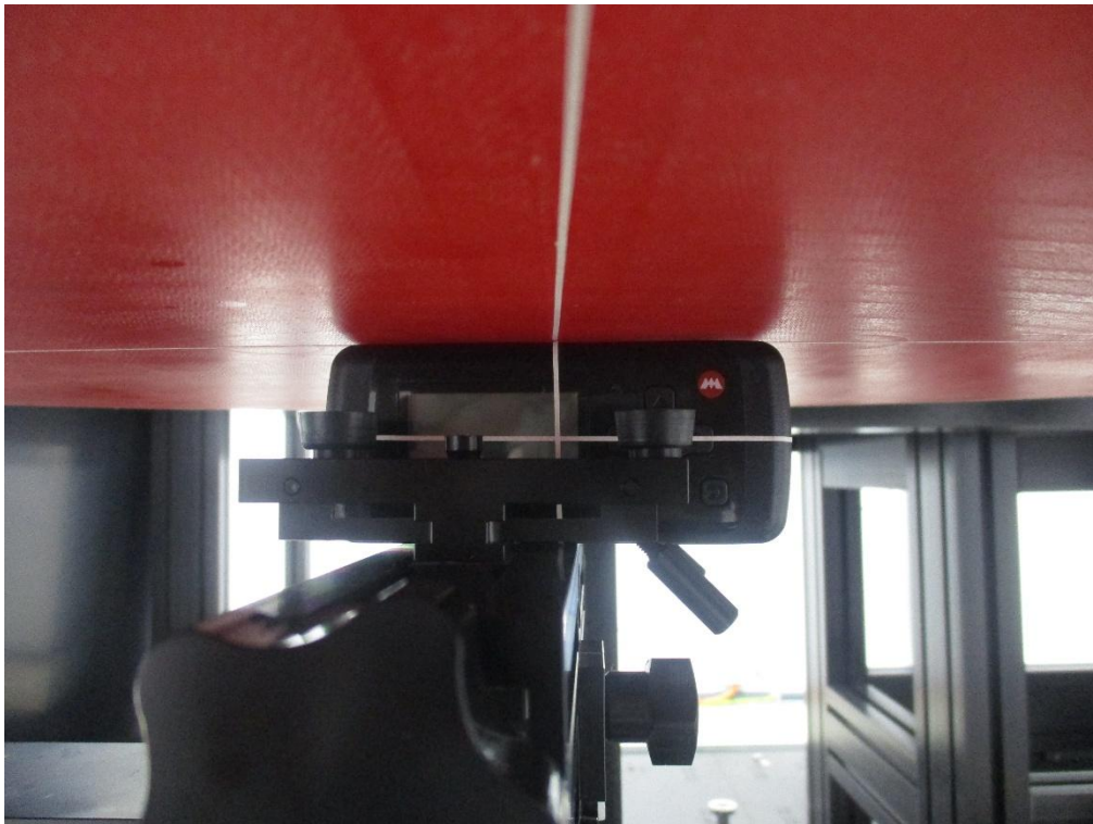
Top Side from Flat Phantom (Separation Distance: 0 cm) – Body SAR
