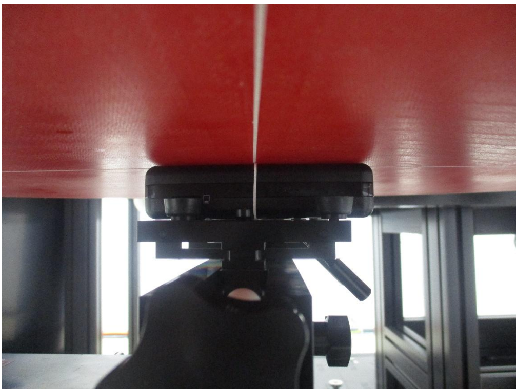
Rear Side from Flat Phantom (Separation Distance: 0 cm) – Body SAR
