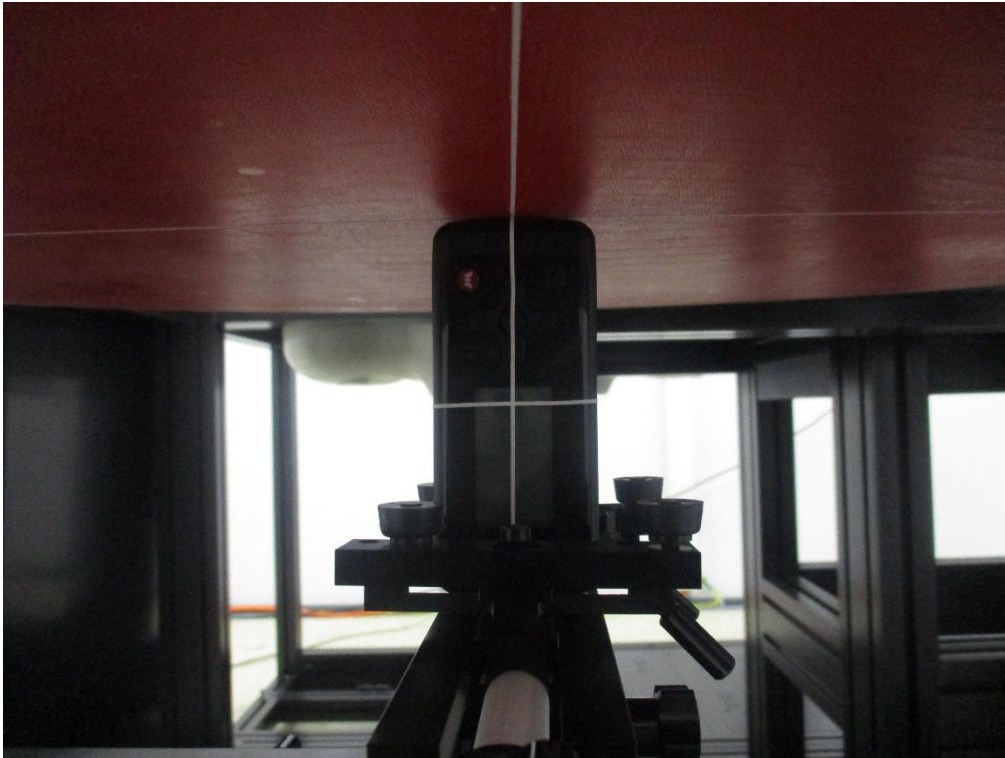
Right Side from Flat Phantom (Separation Distance: 0 cm) – Body SAR
