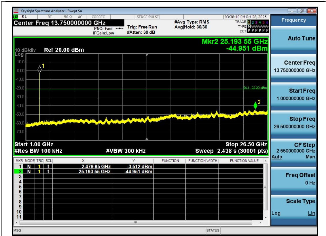
BLE_1M-Ant1-2480-1000~26500-PASS
