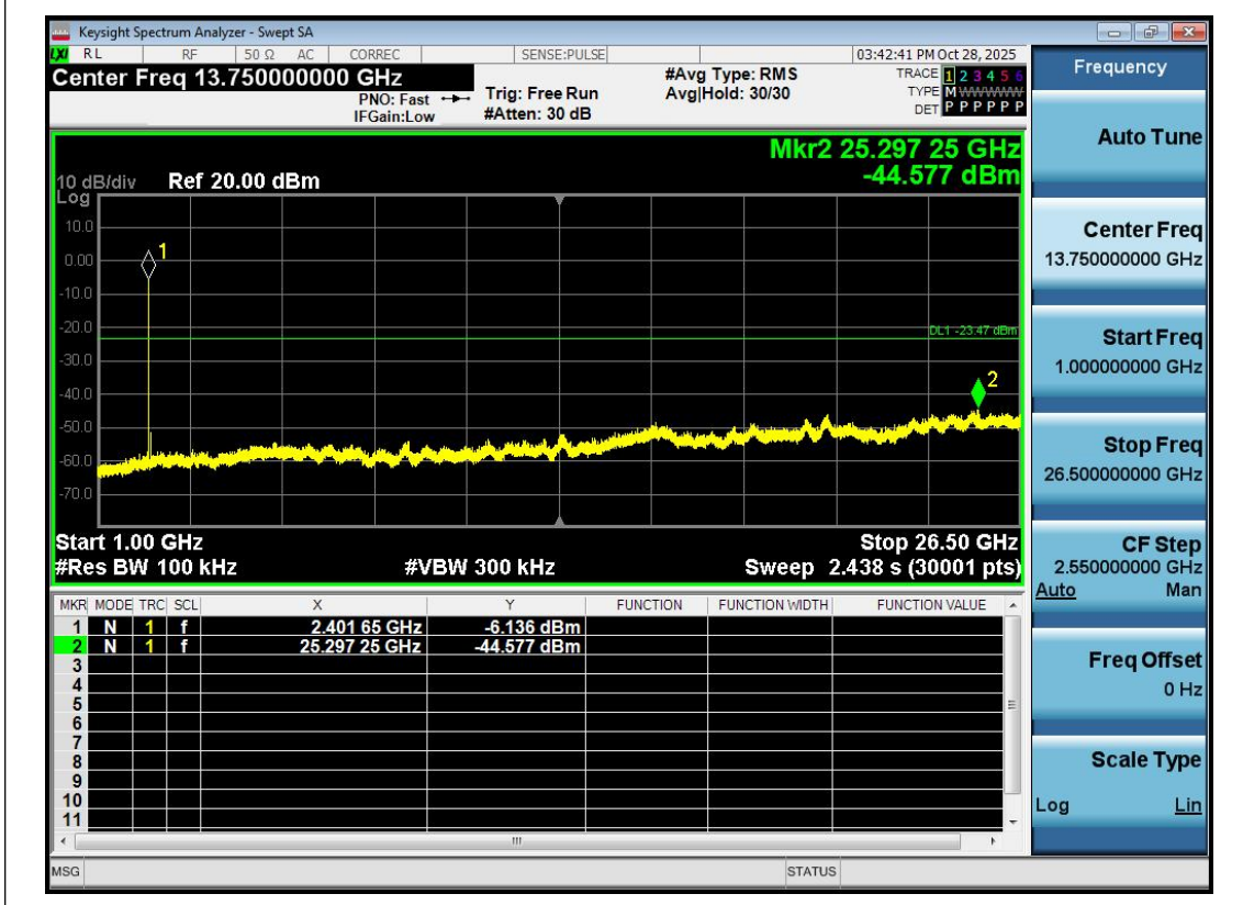
BLE_2M-Ant1-2402-1000~26500-PASS
