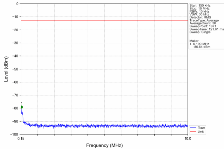
Band2 3MHz 16QAM HCH 1908.5MHz RB 1 0 NTV
