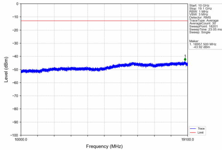
Band2 3MHz 16QAM HCH 1908.5MHz RB 1 0 NTN
