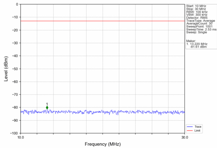
Band2 3MHz 16QAM HCH 1908.5MHz RB 1 0 NTV
