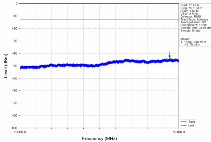
Band2 15MHz 16QAM MCH 1880MHz RB 1 0 NTNV
