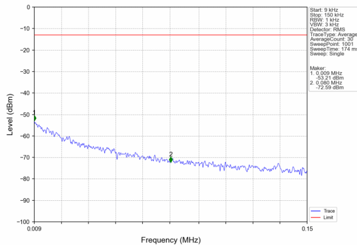
Band2 15MHz 16QAM MCH 1880MHz RB 1 0 NTNV
