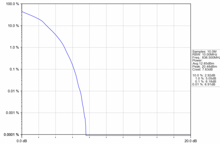
Band5 10MHz 16QAM MCH 836.5MHz RB 27 0 NTNV
