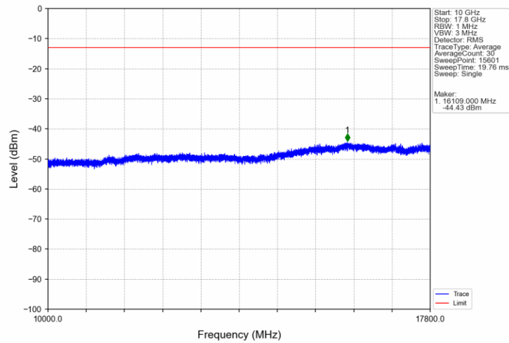
Band66 1.4MHz 16QAM HCH 1779.3MHz RB 1 0 NTNV
