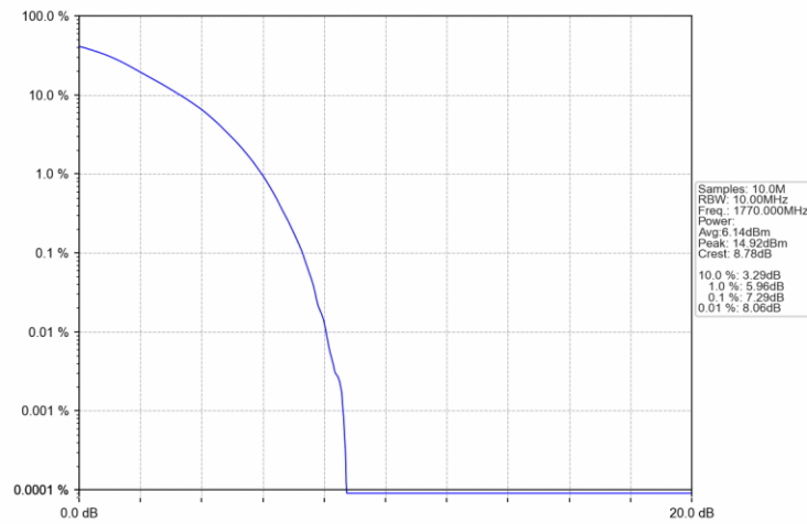
Band66 20MHz 16QAM HCH 1770MHz RB 27 73 NTN
