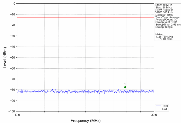
Band66 1.4MHz 16QAM HCH 1779.3MHz RB 1 0 NTNV
