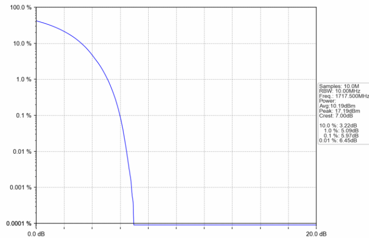
Band66 15MHz 16QAM LCH 1717.5MHz RB 27 0 NTNV
