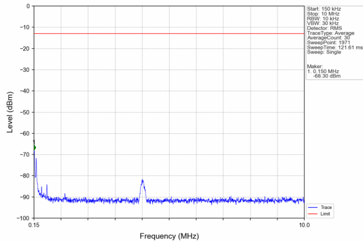
Band66 3MHz QPSK LCH 1711.5MHz RB 1 0 NTNV
