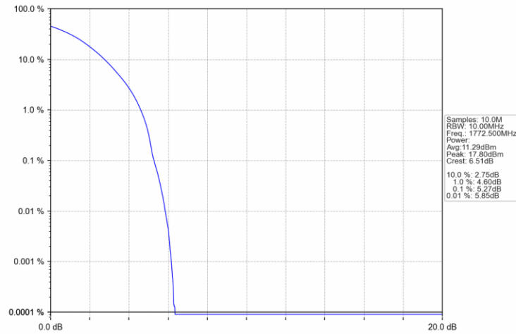
Band66 15MHz QPSK HCH 1772.5MHz RB 75 0 NTNV
