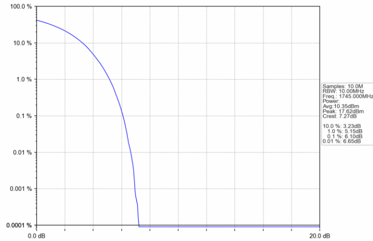
Band66 15MHz 16QAM MCH 1745MHz RB 27 0 NTNV
