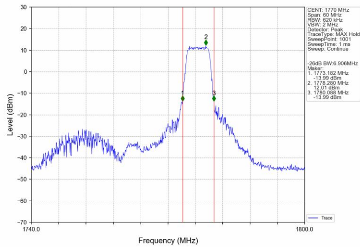
Band66 20MHz 16QAM HCH 1770MHz RB 27 73 NTNV
