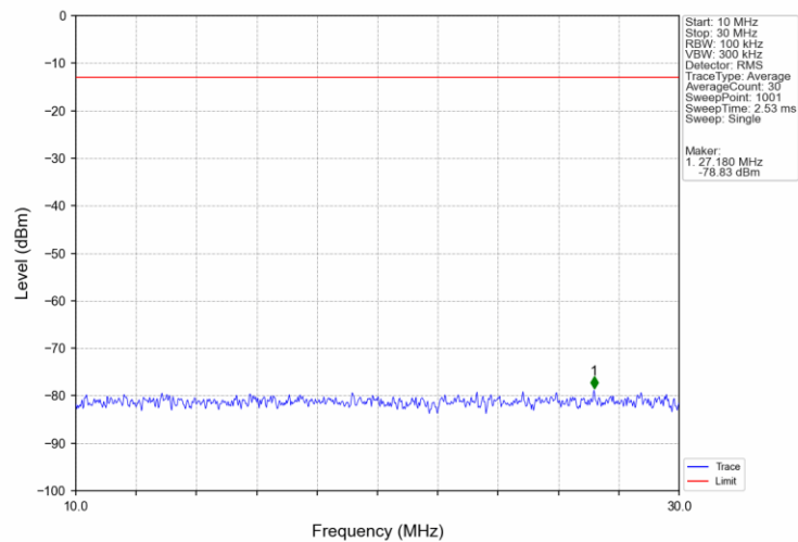
Band66 3MHz QPSK LCH 1711.5MHz RB 1 0 NTNV
