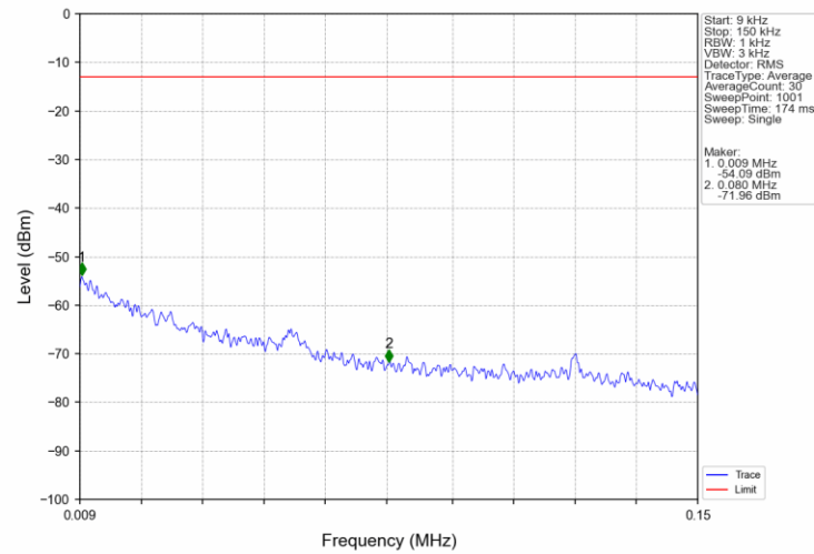
Band66 1.4MHz QPSK HCH 1779.3MHz RB 1 0 NTNV
