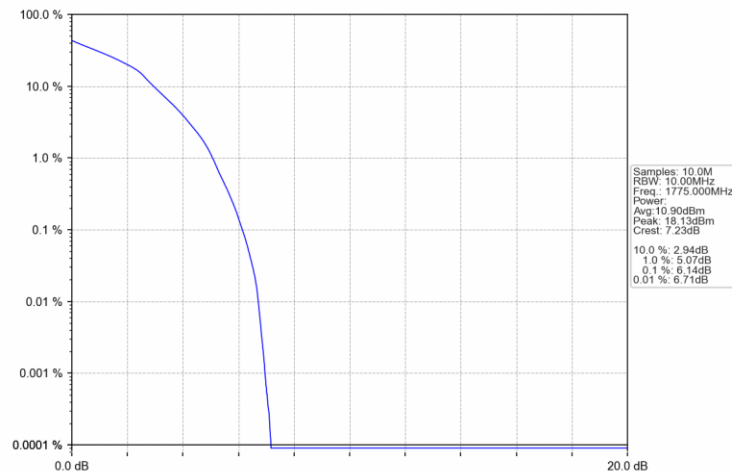
Band66 10MHz 16QAM HCH 1775MHz RB 27 23 NTN
