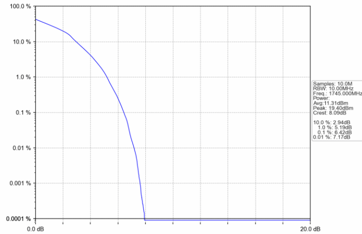
Band66 10MHz 16QAM MCH 1745MHz RB 27 0 NTN
