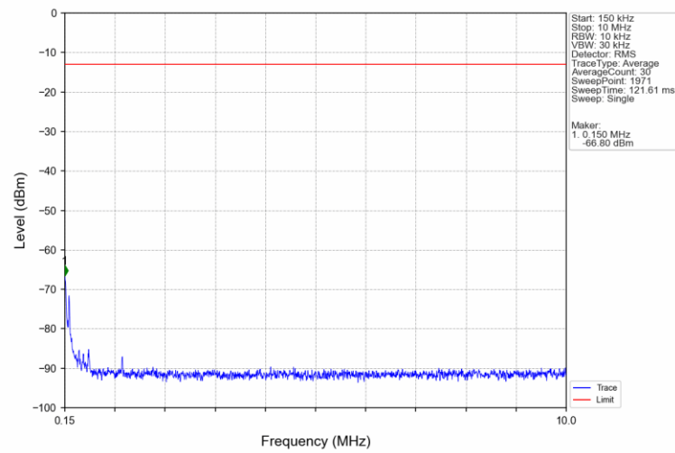
Band66 1.4MHz QPSK HCH 1779.3MHz RB 1 0 NTNV
