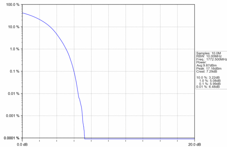
Band66 15MHz 16QAM HCH 1772.5MHz RB 27 48 NTNV
