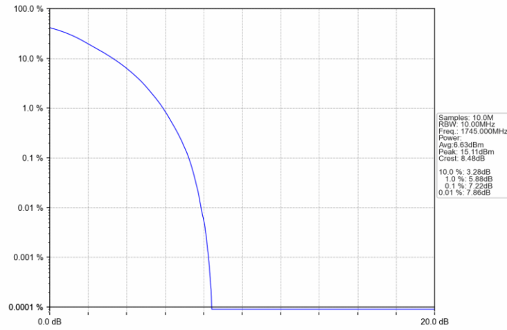
Band66 20MHz 16QAM MCH 1745MHz RB 27 0 NTN
