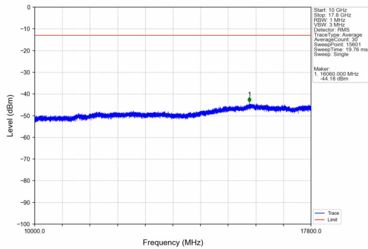
Band66 15MHz QPSK MCH 1745MHz RB 1 0 NTNV
