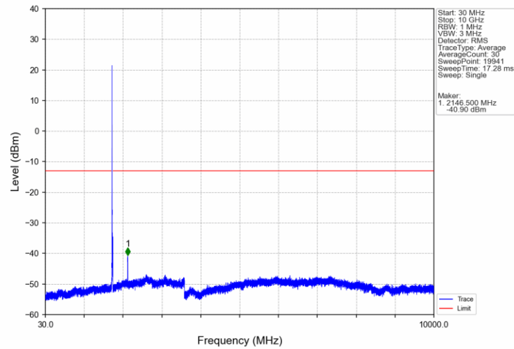
Band66 10MHz 16QAM MCH 1745MHz RB 1 0 NTNV
