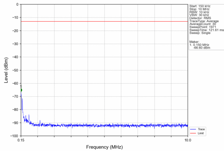
Band66_10MHz_16QAM_HCH_1775MHz_RB_1_0_NTNV
