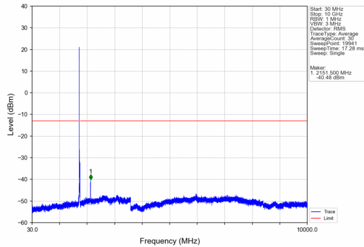
Band66 15MHz QPSK MCH 1745MHz RB 1 0 NTNV
