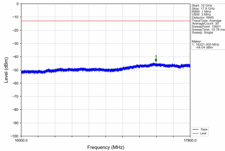
Band66 15MHz 16QAM MCH 1745MHz RB 1 0 NTN
