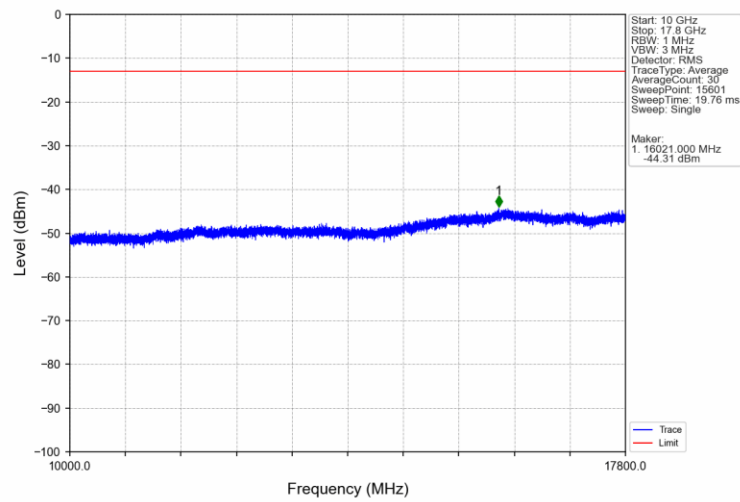
Band66 10MHz 16QAM MCH 1745MHz RB 1 0 NTNV
