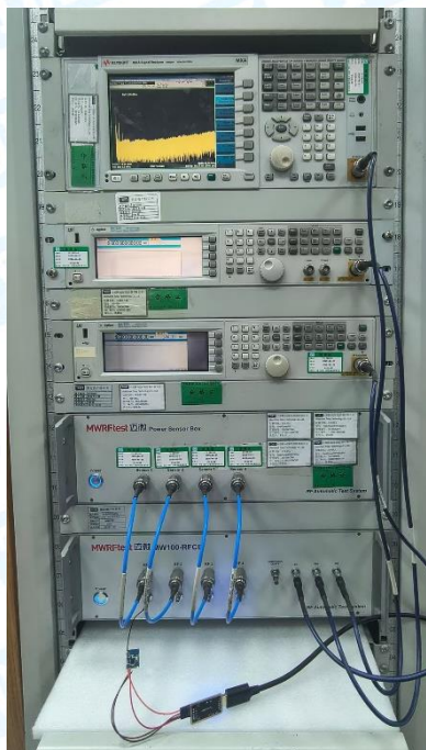
Photo of Setup for Conducted Measurements
