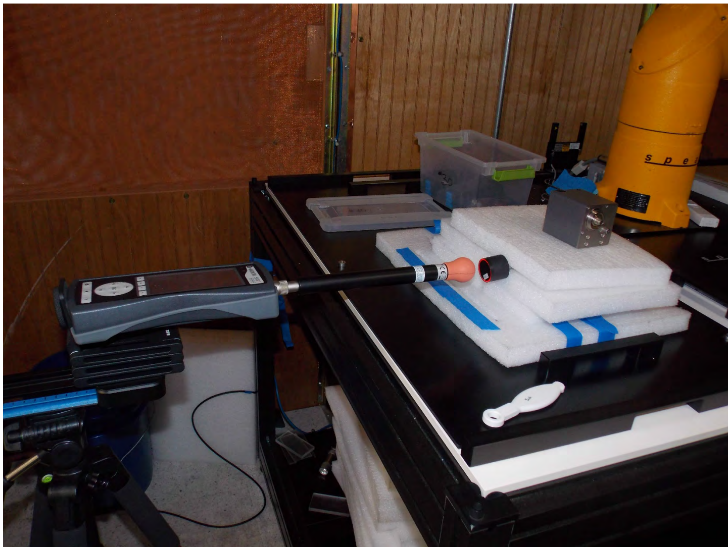
Test Position Front 125 kHz Measurements
