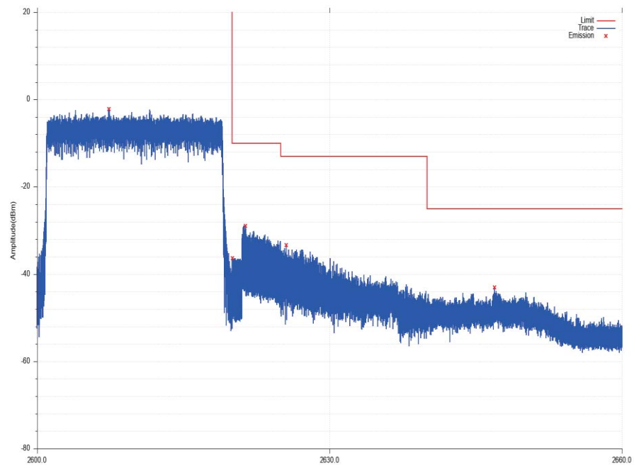
UP_EDGE_65_NT_NV_0_Band_38_QPSK_20M_CH38150_1_99
