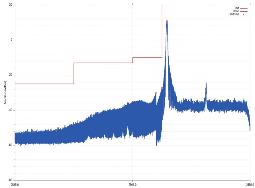
LOW_EDGE_65_NT_NV_0_Band_38_QPSK_15M_CH37825_75_0
