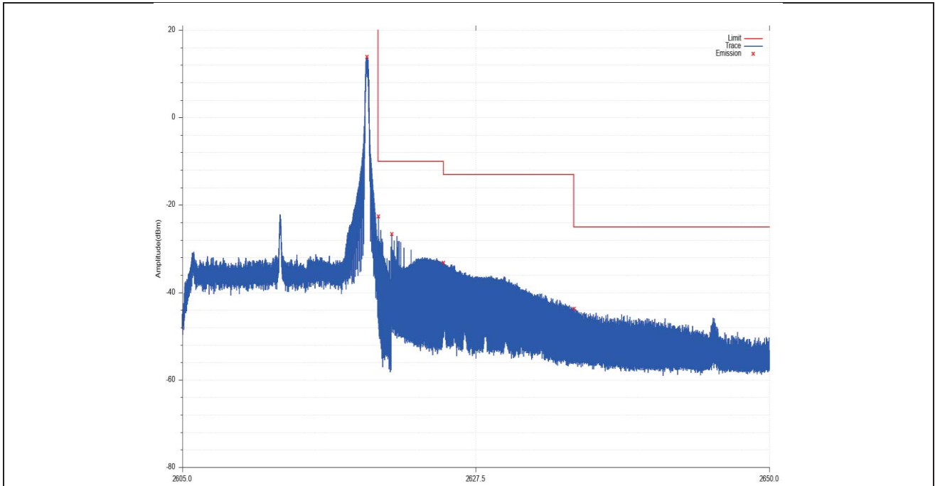
UP_EDGE_65_NT_NV_0_Band_38_16QAM_15M_CH38175_75_0
