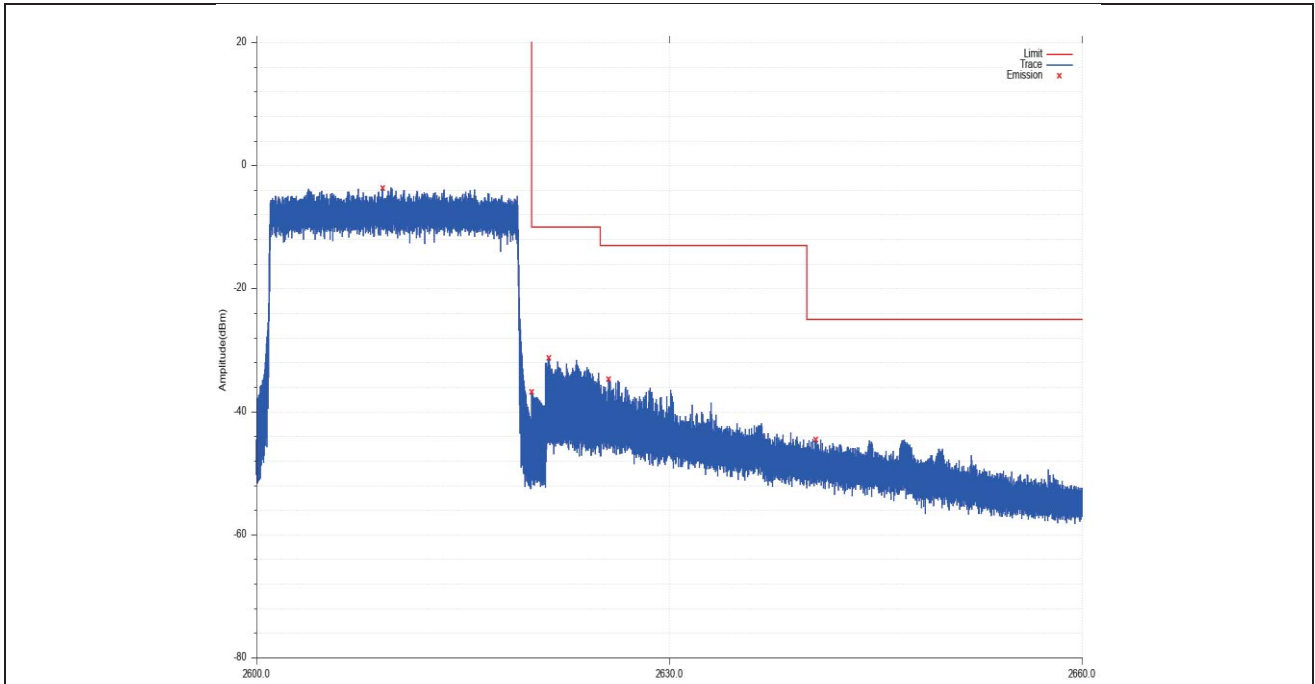
UP_EDGE_65_NT_NV_0_Band_38_16QAM_20M_CH38150_1_99
