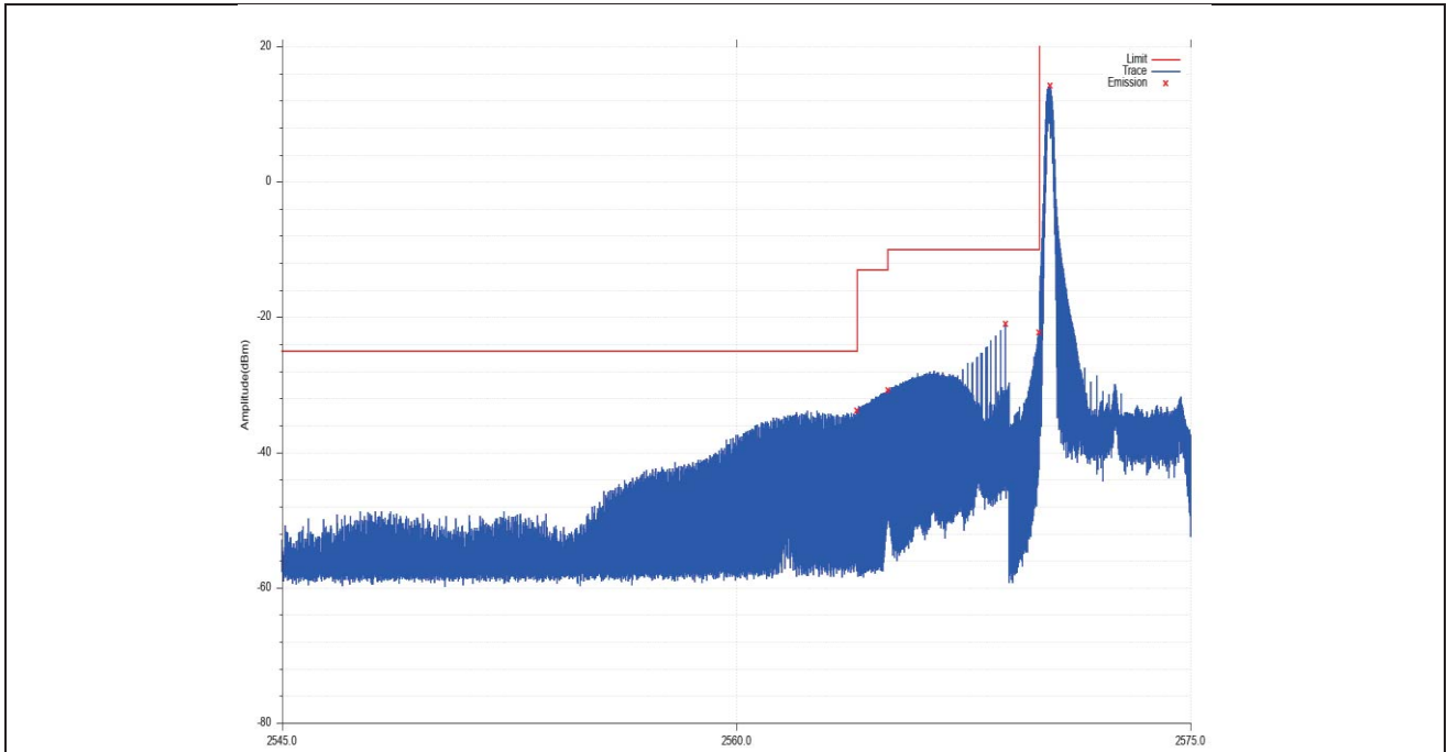
LOW_EDGE_65_NT_NV_0_Band_38_16QAM_5M_CH37775_25_0
