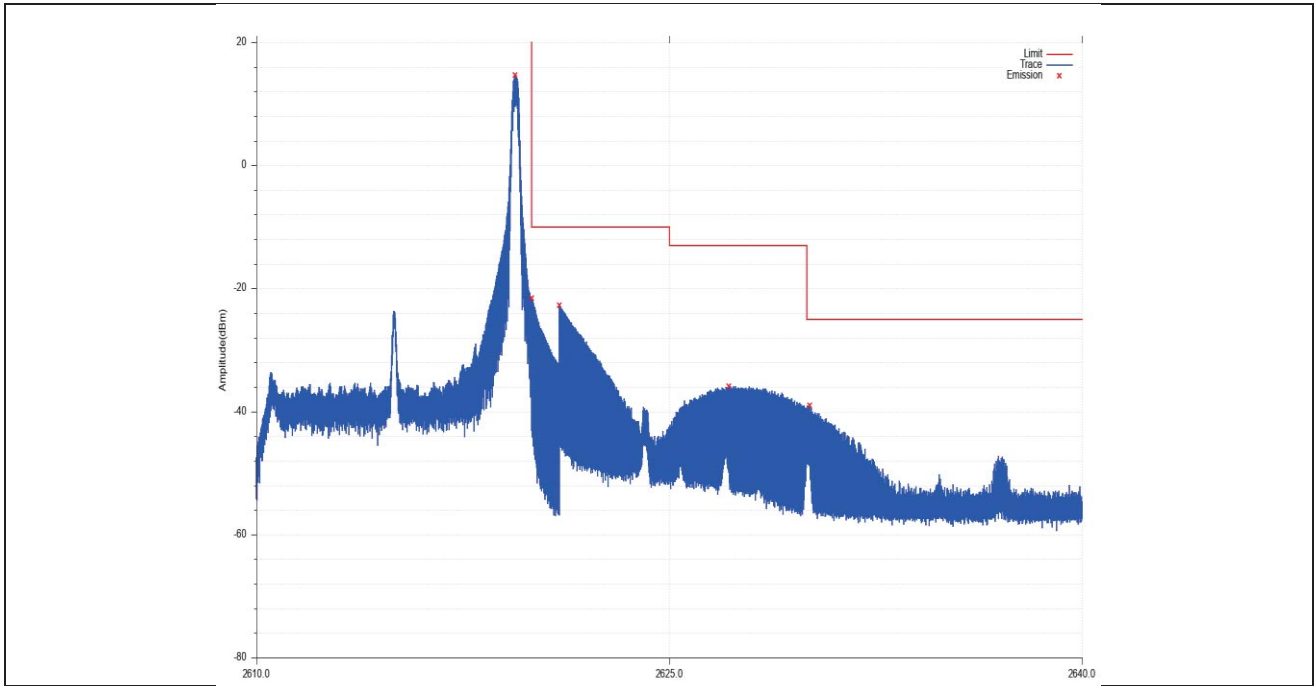
UP_EDGE_65_NT_NV_0_Band_38_16QAM_10M_CH38200_50_0
