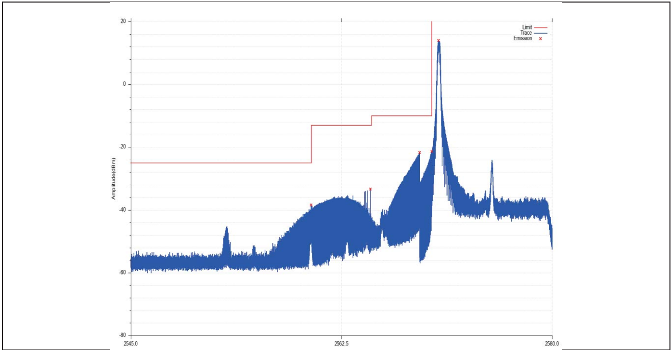
LOW_EDGE_65_NT_NV_0_Band_38_16QAM_10M_CH37800_50_0
