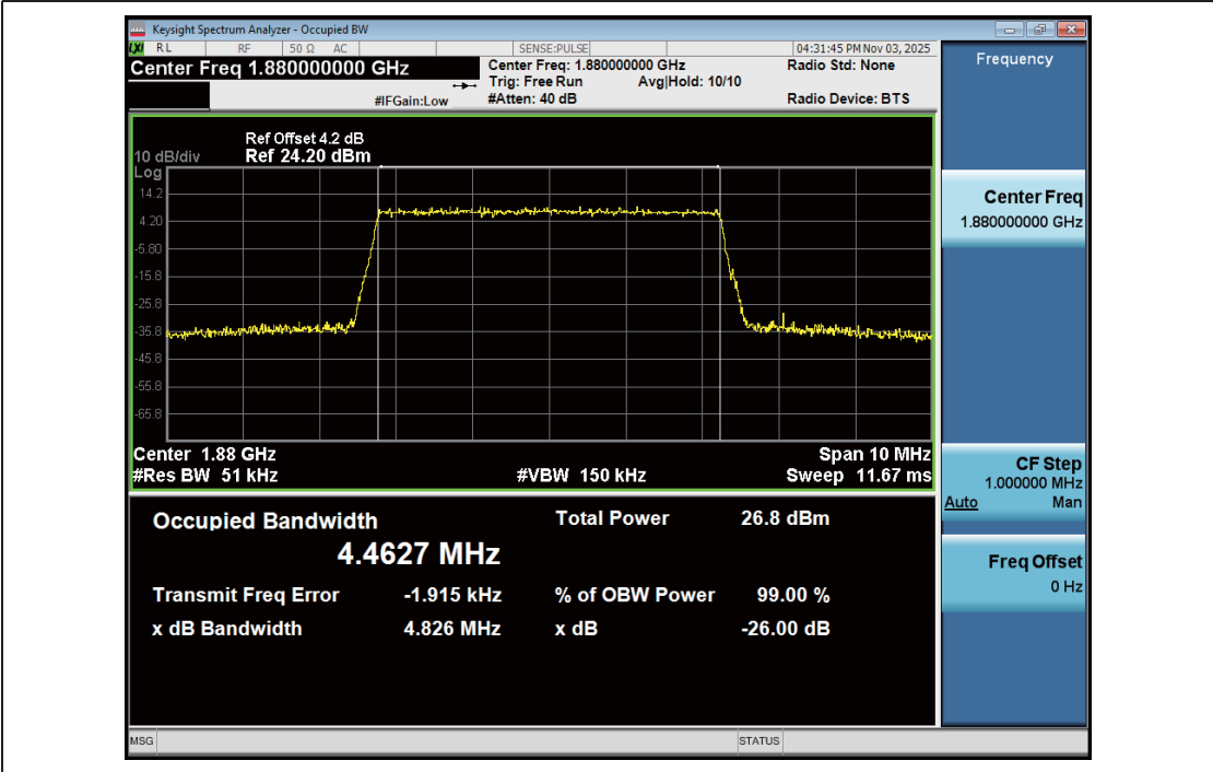
SA_65_NT_NV_0_Band_2_16QAM_5M_CH18900_25_0
