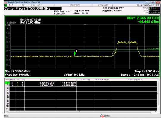
Out Of Band Emission IEEE 802.11ax Channel 1 20MHz Antenna 0 Full RU
