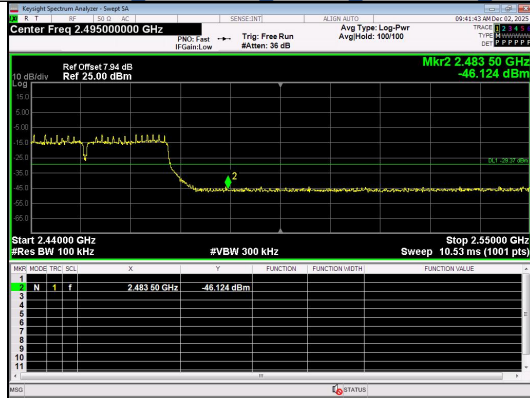
Out Of Band Emission IEEE 802.11ax Channel 9 40MHz Antenna 0 Full RU
