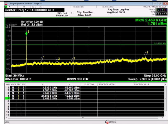
30.0 MHz - 25000.0 MHz IEEE 802.11ax Channel 11 20MHz Antenna 0 Full RU
