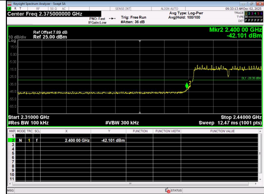
Out Of Band Emission IEEE 802.11ax Channel 3 40MHz Antenna 0 Full RU
