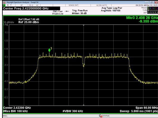
In-Band Reference Level IEEE 802.11ax Channel 3 40MHz Antenna 0 Full RU
