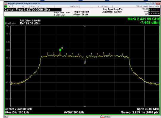
In-Band Reference Level IEEE 802.11ax Channel 6 20MHz Antenna 0 Full RU
