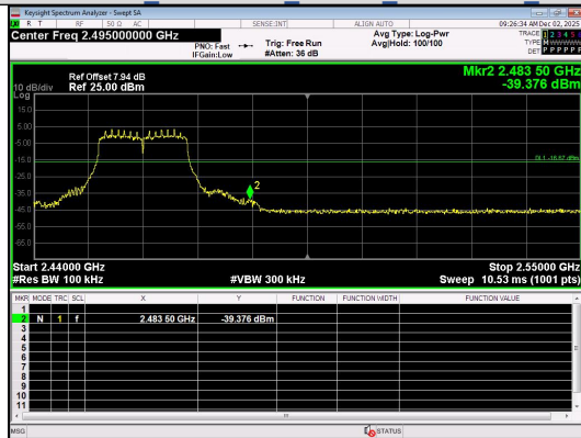
Out Of Band Emission IEEE 802.11ax Channel 11 20MHz Antenna 0 Full RU
