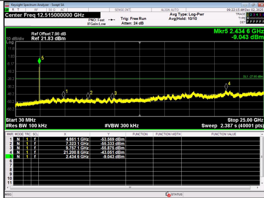
30.0 MHz - 25000.0 MHz IEEE 802.11ax Channel 6 20MHz Antenna 0 Full RU
