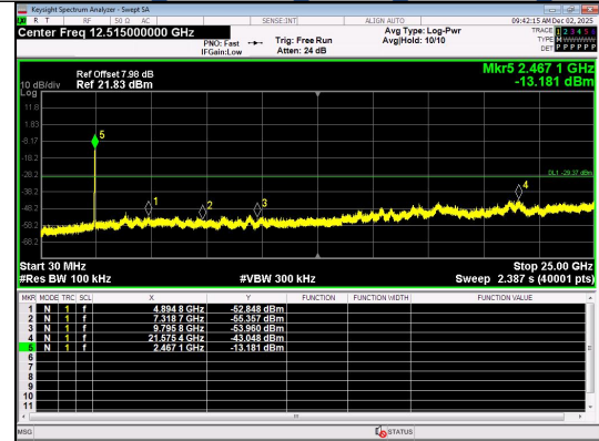
30.0 MHz - 25000.0 MHz IEEE 802.11ax Channel 9 40MHz Antenna 0 Full RU
