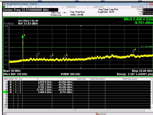
30.0 MHz - 25000.0 MHz IEEE 802.11ax Channel 3 40MHz Antenna 0 Full RU
