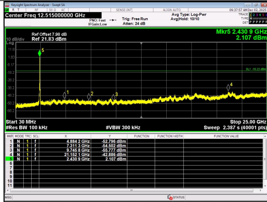
30.0 MHz - 25000.0 MHz IEEE 802.11ax Channel 6 40MHz Antenna 0 Full RU
