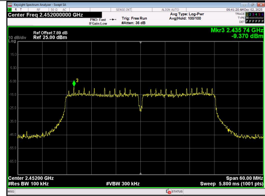
In-Band Reference Level IEEE 802.11ax Channel 9 40MHz Antenna 0 Full RU
