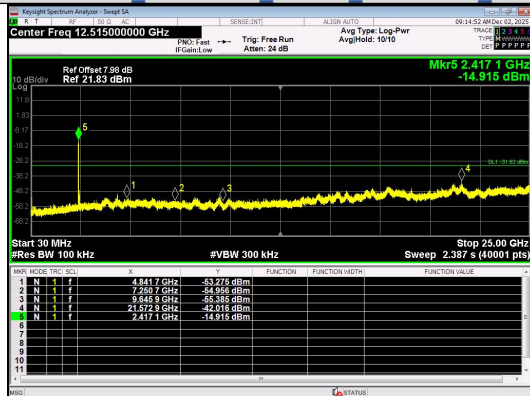
30.0 MHz - 25000.0 MHz IEEE 802.11ax Channel 1 20MHz Antenna 0 Full RU
