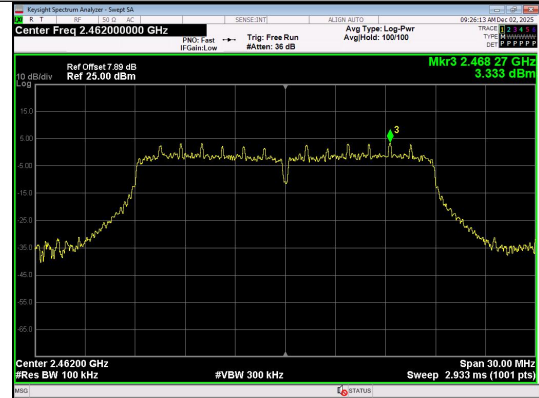
In-Band Reference Level IEEE 802.11ax Channel 11 20MHz Antenna 0 Full RU
