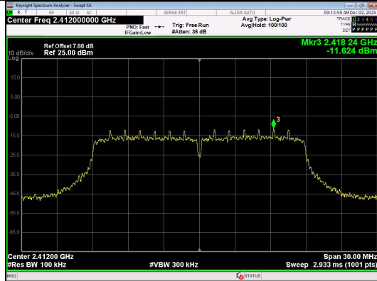
In-Band Reference Level IEEE 802.11ax Channel 1 20MHz Antenna 0 Full RU
