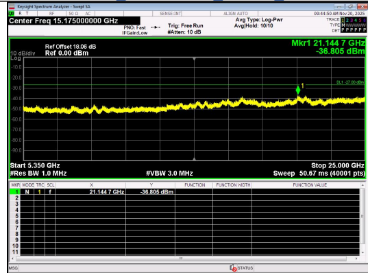
Spurious Emission:5350~25000.0 MHz IEEE 802.11n Channel 36_20MHz_Antenna 0
