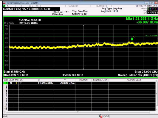
Out Of Band Emission IEEE 802.11ax Channel 36 20MHz Antenna 0 Full RU
