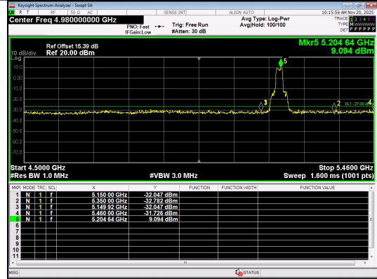
Out Of Band Emission IEEE 802.11ac_Channel 40_20MHz_Antenna 0
