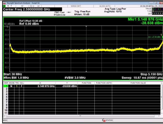
Spurious Emission:30.0~5150 MHz IEEE 802.11ac Channel 42 80MHz Antenna 0
