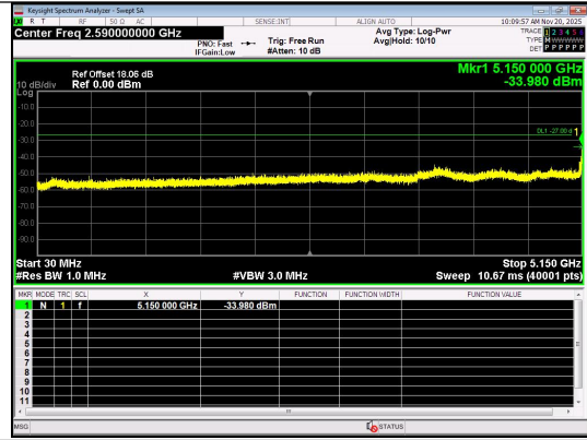
Spurious Emission:30.0~5150 MHz IEEE 802.11ac_Channel 36_20MHz_Antenna 0
