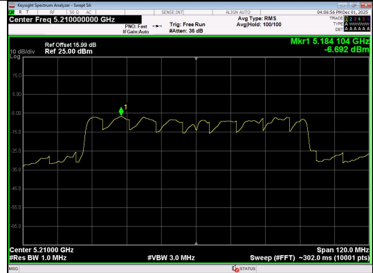
IEEE 802.11ax Channel 42 80MHz Antenna 0 Full RU
