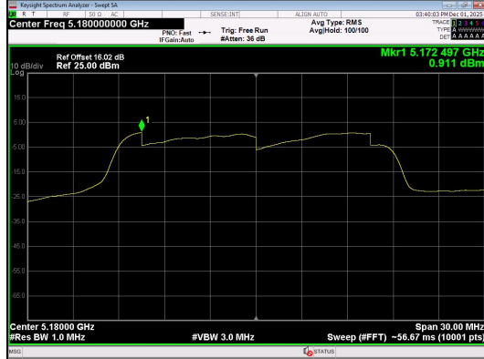
IEEE 802.11ax Channel 36 20MHz Antenna 0 Full RU
