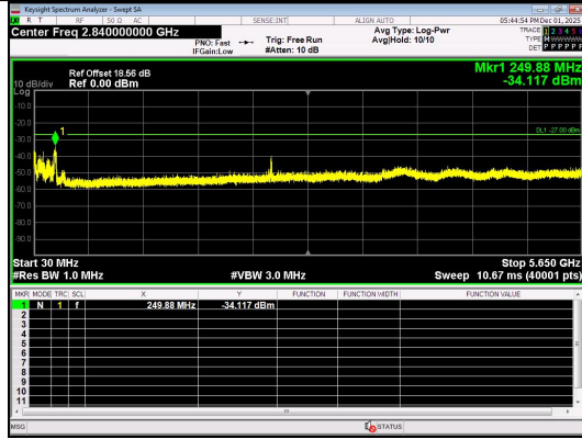
Spurious Emission:30.0~5650 MHz IEEE 802.11ax Channel 151 40MHz Antenna 0 Full RU
