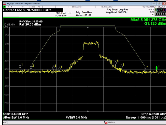
Out Of Band Emission IEEE 802.11ax Channel 159 40MHz Antenna 0 Full RU
