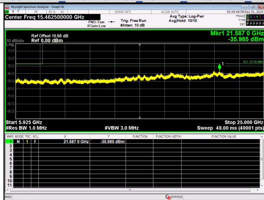
Spurious Emission:5925~25000.0 MHz IEEE 802.11ax Channel 159 40MHz Antenna 0 Full RU
