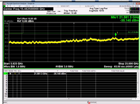
Spurious Emission:5925~25000.0 MHz IEEE 802.11ax Channel 157 20MHz Antenna 0 Full RU
