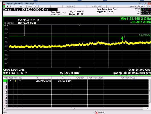
Spurious Emission:5925~25000.0 MHz IEEE 802.11ax Channel 165 20MHz Antenna 0 Full RU
