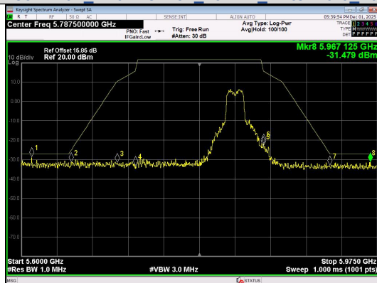
Out Of Band Emission IEEE 802.11ax Channel 165 20MHz Antenna 0 Full RU
