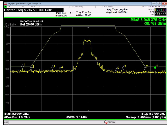
Out Of Band Emission IEEE 802.11ax Channel 157 20MHz Antenna 0 Full RU
