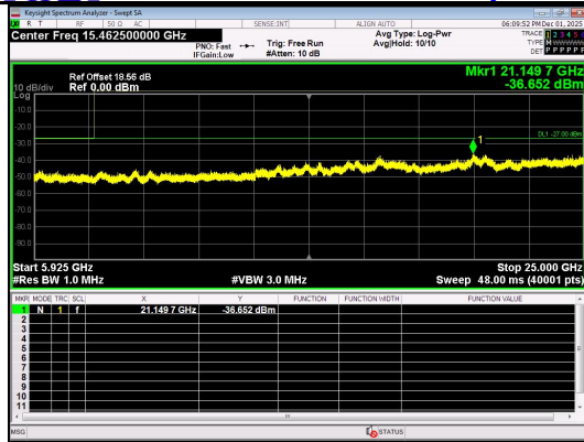
Spurious Emission:5925~25000.0 MHz IEEE 802.11ax Channel 149 20MHz Antenna 0 Full RU
