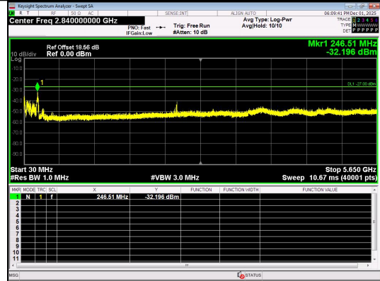
Spurious Emission:30.0~5650 MHz IEEE 802.11ax Channel 149 20MHz Antenna 0 Full RU
