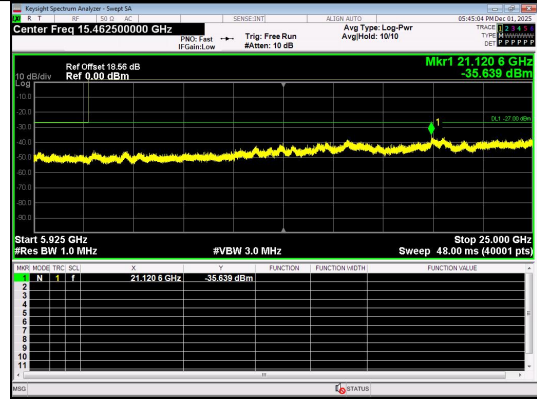
Spurious Emission:5925~25000.0 MHz IEEE 802.11ax Channel 151 40MHz Antenna 0 Full RU
