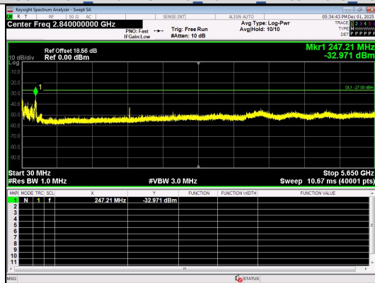
Spurious Emission:30.0~5650 MHz IEEE 802.11ax Channel 157 20MHz Antenna 0 Full RU
