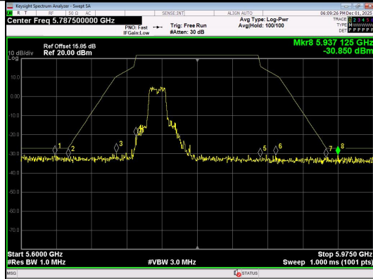
Out Of Band Emission IEEE 802.11ax Channel 149 20MHz Antenna 0 Full RU
