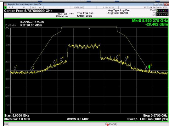
Out Of Band Emission IEEE 802.11ax Channel 155 80MHz Antenna 0 Full RU
