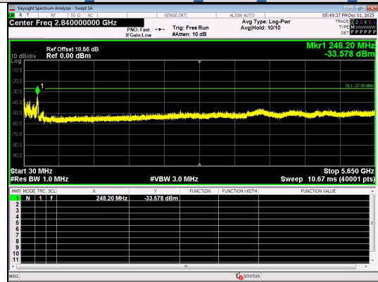
Spurious Emission:30.0~5650 MHz IEEE 802.11ax Channel 159 40MHz Antenna 0 Full RU
