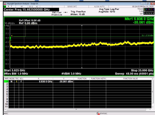
Spurious Emission:5925~25000.0 MHz IEEE 802.11ax Channel 155 80MHz Antenna 0 Full RU
