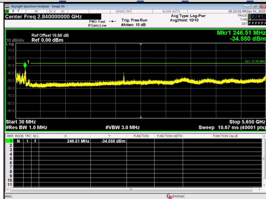
Spurious Emission:30.0~5650 MHz IEEE 802.11ax Channel 155 80MHz Antenna 0 Full RU
