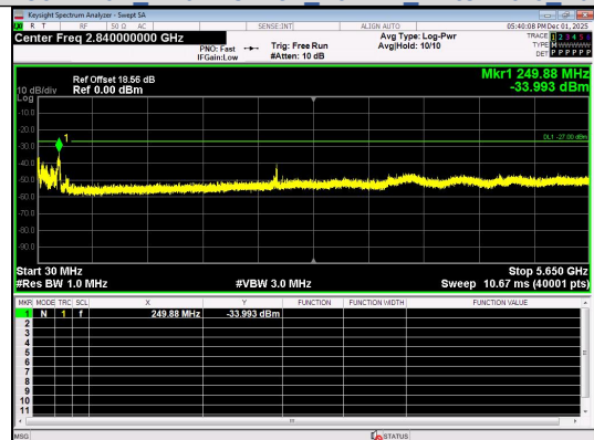
Spurious Emission:30.0~5650 MHz IEEE 802.11ax Channel 165 20MHz Antenna 0 Full RU
