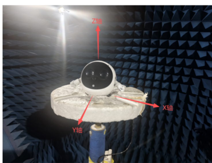
3D image of a 2400M antenna
