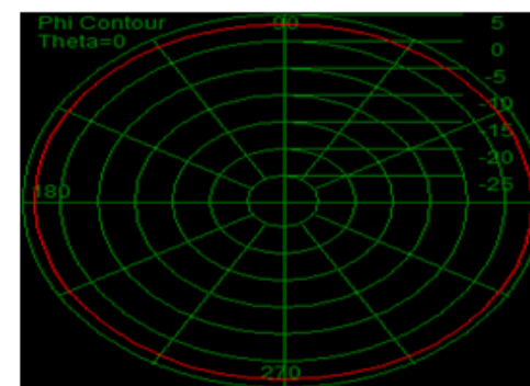
2D antenna diagram H plane
