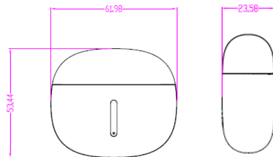
Charging box
