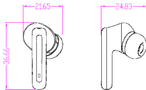
Bluetooth headset
