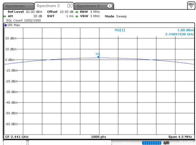
BDR_DH5_Middle
