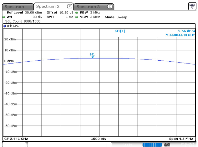
2EDR_DH3_Middle
