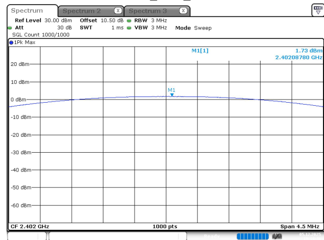
2EDR_DH3_Low
