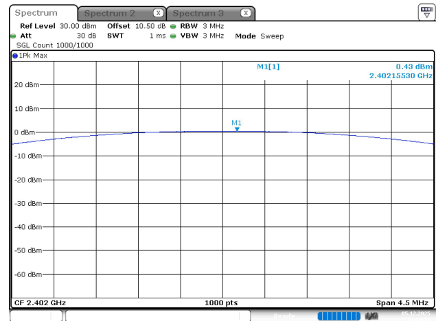
BDR_DH5_Low
