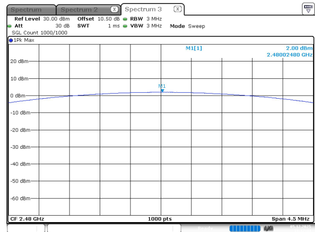
BDR_DH5_High
