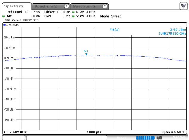
2EDR_DH5_Low
