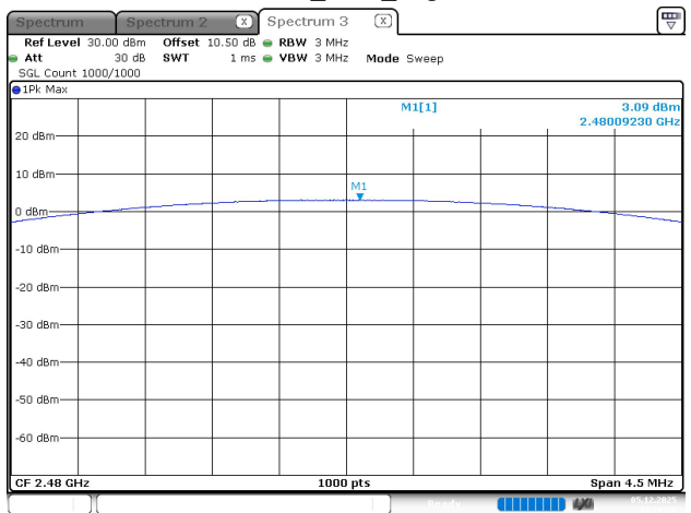
2EDR_DH5_High
