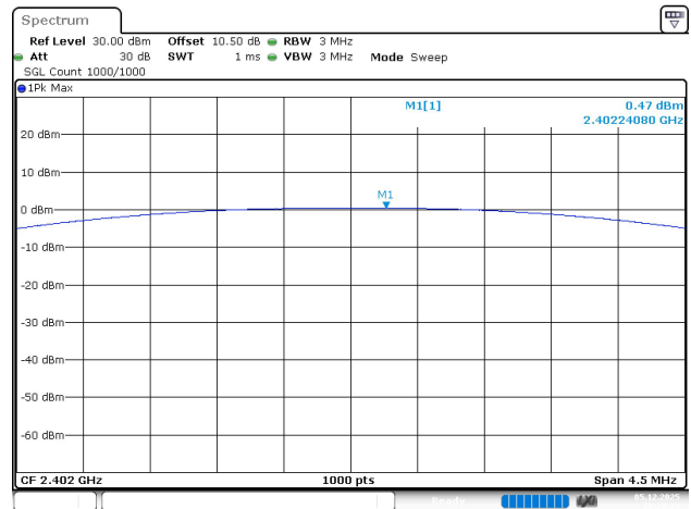
BDR_DH3_Low
