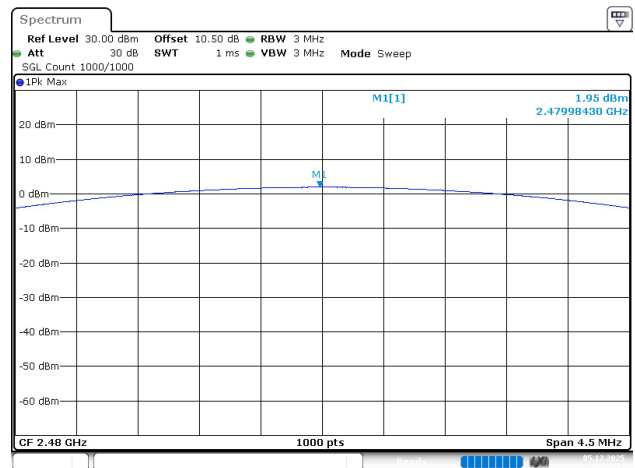
BDR_DH3_High
