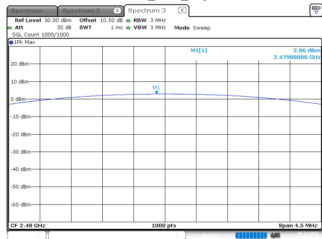
2EDR_DH3_High
