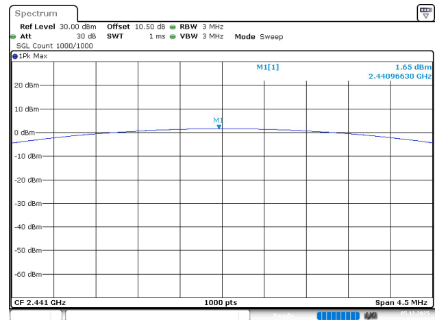
BDR_DH3_Middle
