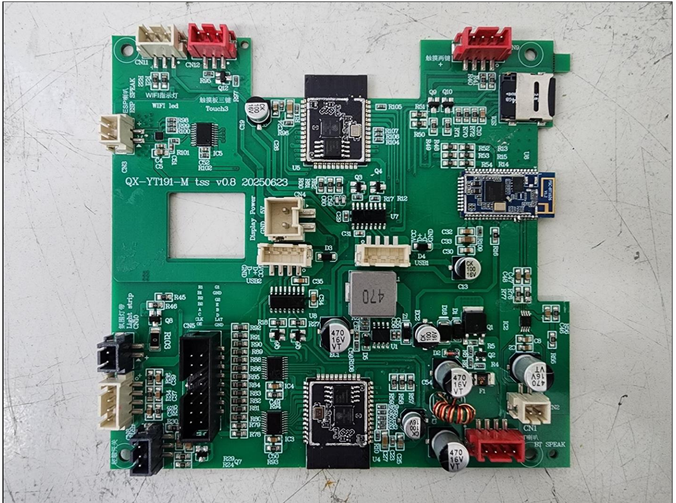
Top view of Main PCB
