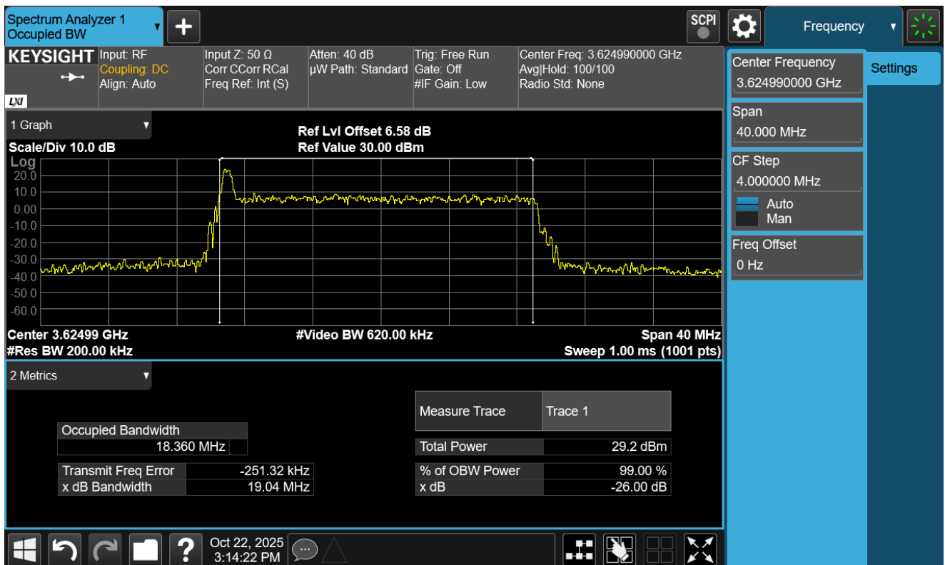
Emission Bandwidth & Occupied Bandwidth\n48\20M\n48_20M_CP_DL641666_Outer_Full RB_256QAM.png
