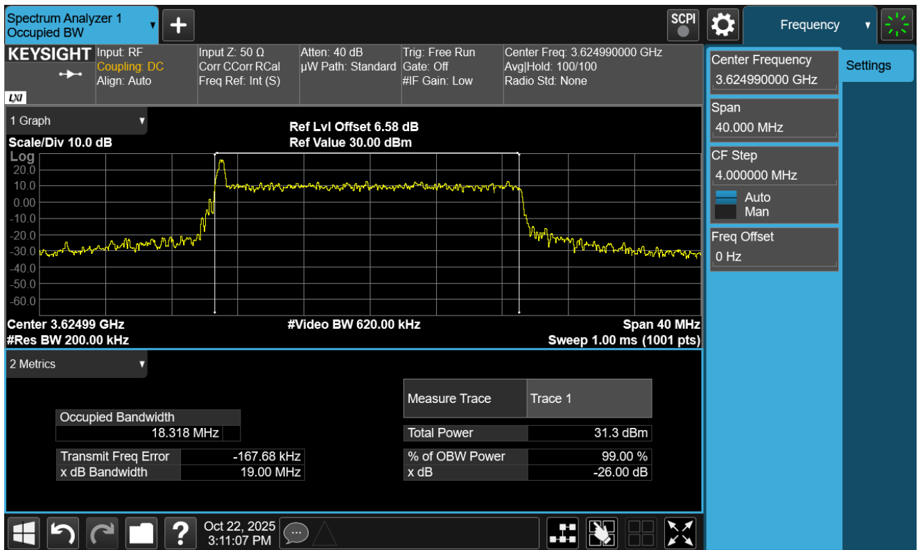
Emission Bandwidth & Occupied Bandwidth\n48\20M\n48_20M_CP_DL641666_Outer_Full RB_16QAM.png
