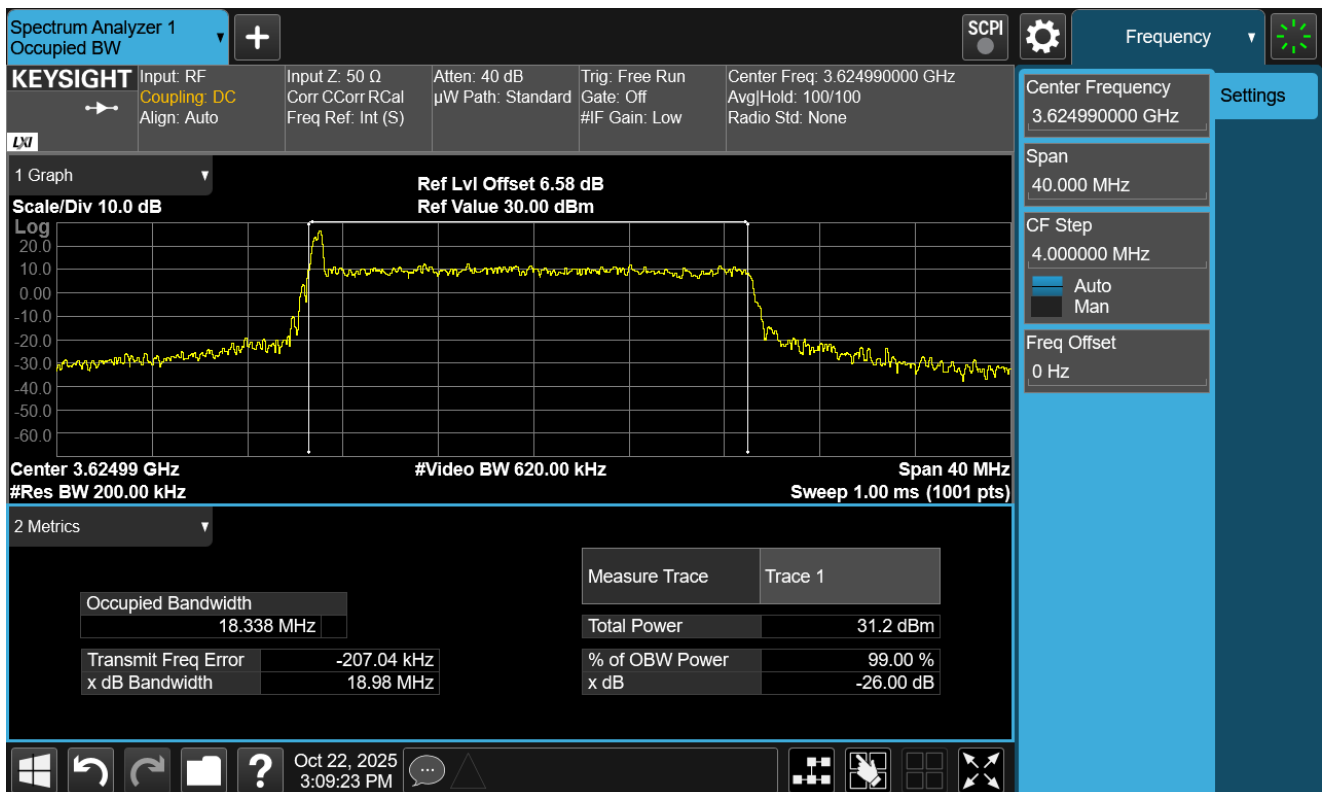
Emission Bandwidth & Occupied Bandwidth\n48\20M\n48_20M_CP_DL641666_Outer_Full RB_QPSK.png
