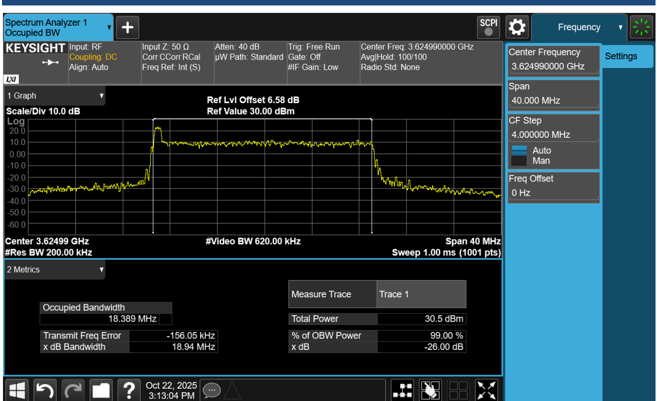
Emission Bandwidth & Occupied Bandwidth\n48\20M\n48_20M_CP_DL641666_Outer_Full RB_64QAM.png
