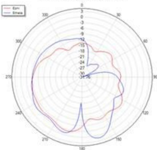
Phi=0 freq=2500MHz
