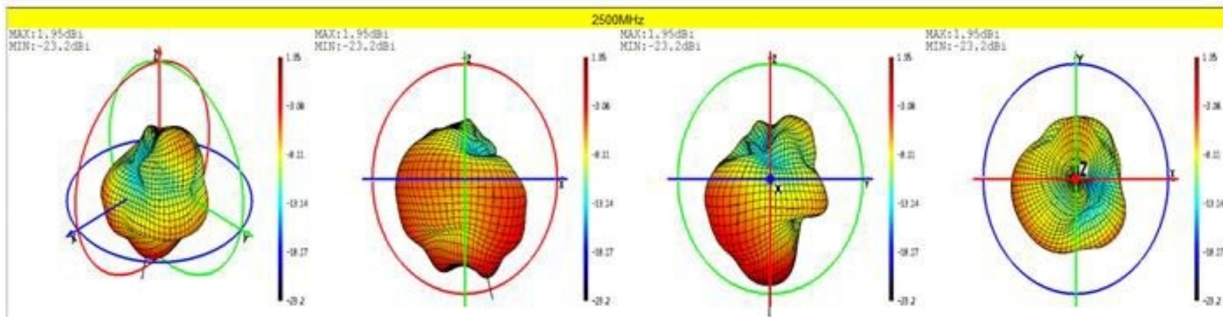
Phi=0 freq=2500MHz
