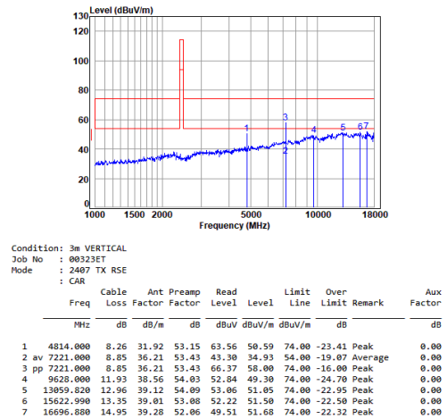
2.4G_SRD_LOW_TX_Vertical
