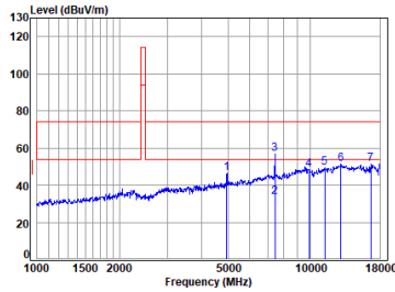
2.4G_SRD_HIGH_TX_Horizontal
