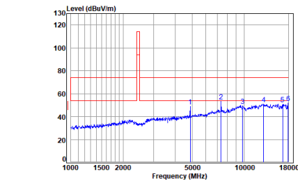
2.4G_SRD_MID_TX_Horizontal
