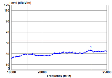
2.4G_SRD_LOW_TX_Vertical
