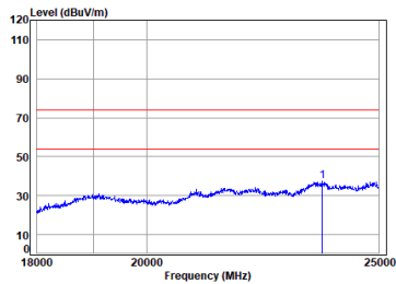
2.4G_SRD_MID_TX_Horizontal
