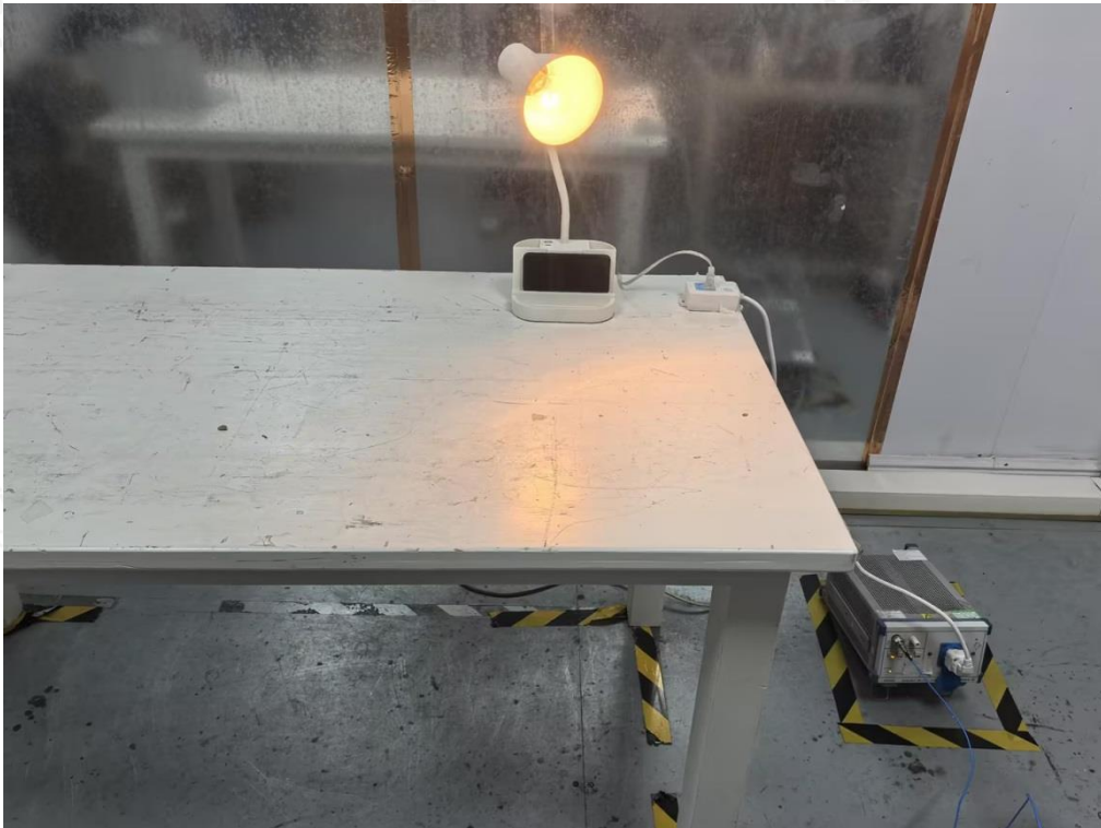
Conducted Emission-AC charge mode
